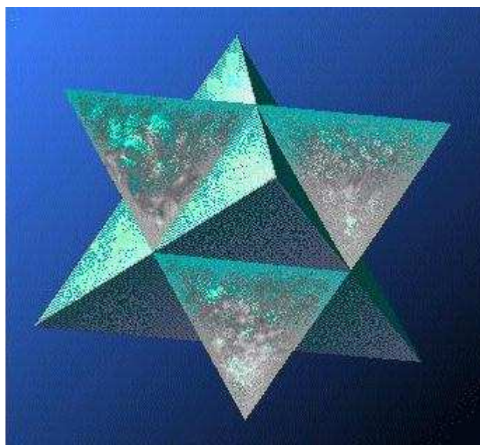
Star Tetrahedron
