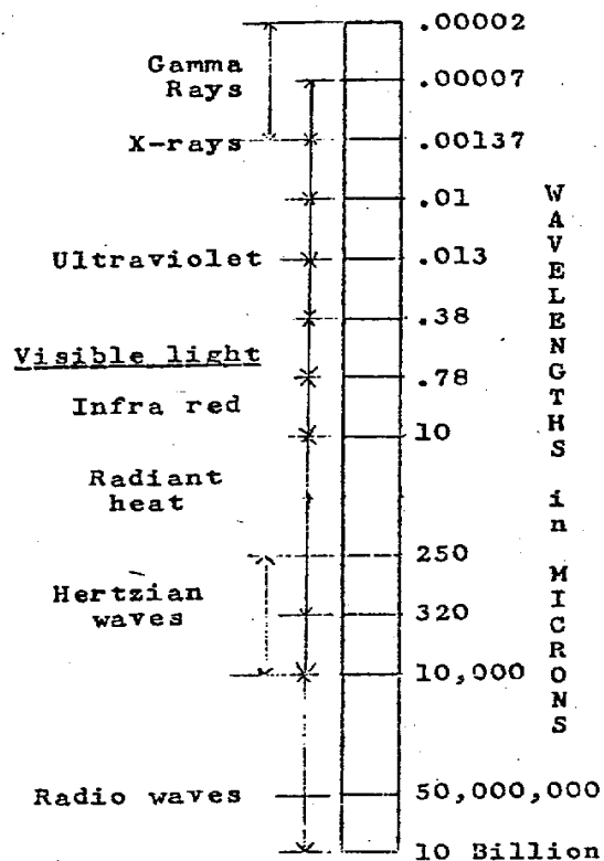
THE ELECTROMAGNETIC SPECTRUM From Williams' "The Fundamentals of Radio"
