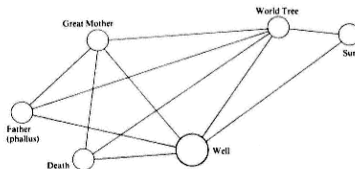
Figure 8. A field of related archetypes.
