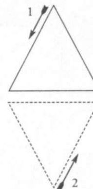
Figure 64. Western hexagram.
