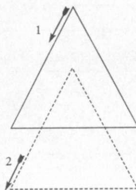
Figure 62. Eastern hexagram.
