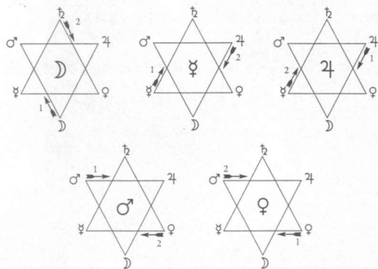
Figure 66. Planetary hexagrams.
