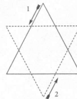
Figure 63. Southern hexagram.
