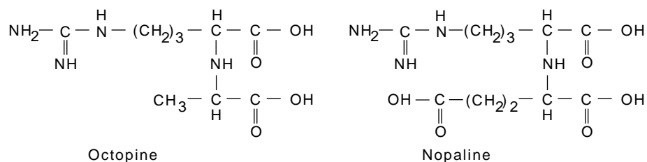
Figure 23.1 Structures of octopine and nopaline.
