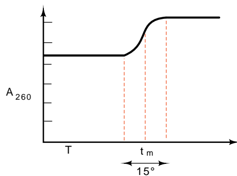
Figure 2.4 Increase in absorbance at 260\text{ nm} , A_{260} , of a DNA sample as the temperature is increased through the melting temperature.
