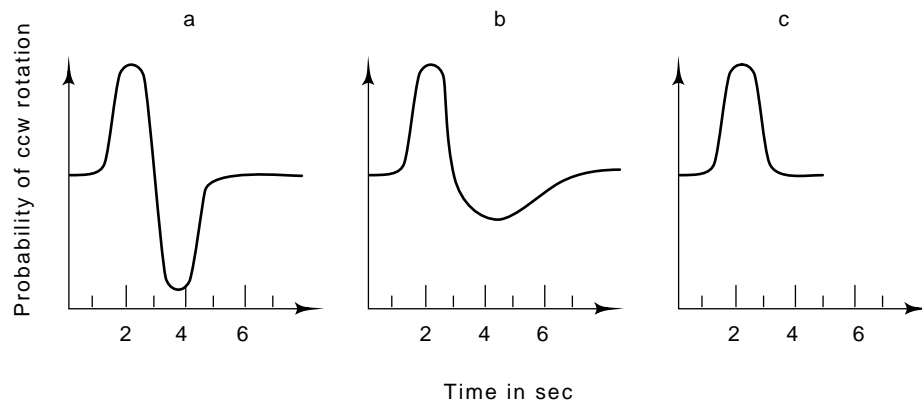
Figure 22.14 Probabilities of counterclockwise rotation following a brief exposure to attractant.
