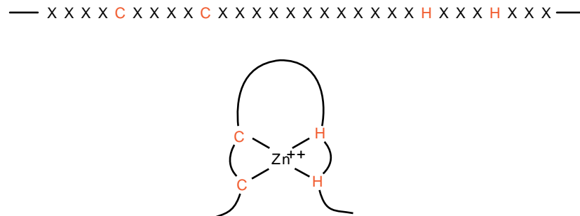
Figure 15.8 Locations of cysteines and histidines in zinc fingers.
