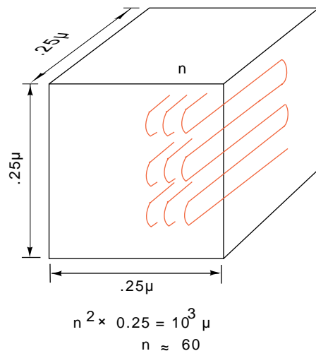
Figure 1.6 Calculation of the number of times the E. coli chromosome winds back and forth if it is confined within a cube of edge 0.25 \text{ }\mu . Each of the n layers of DNA possesses n segments of length 0.25 \text{ }\mu .
