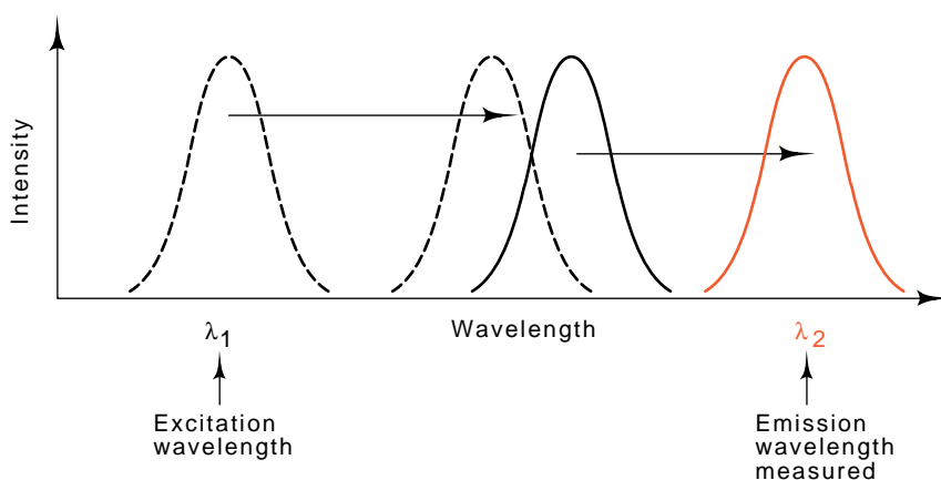
Figure 21.8 Spectra used in measuring distances separating ribosomal proteins. Dotted line is the excitation and emission spectrum of fluorescent molecule 1 and the solid line is the excitation and emission spectra for molecule 2.
