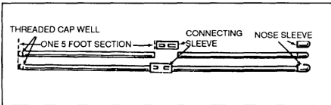
Figure 2-81. Bangalore torpedo.
