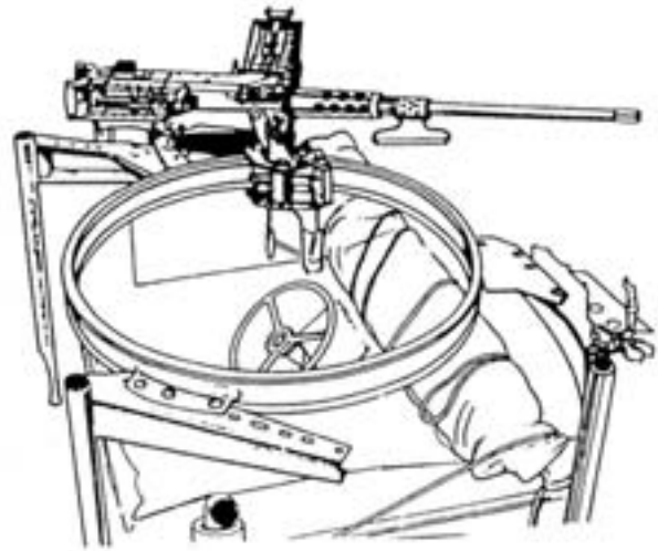
Figure 4-73. M66 Truck Ring Mount.
