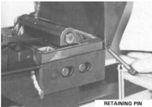
Figure 5-10. Removing the Feed Tray Cover Retaining Pin.
