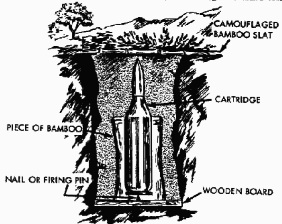
CARTRIDGE TRAP (FOOT BREAKER) 75 Spike Board Pit
