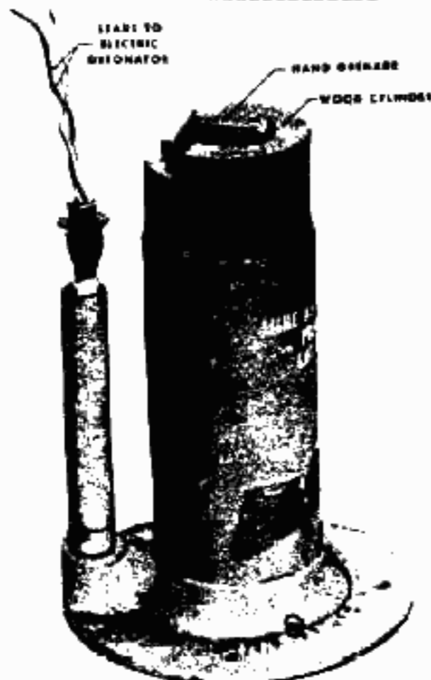
BOUNDING FRAGMENTATION MINE
