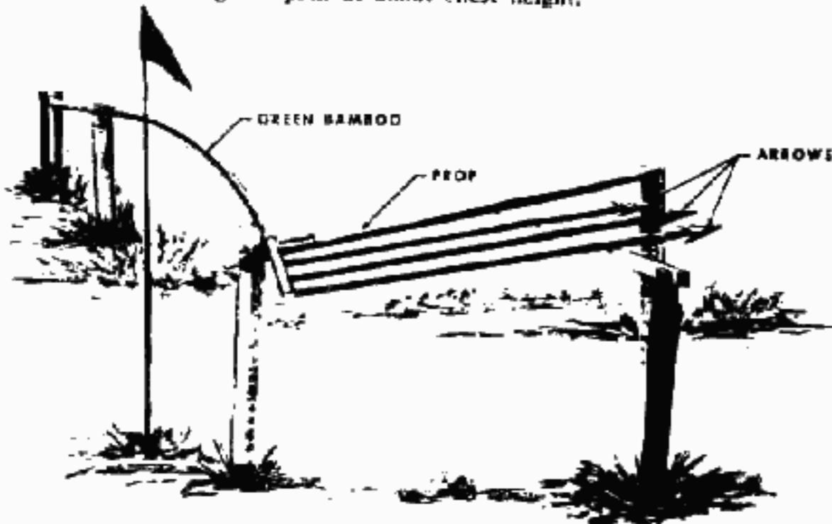
WHIP 71 Bicycle Mine
