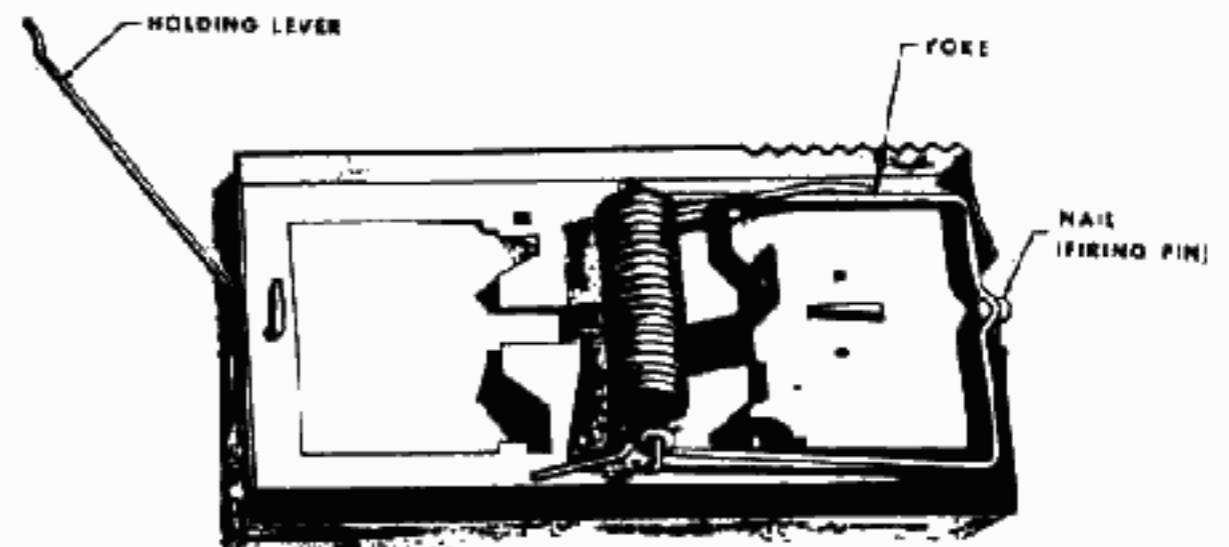
MOUSETRAP FIRING DEVICE
