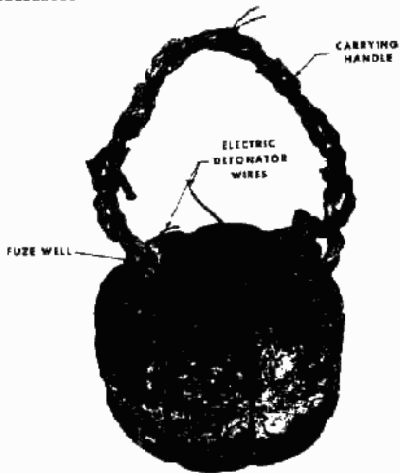
METAL BOX MINE
