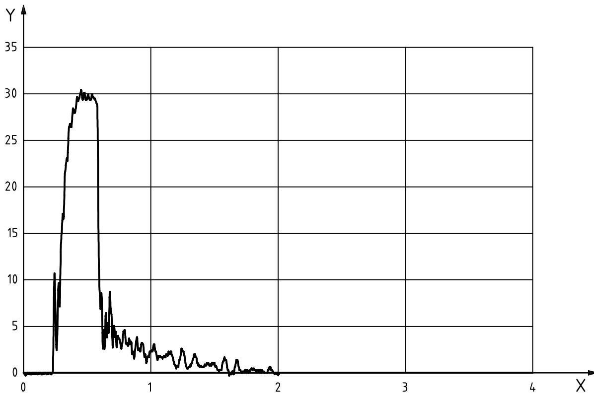
b) Test material Type T, temperature = -30 °C
