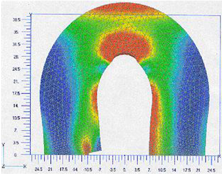
Figure 28 — Finite element analysis of chain links with eroded slit, ald = 0,22
