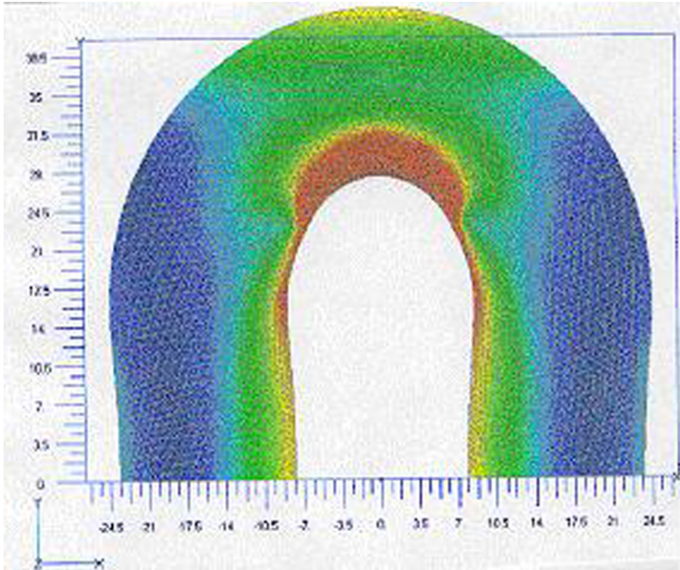
Figure 27 — Finite element analysis of chain links with eroded slit, ald = 0
