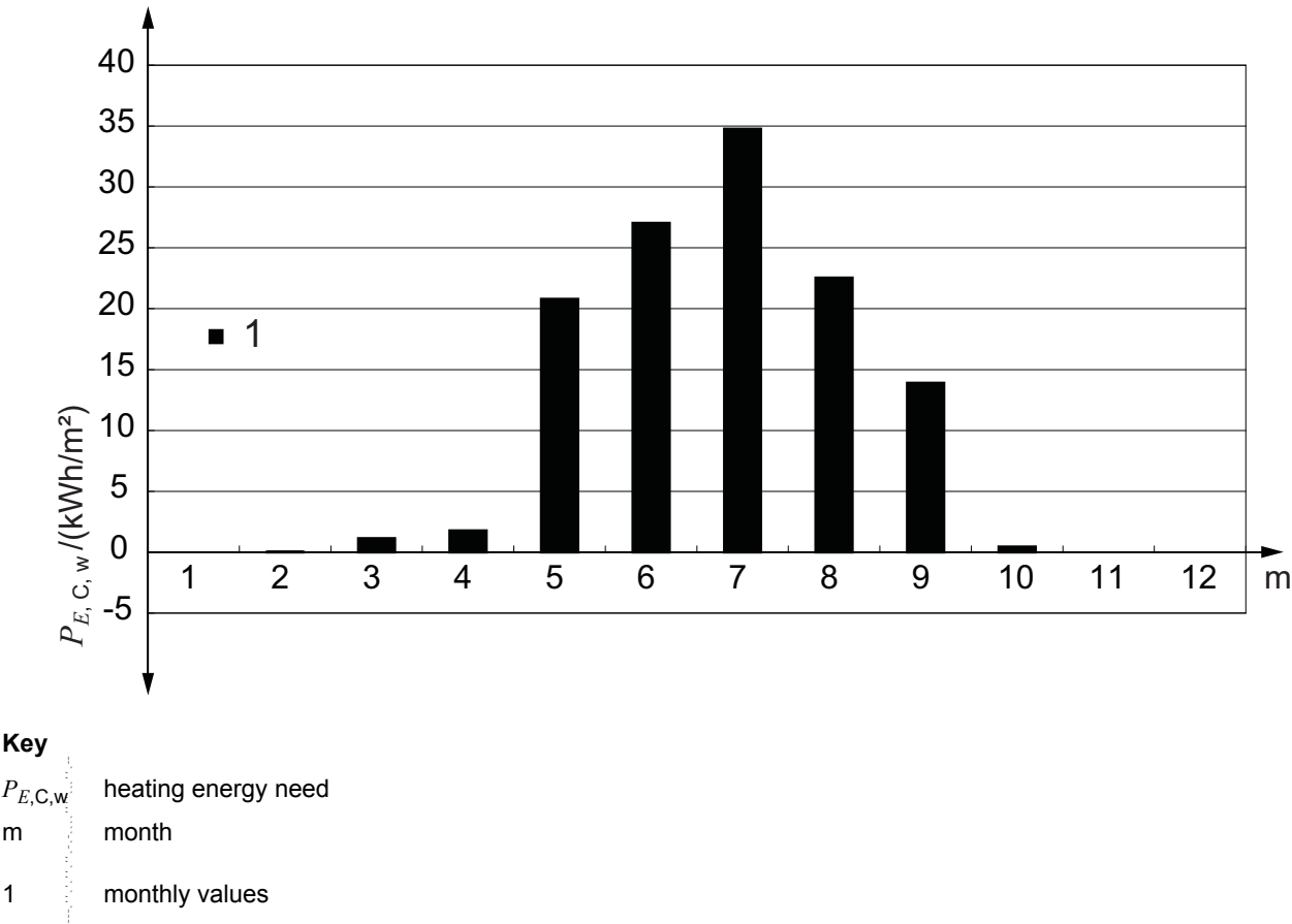
Figure C.3 — Energy performance of fenestration system for cooling, monthly values
