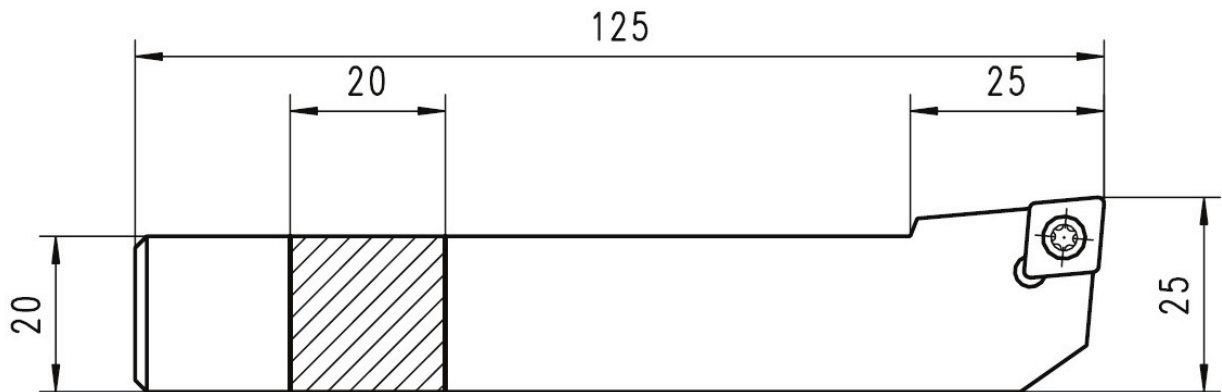
Figure A.1 — Tool holder SCLCR2020K12
