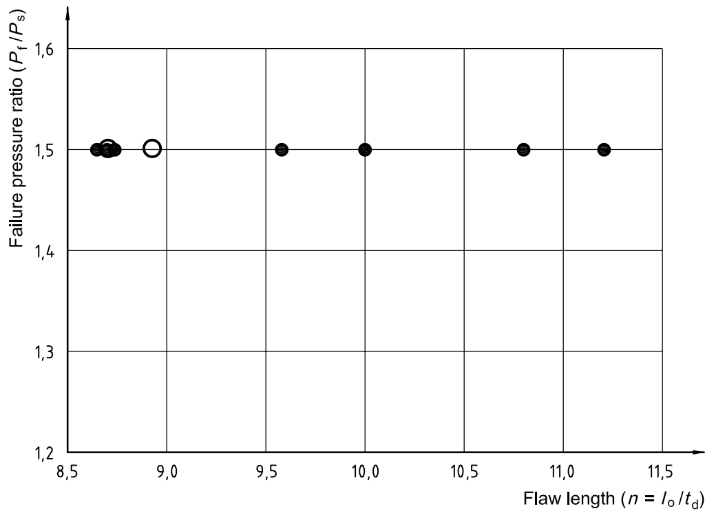
Figure 2 — Defining the leak-fracture boundary
