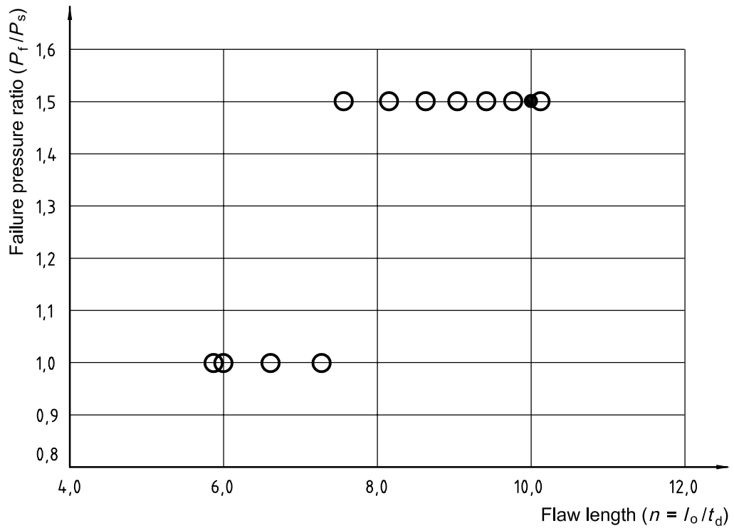
Figure 4 — Flawed-cylinder burst test results for C-5 material
