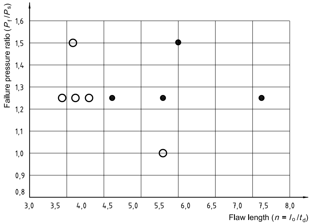
Figure 6 — Flawed-cylinder burst test results for D-7 material
