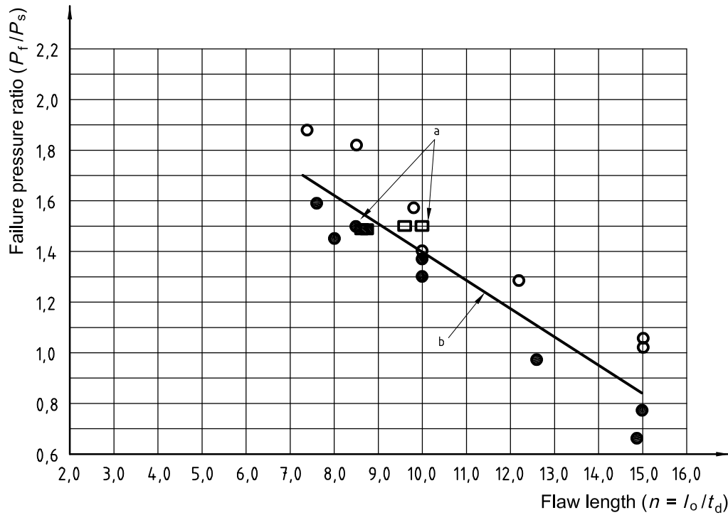
Key • Burst – leak ○ Burst – fracture ■ Cycle – leak □ Cycle – fracture a Cycle tests b Leak-fracture boundary
