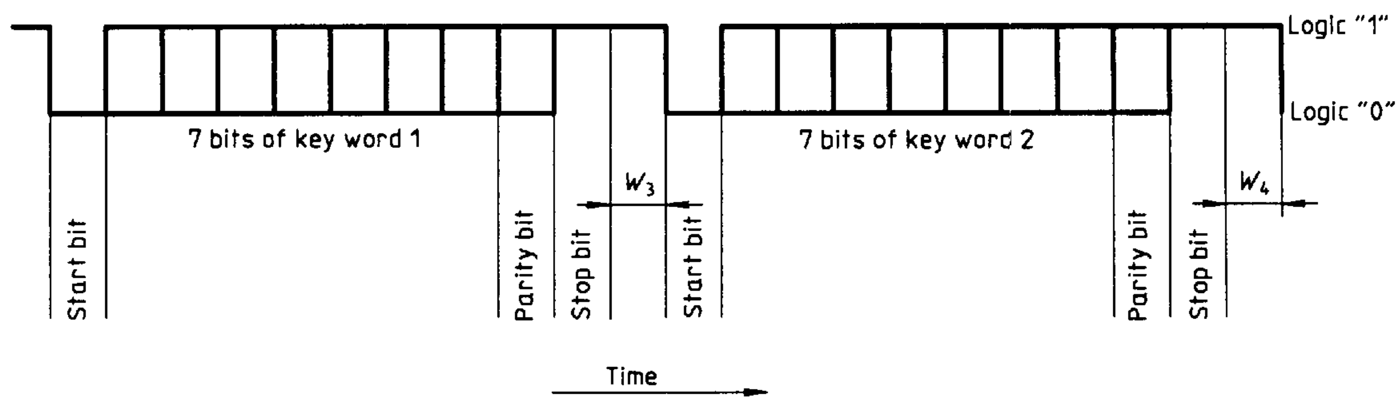
Figure 5 — Key word format
