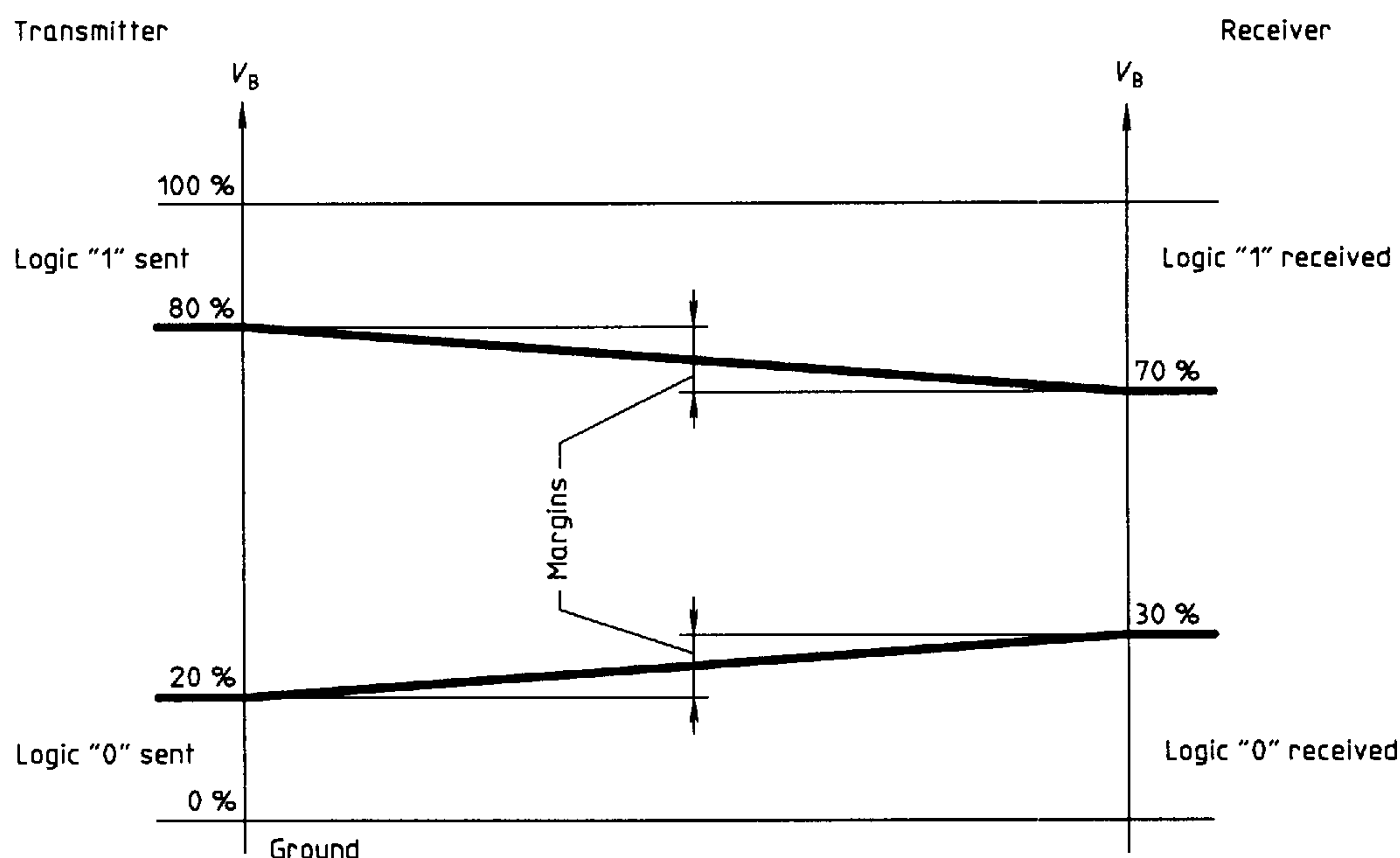
Figure 2 — Signal voltage levels, worst-case values
