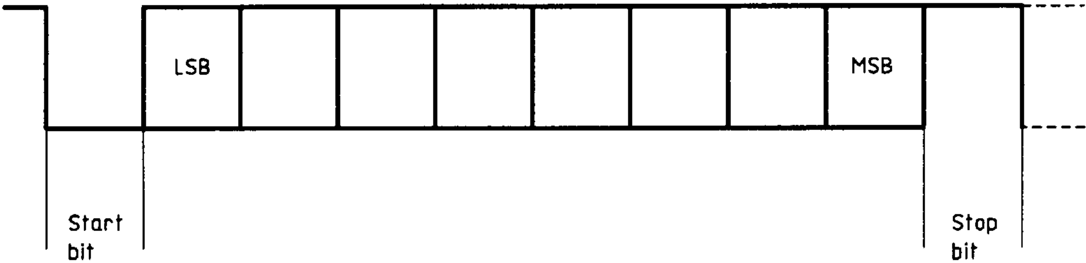
Figure 7 — Byte format
