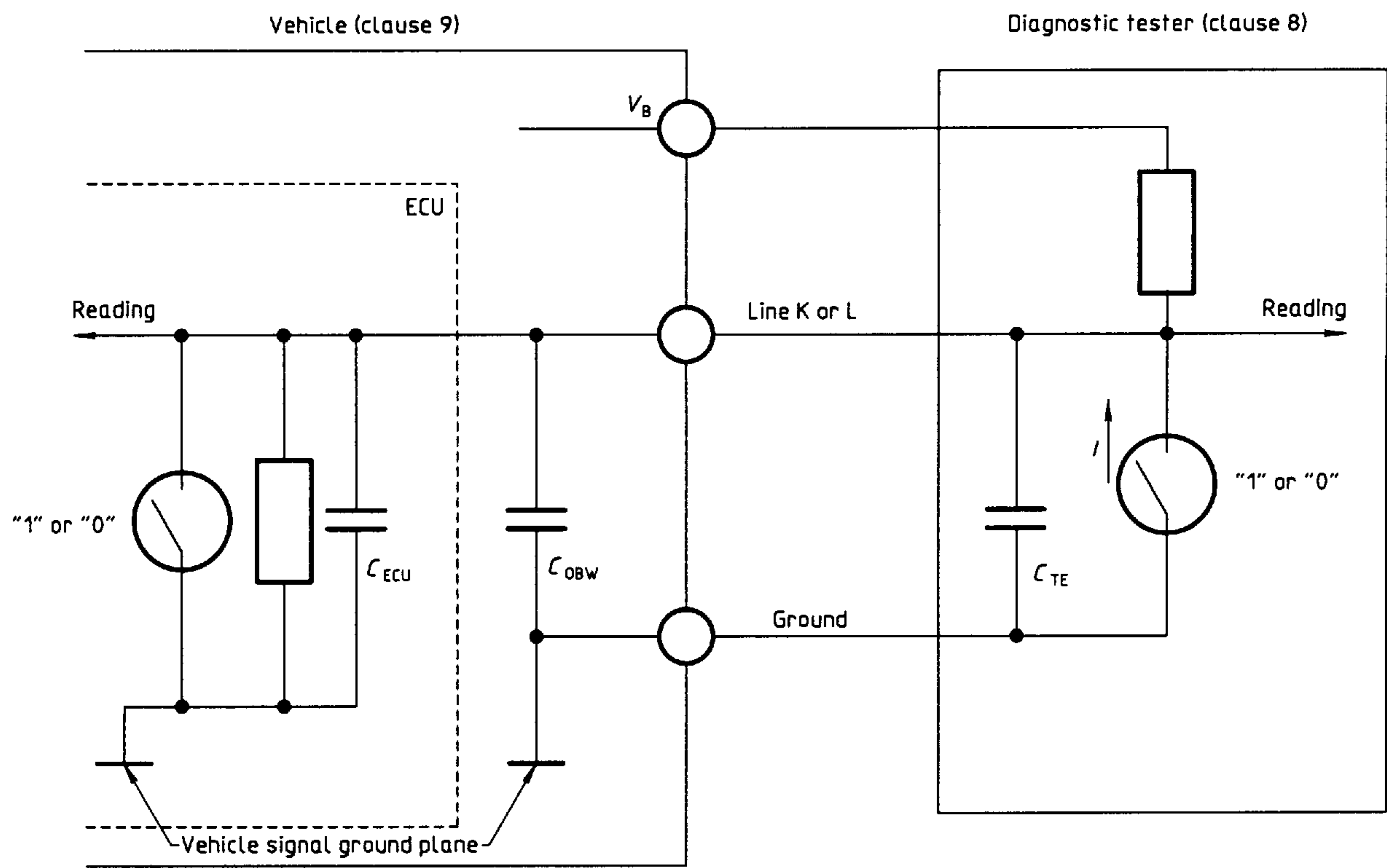
Figure 3 — Vehicle signal ground plane
