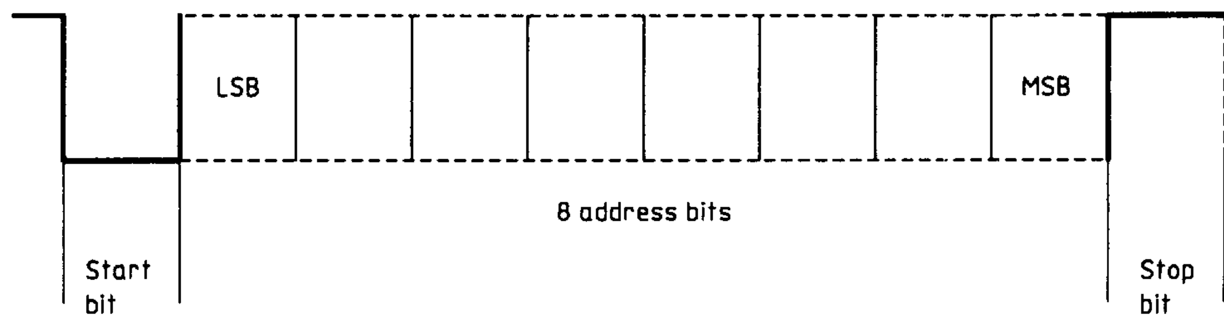
Figure 4 — Initialization format
