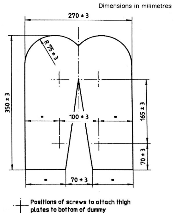
Figure 11 — Thigh plate for 50 kg dummy
