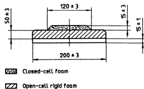
Figure 8 — Backplate for 50 kg dummy
