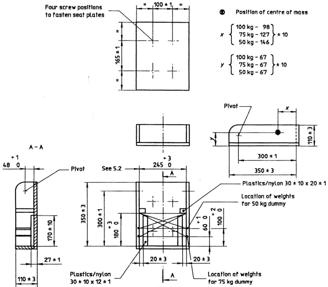
Figure 2 — Test dummy devices of 100 kg, 75 kg and 50 kg: seat construction
