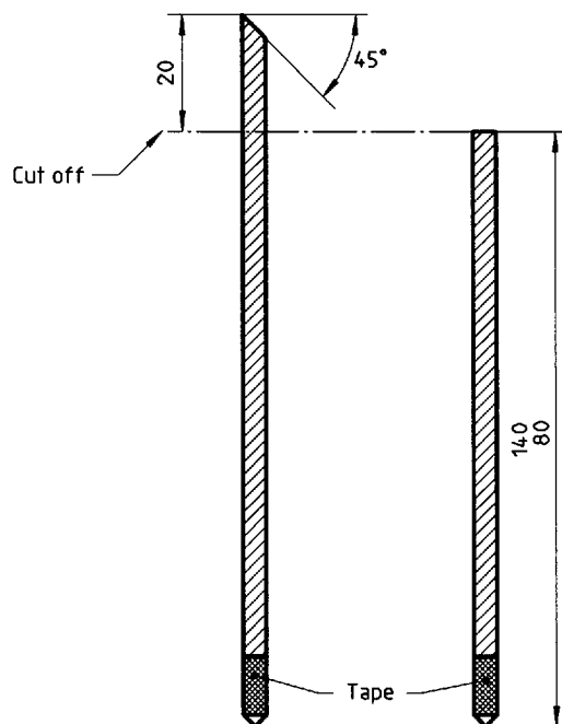
Figure 4 — Rolled specimen
