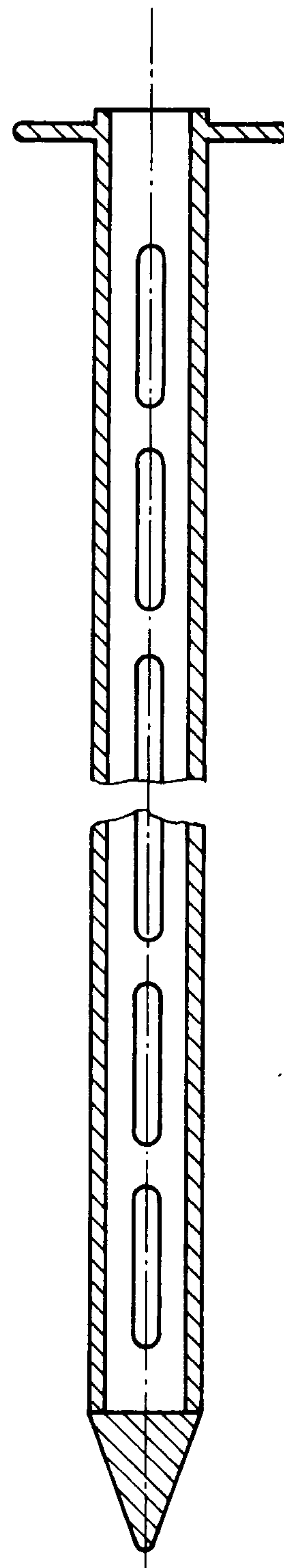
Outer tube
