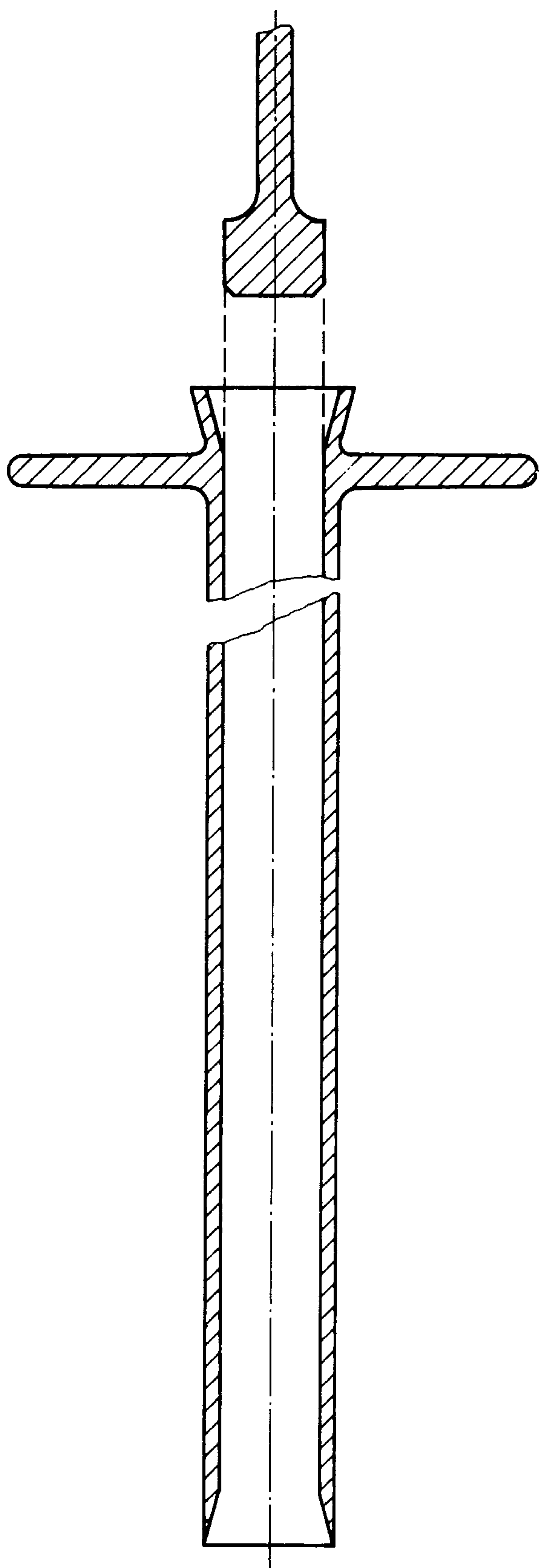
Sampling tube for paste
