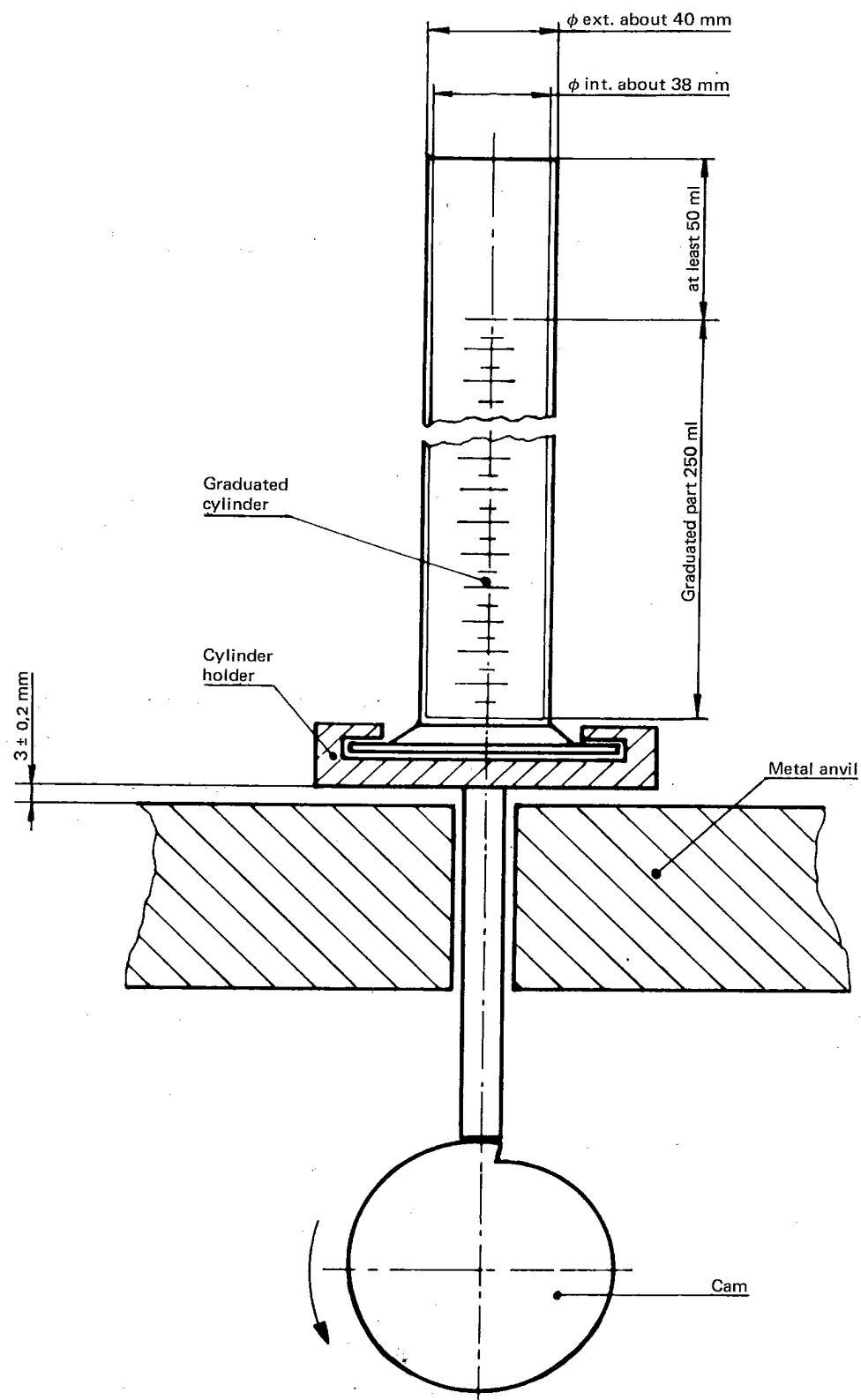
FIGURE — Test apparatus
