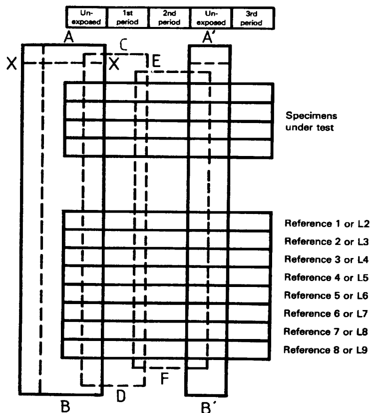
Figure 3 — Mounting of specimens and references for exposure method 2
