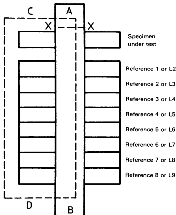
Figure 2 — Mounting of specimen and references for exposure method 1
