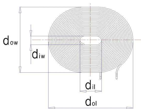
Figure 24. Primary Coil of Power Transmitter design A8
