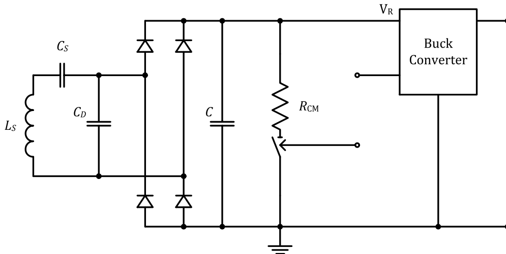
Figure 205. Electrical details of Power Receiver example 2
