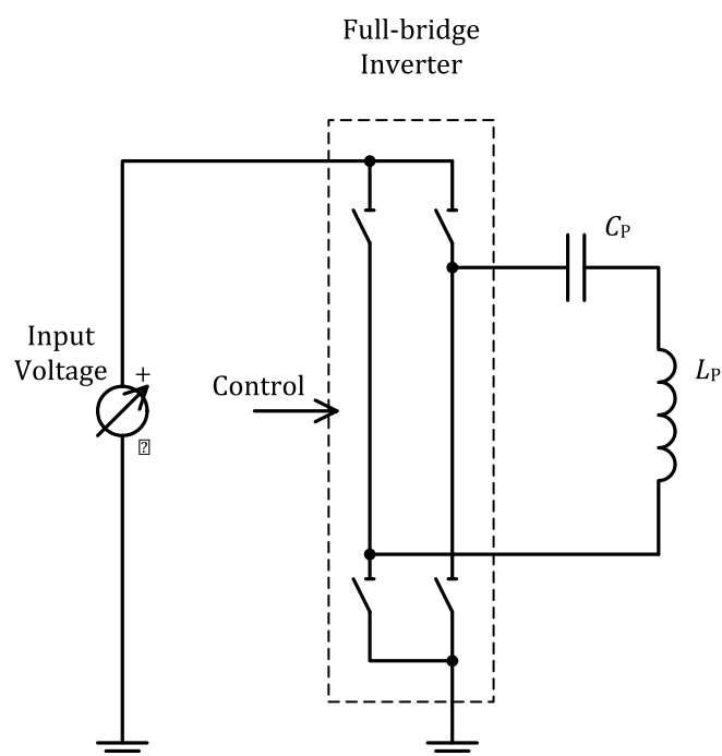
Figure 52. Electrical diagram (outline) of Power Transmitter design A15
