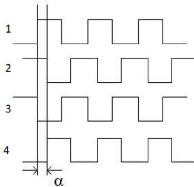
Figure 193. Phase control signals to Full Bridge inverter
