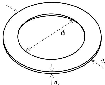
Figure 203. Secondary Coil of Power Receiver example 2
