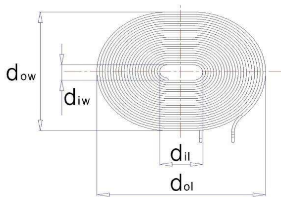
Figure 81. Primary Coil of Power Transmitter design A22
