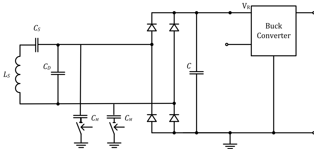
Figure 214. Electrical details of Power Receiver example 5
