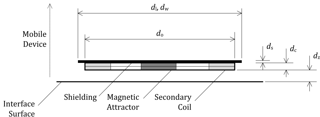
Figure 204. Secondary Coil and Shielding assembly of Power Receiver example 2
