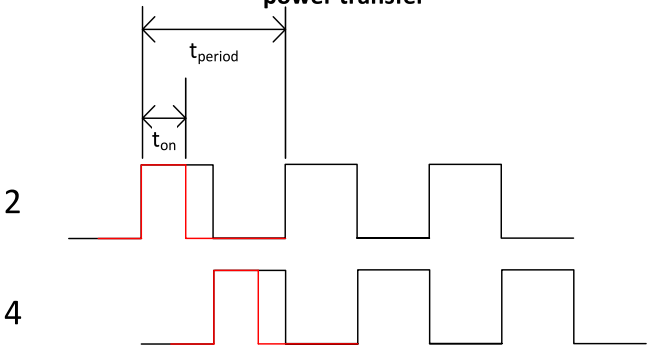
Figure 181. Duty control signals to Half Bridge inverter Phase Difference \alpha is 0, 180° Larger phase difference results in lower power transfer
