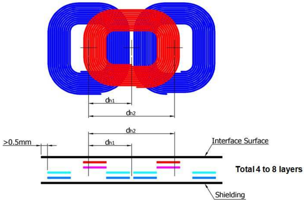
Figure 76. Primary Coils of Power Transmitter design A21
