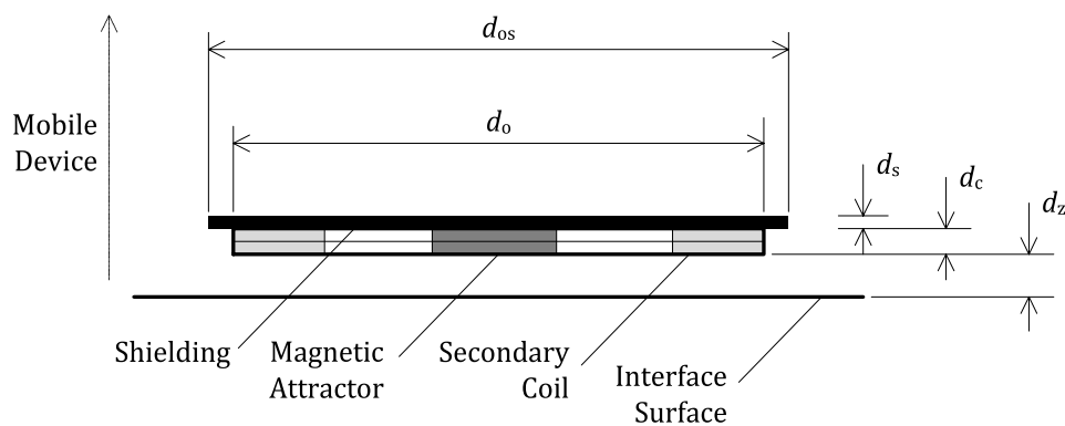
Figure 210. Secondary Coil and Shielding assembly of Power Receiver example 4
