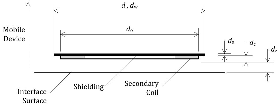
Figure 213. Secondary Coil and Shielding assembly of Power Receiver example 5
