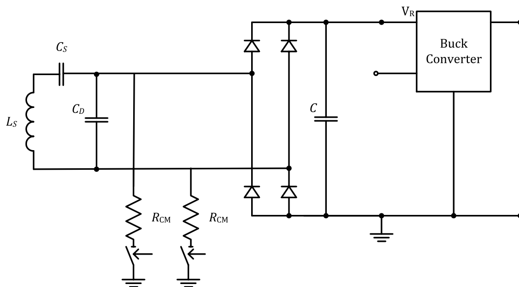
Figure 211. Electrical details of Power Receiver example 4
