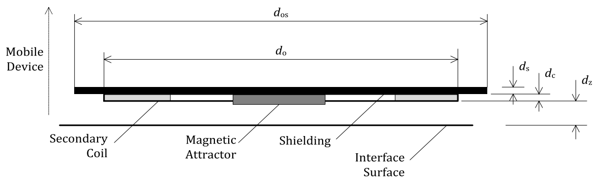
Figure 207. Secondary Coil and Shielding assembly of Power Receiver example 3
