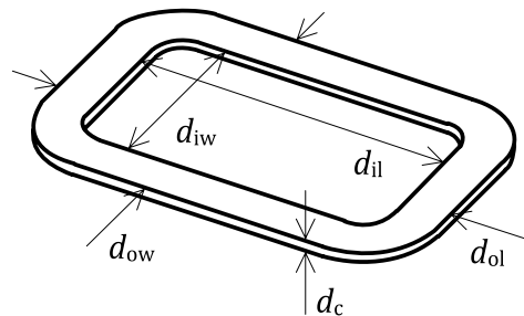
Figure 199. Secondary Coil of Power Receiver example 1
