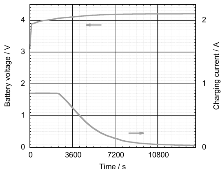
Figure 202. Li-ion battery charging profile
