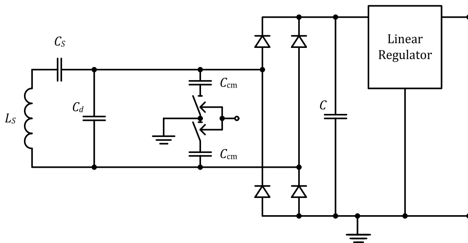
Figure 208. Electrical details of Power Receiver example 3
