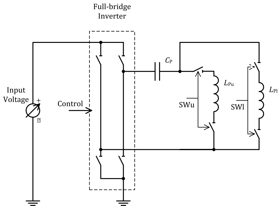
Figure 14. Electrical diagram (outline) of Power Transmitter design A4
