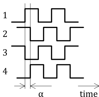
Figure 104. Control signals to the inverter
