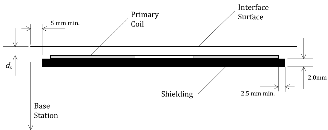
Figure 72. Primary Coil assembly of Power Transmitter design A20
