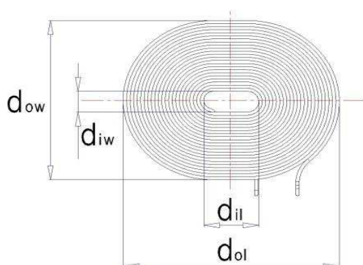
Figure 11. Primary Coil of Power Transmitter design A4
