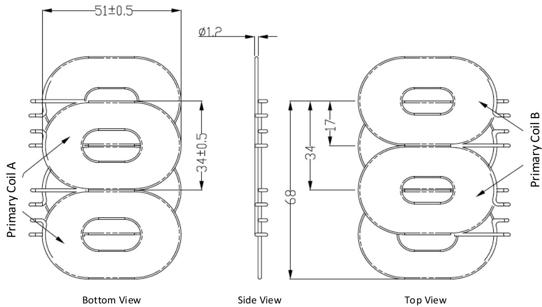
Figure 173. Example of Power Transmitter design B7 in a 4-coil execution
