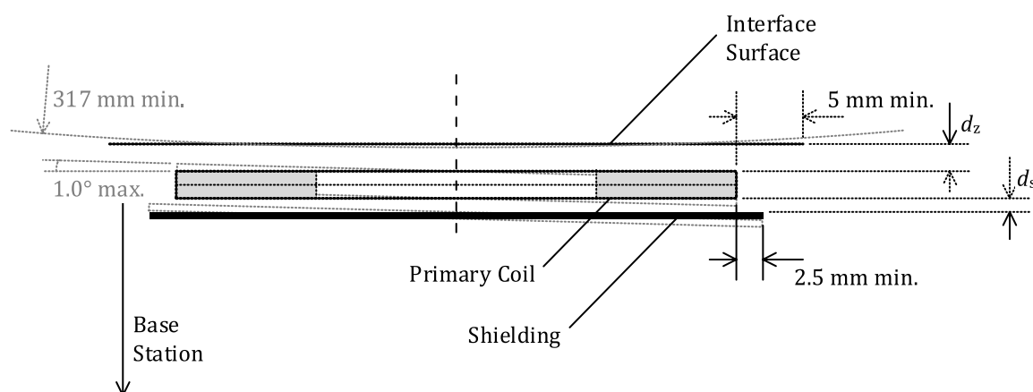
Figure 184. Primary Coil assembly of Power Transmitter design MP-A2
