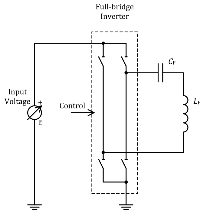
Figure 64. Electrical diagram (outline) of Power Transmitter design A18
