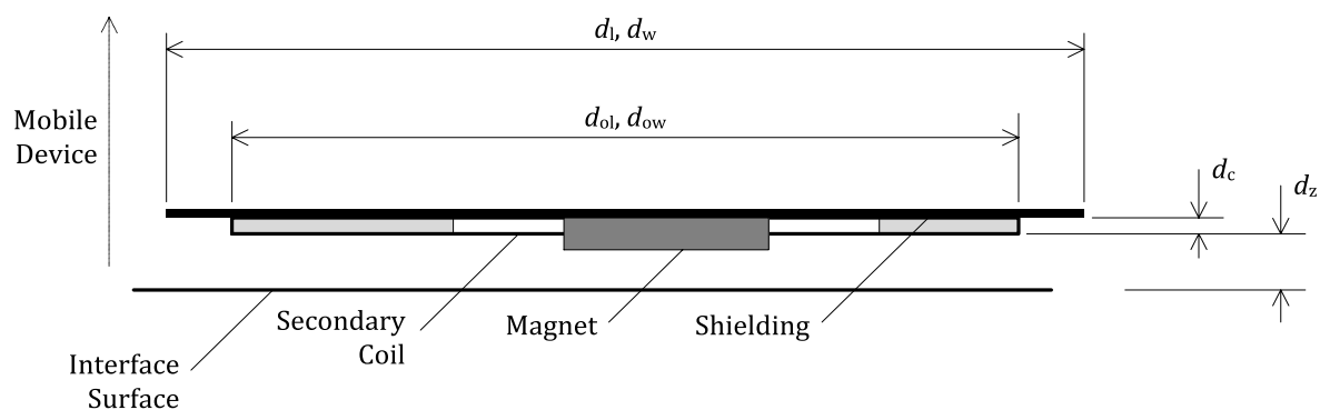
Figure 200. Secondary Coil and Shielding assembly of Power Receiver example 1
