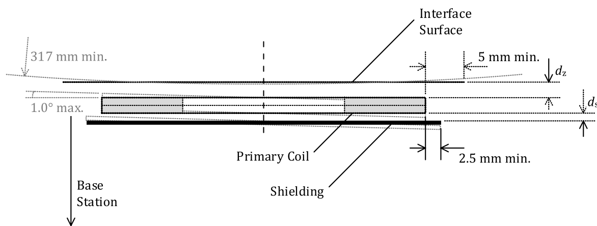
Figure 55. Primary Coil assembly of Power Transmitter design A16
