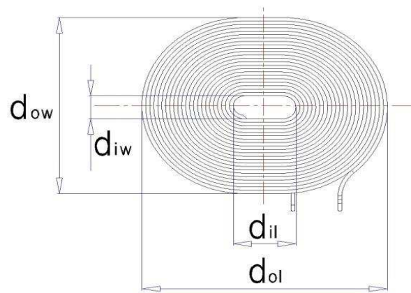
Figure 115. Primary Coil of Power Transmitter design A30
