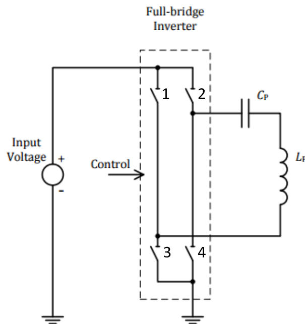
Figure 179. Electrical diagram (outline) of Power Transmitter design MP-A1
