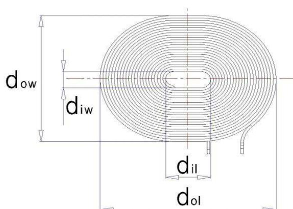
Figure 71. Primary Coil of Power Transmitter design A20
