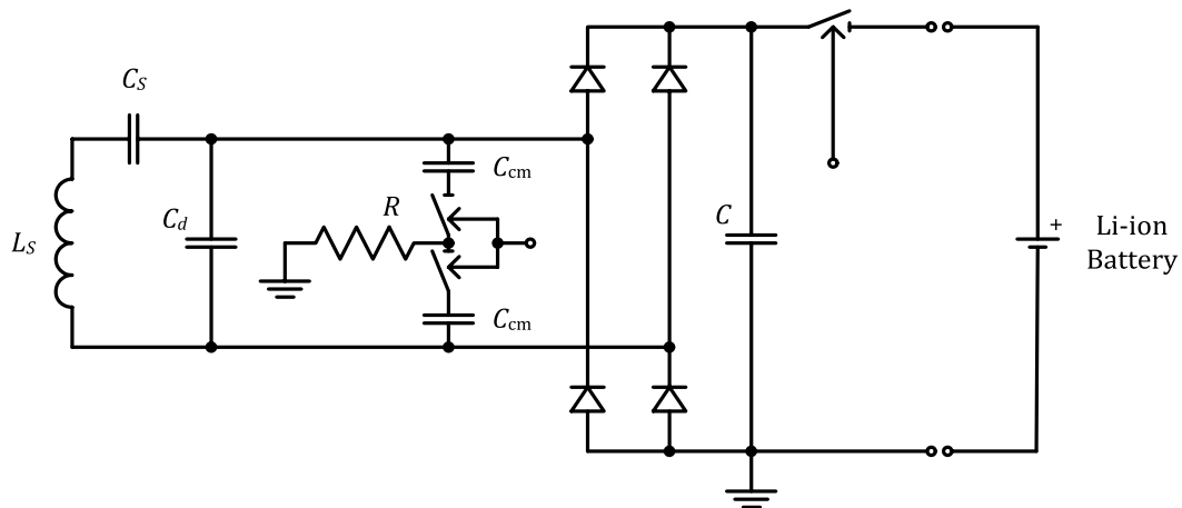
Figure 201. Electrical details of Power Receiver example 1
