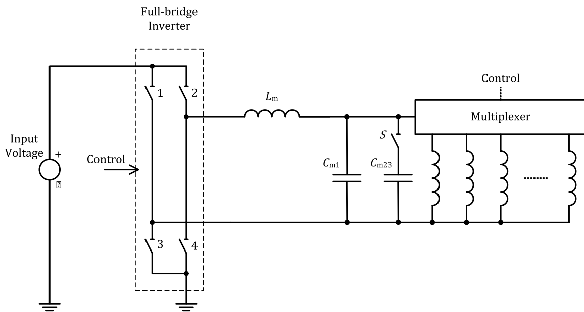
Figure 175. Electrical diagram (outline) of Power Transmitter design B7
