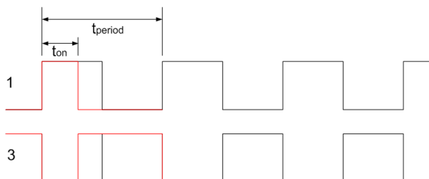
Figure 194. Duty control signals to Half Bridge inverter
