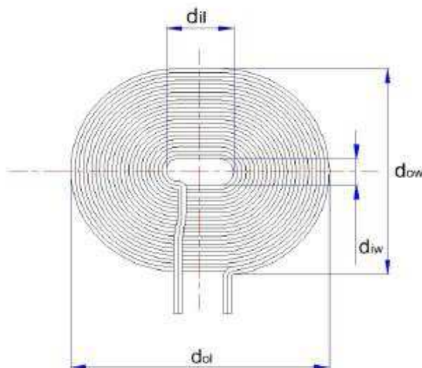
Figure 93. Primary Coil of Power Transmitter design A25
