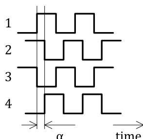
Figure 176. Control signals to the inverter
