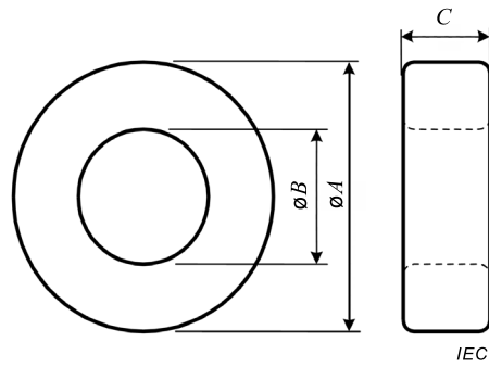
Figure 4 – Ring core
