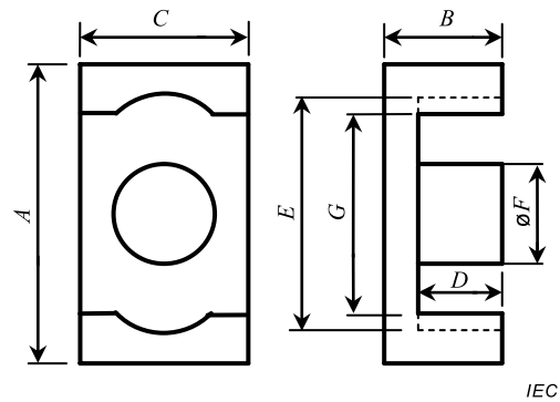
Figure 8 – Planar ER-core
