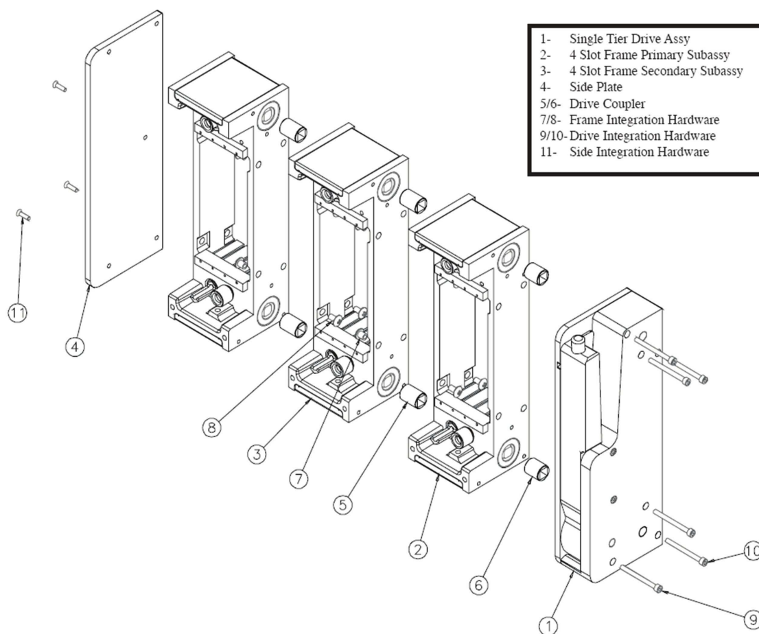
Figure 4—IEEE 1505 receiver segmented framework example
