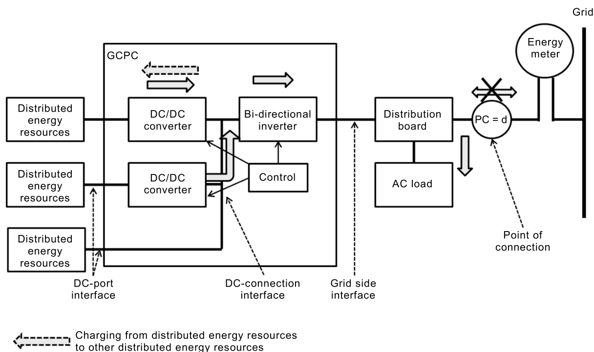
Figure 5 – Power flow of mode IV
