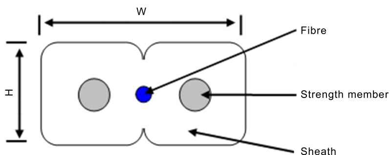
Figure 19a – Cable with high stiffness
