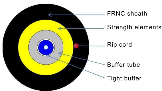
Figure 21a – Facade cable suitable for the installation between fixations using clamps
