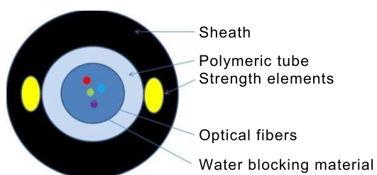
Figure 18 – Lashed cable
