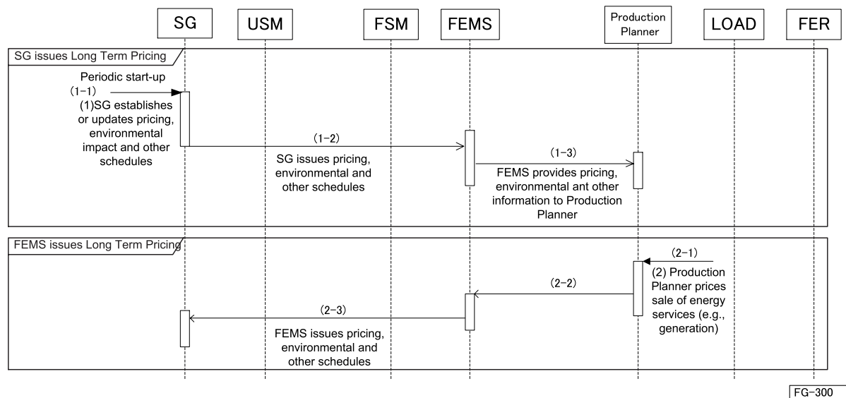
Figure A.4 – Sequence diagram for FG-300
