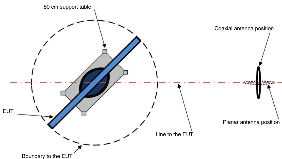
Figure 1 – Setup of a plasma display panel TV for magnetic-field measurement
