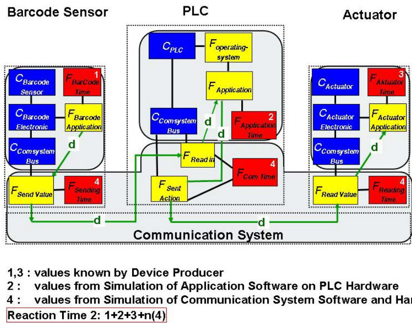
Figure 18 – Performance simulation of a digital factory
