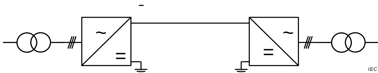
Figure 10 – VSC transmission with an asymmetrical monopole with earth return
