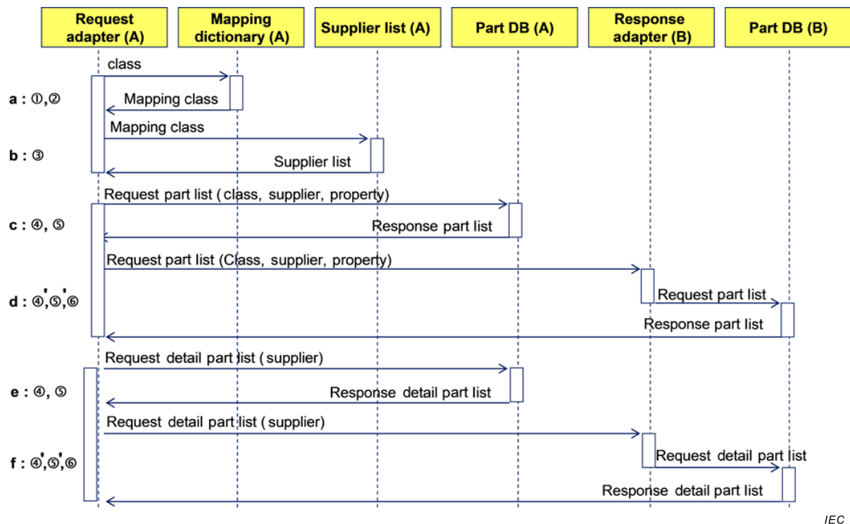
Figure 4 – Sequence diagram
