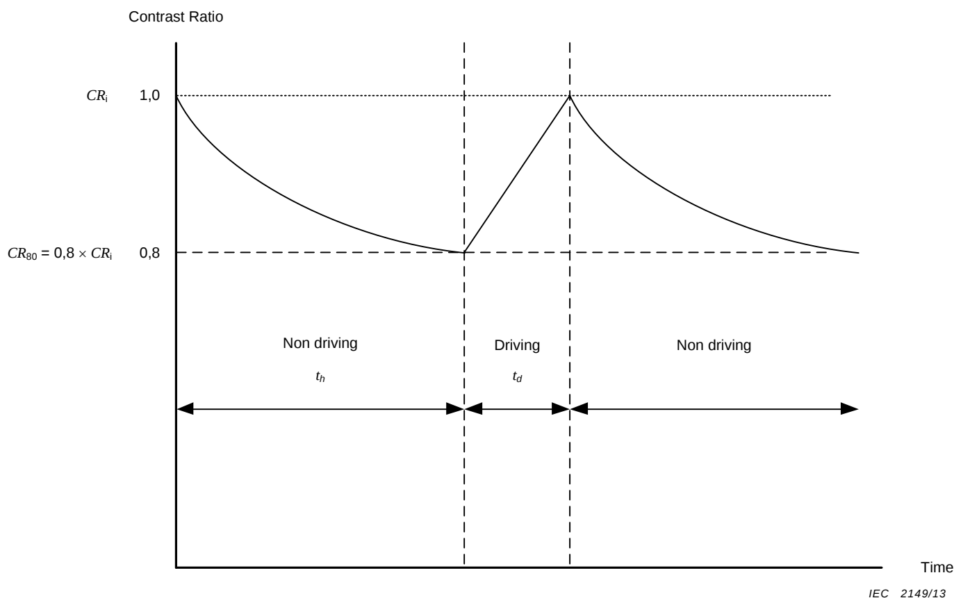
Figure 11 – Image contrast and driving mode
