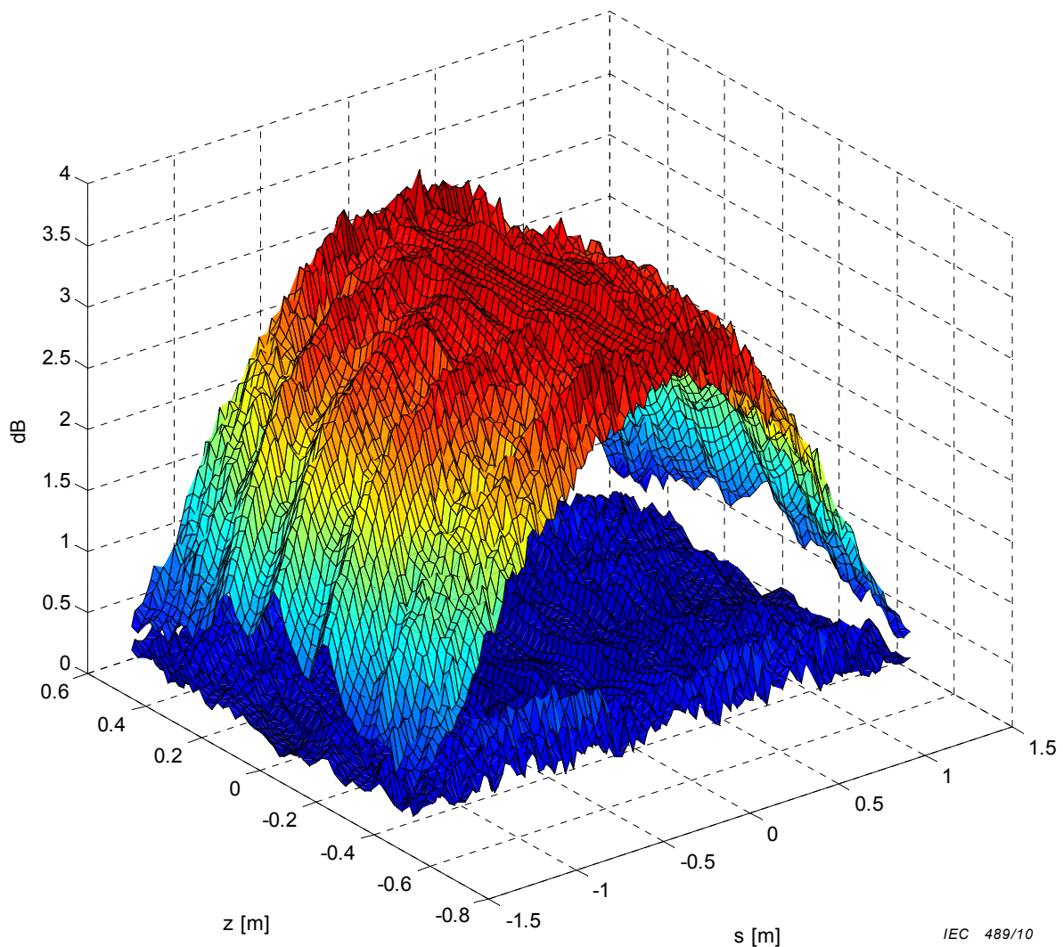
Figure C.6 – Overestimations produced by Equations (10) and (12) over the exposure evaluation area \Sigma_\rho ( \rho = 1 m) for the 3,5 GHz smart antenna shown in Figure C.4
