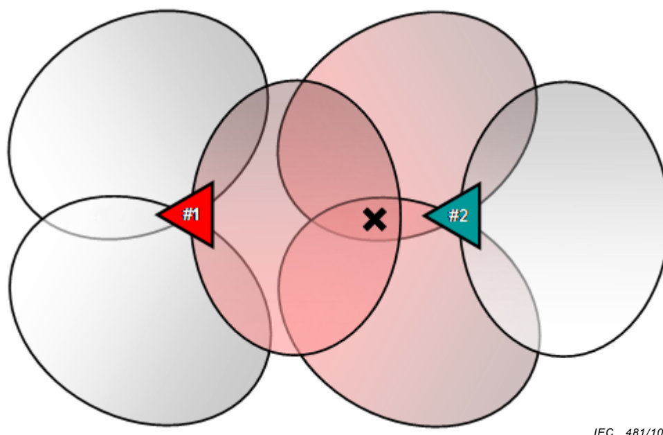
Figure 3 – Simultaneous exposure at the location X by multiple sector-antennas belonging to adjacent tri-sector cellular masts (labelled #1 and #2)
