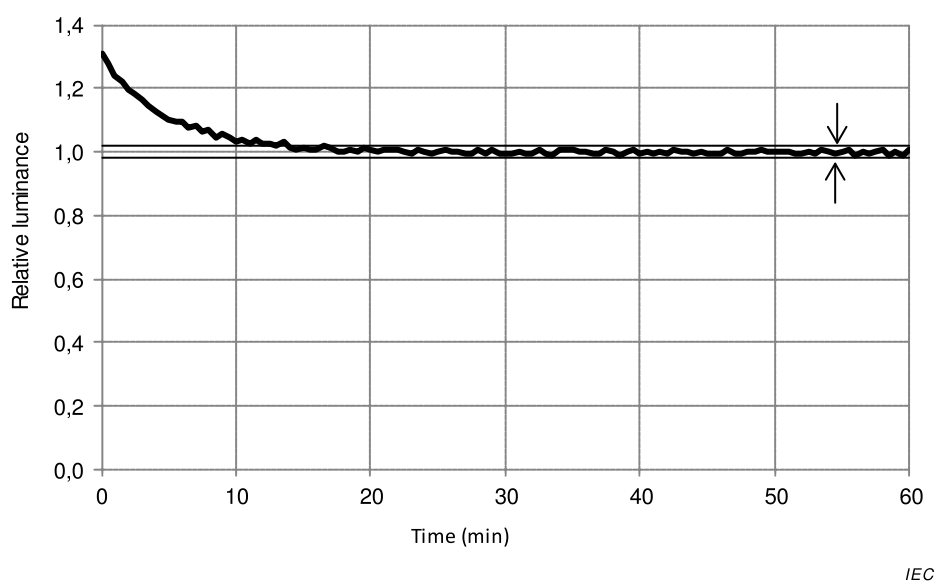
Figure 2 – Example of warm-up characteristic of BLU
