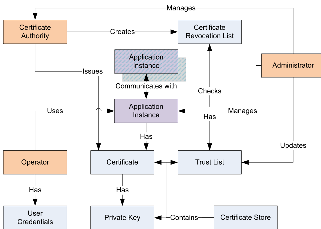
Figure 9 – Certificate handling
