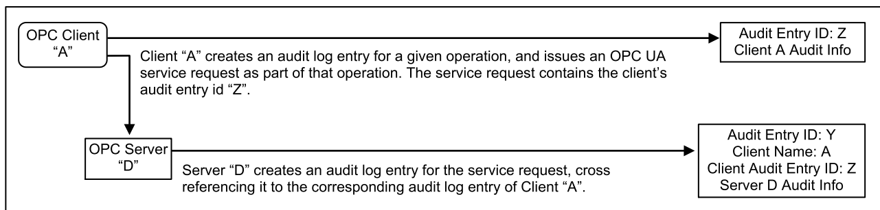
Figure 3 – Simple Servers
