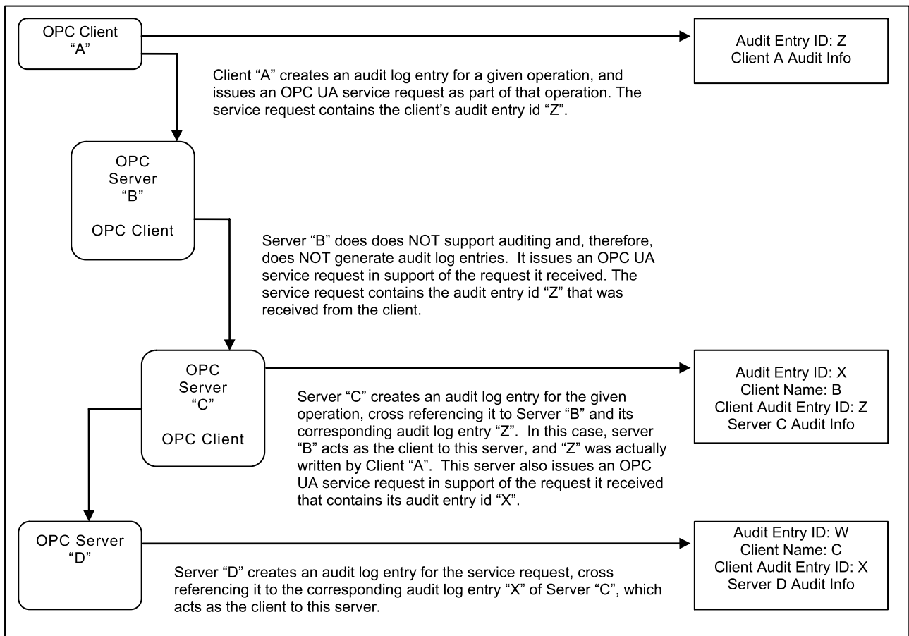
Figure 5 – Aggregation with a non-auditing Server
