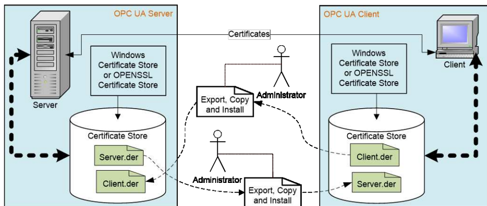
Figure 7 – Manual Certificate handling
