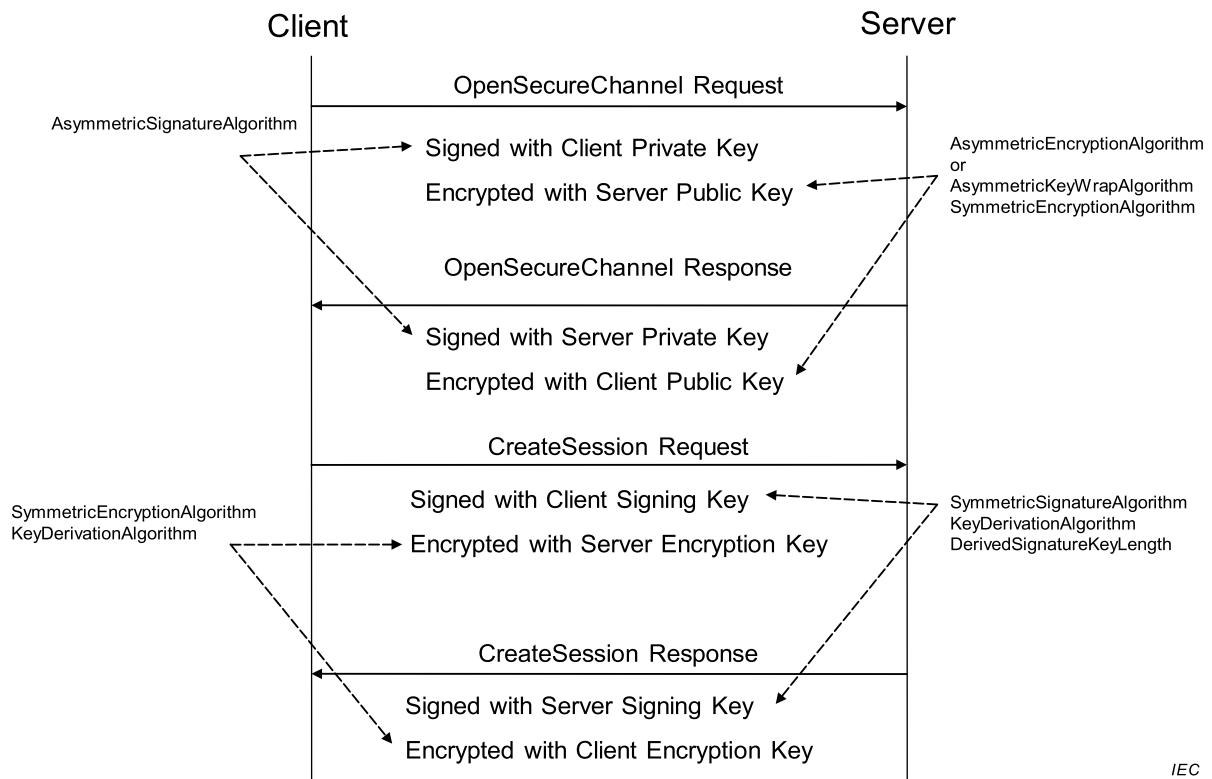
Figure 10 – Security handshake
