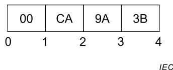
Figure 2 – Encoding Integers in a binary stream
