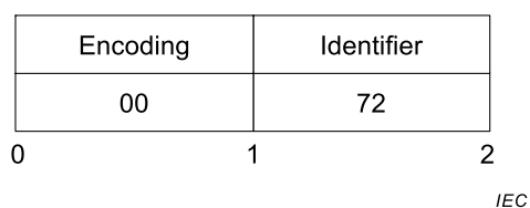
Figure 8 – A Two Byte NodeId
