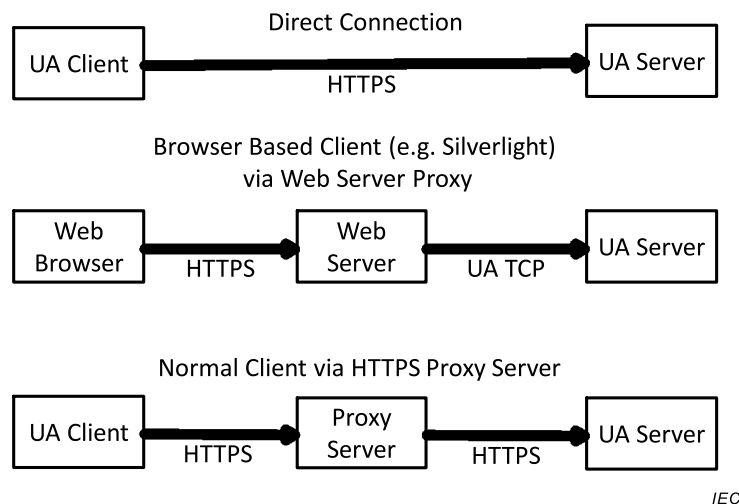
Figure 18 – Scenarios for the HTTPS Transport
