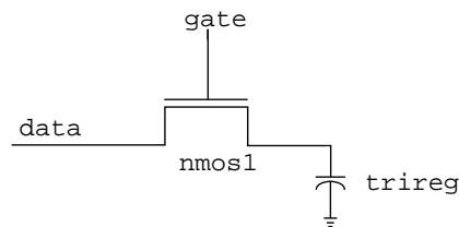
Figure 28-26—Triereg net with capacitance
