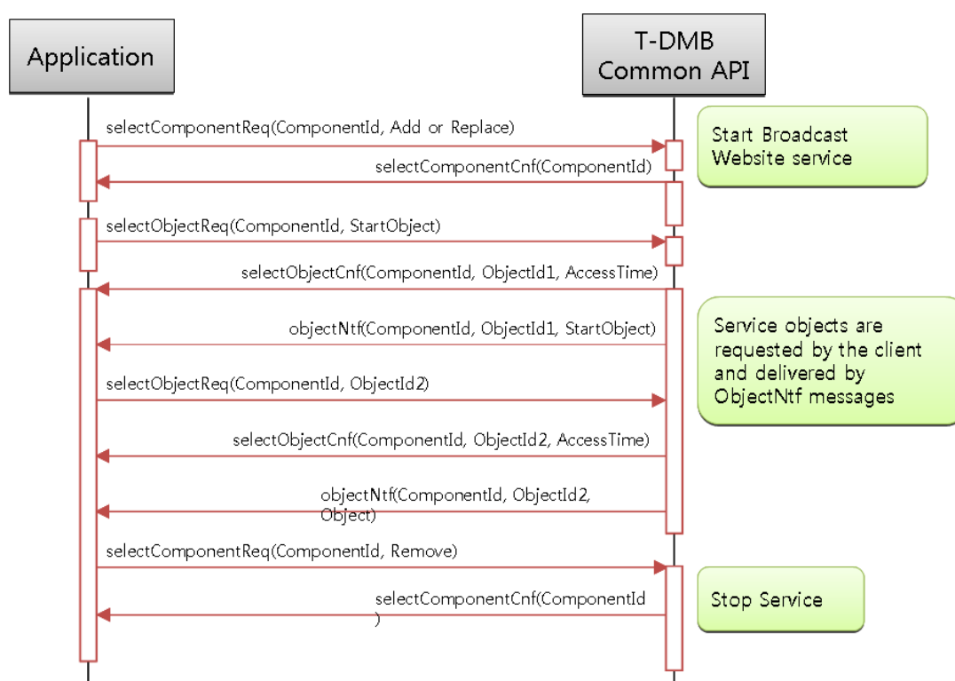
Figure 9 – Selecting a broadcast website service
