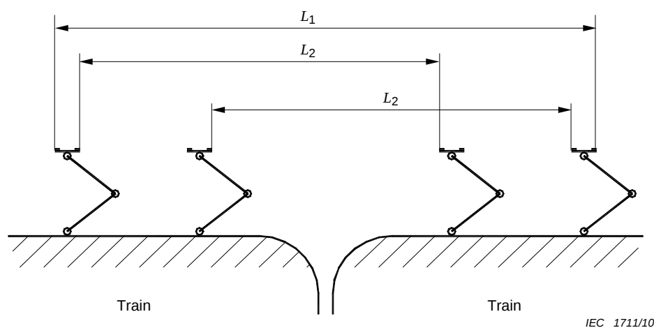
Figure A.6 – Arrangement of pantographs on trains
