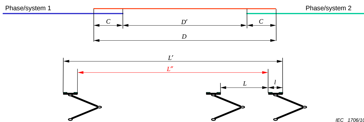
Figure A.1 – Symbol visualisation
