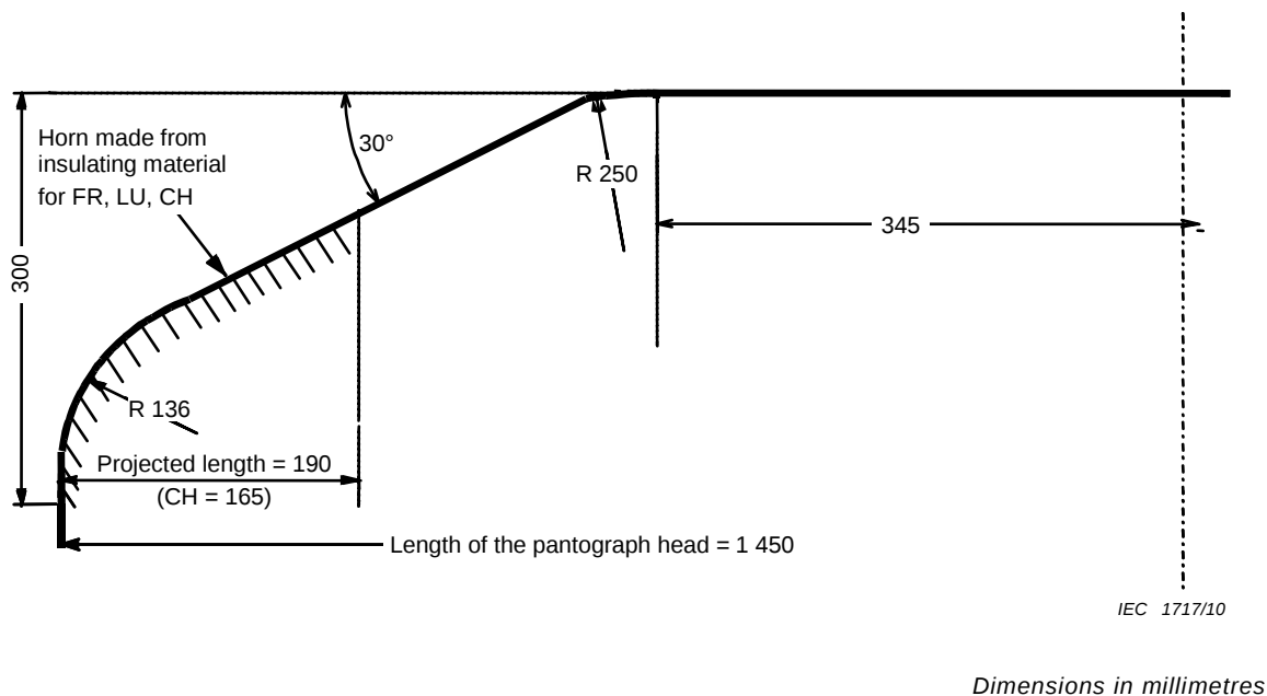
Figure B.2 – Pantograph head with length of 1 450 mm
