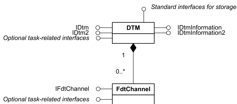
Figure 3 – DTM interfaces
