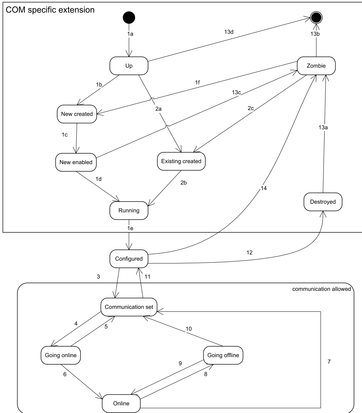
Figure 9 – State machine of a DTM
