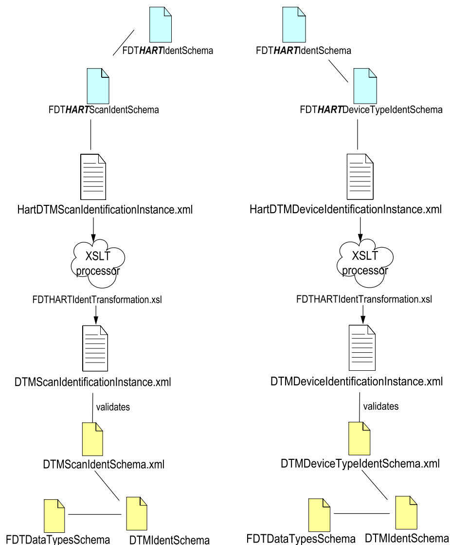
Figure E.1 – XSLT role
