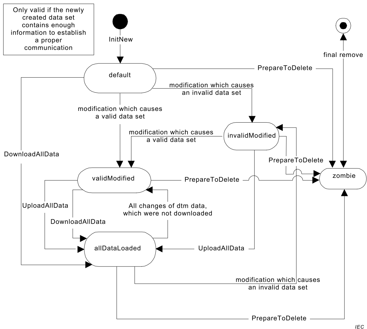
Figure 50 – State machine of instance data set
