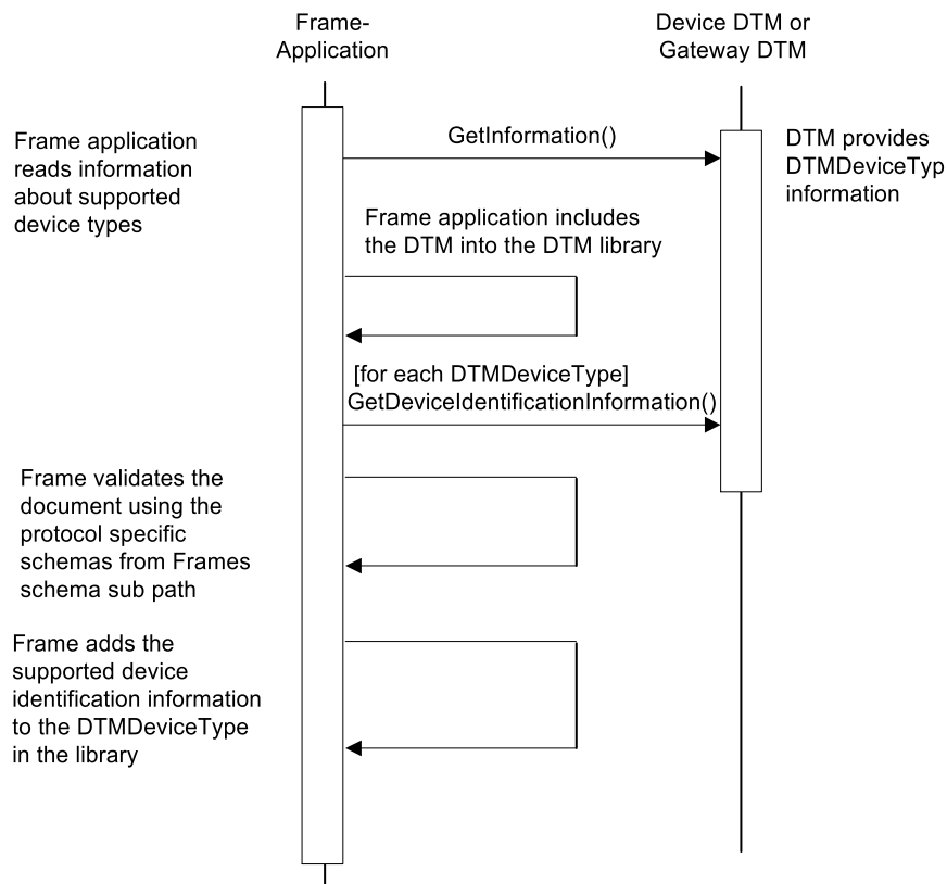
Figure 31 – Frame Application reads protocol-specific device identification information of DTMDDeviceTypes
