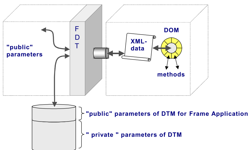
Figure 5 – Data access and storage
