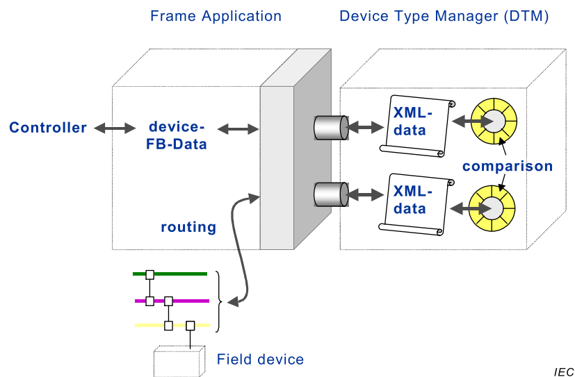
Figure 8 – Parameter verification in case of failsafe devices
