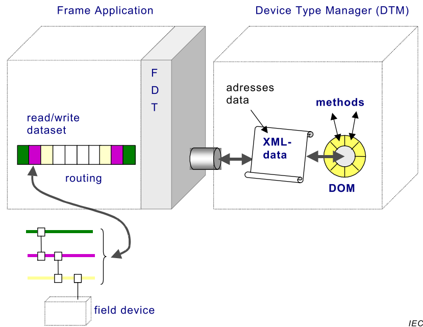
Figure 6 – Communication
