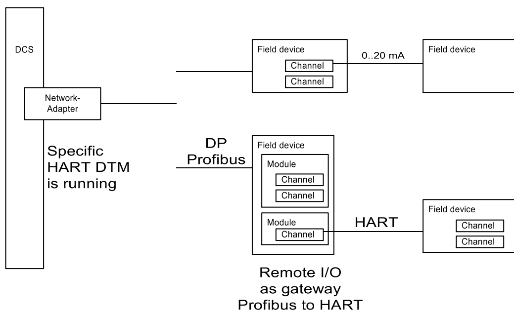
Figure 20 – System-topology
