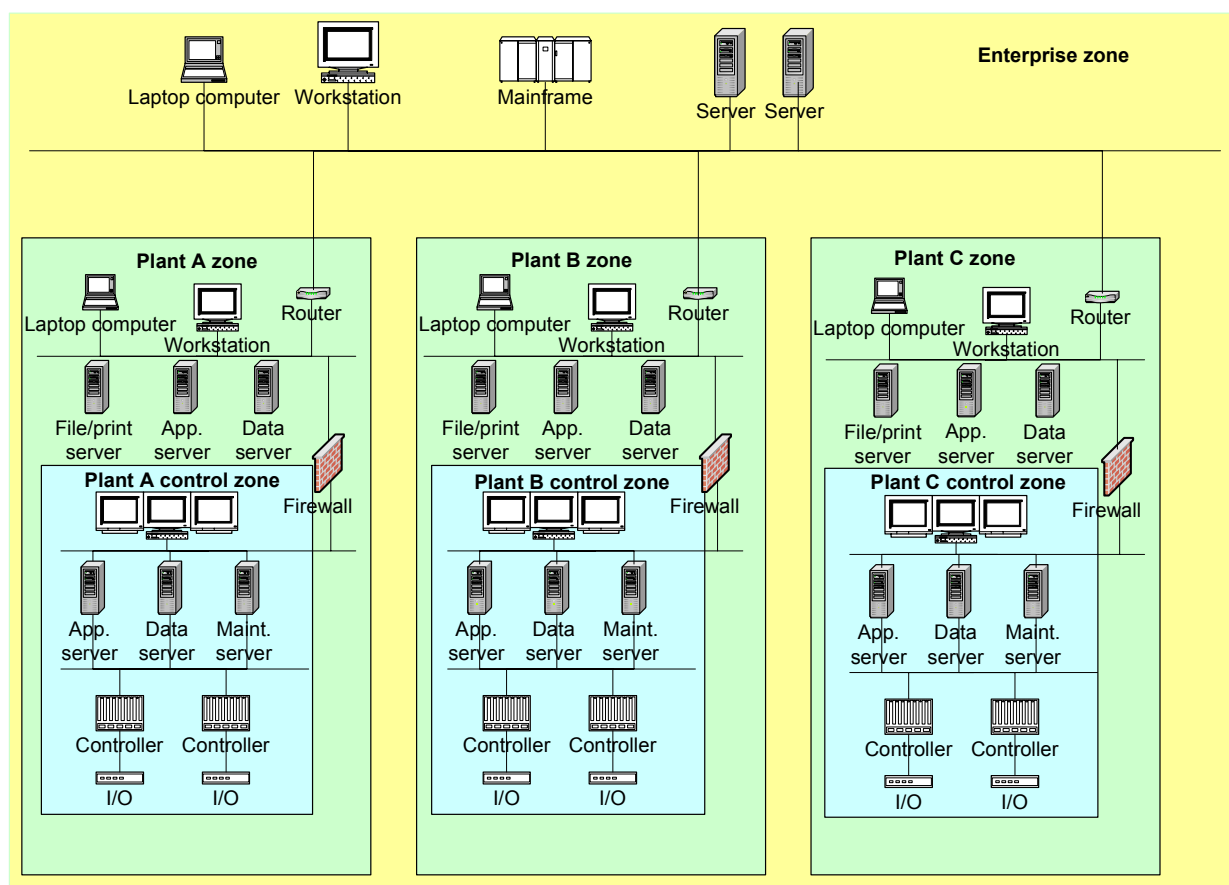
Figure 17 – Multiplant zone example
