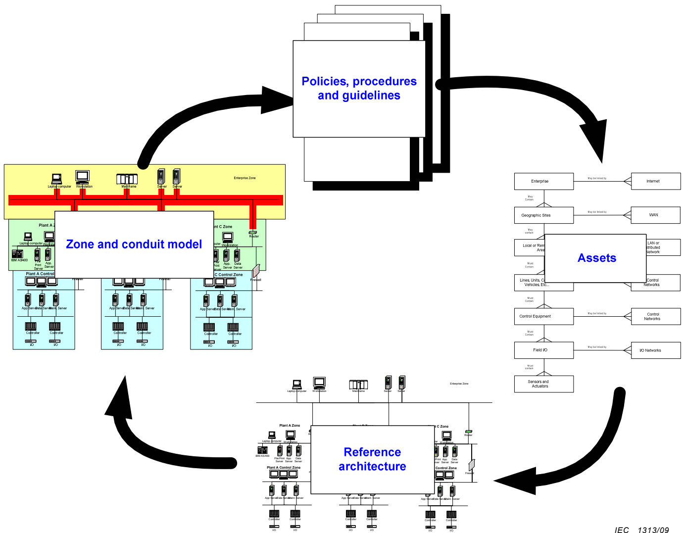
Figure 23 – Model relationships
