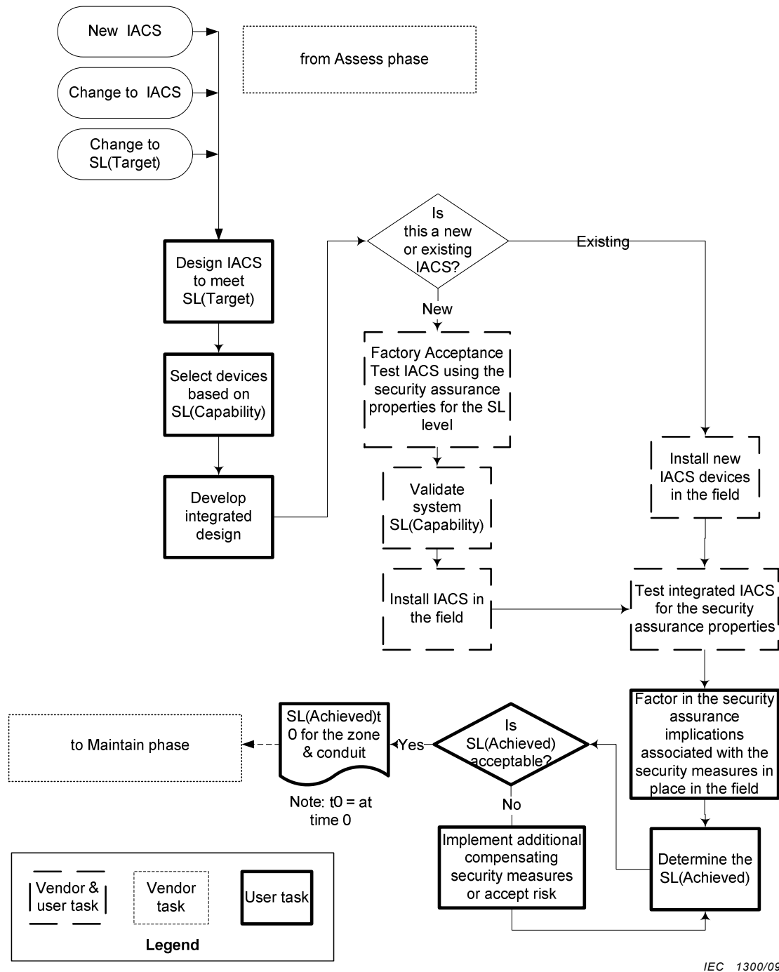
Figure 10 – Security level lifecycle – Implement phase
