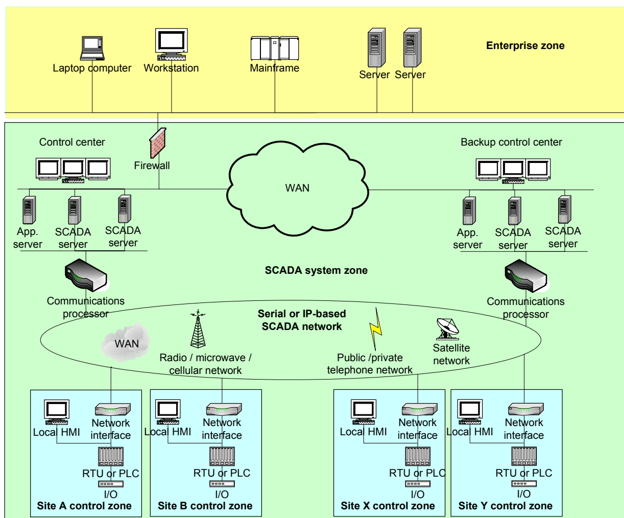
Figure 19 – SCADA zone example
