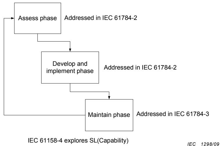
Figure 8 – Security level lifecycle
