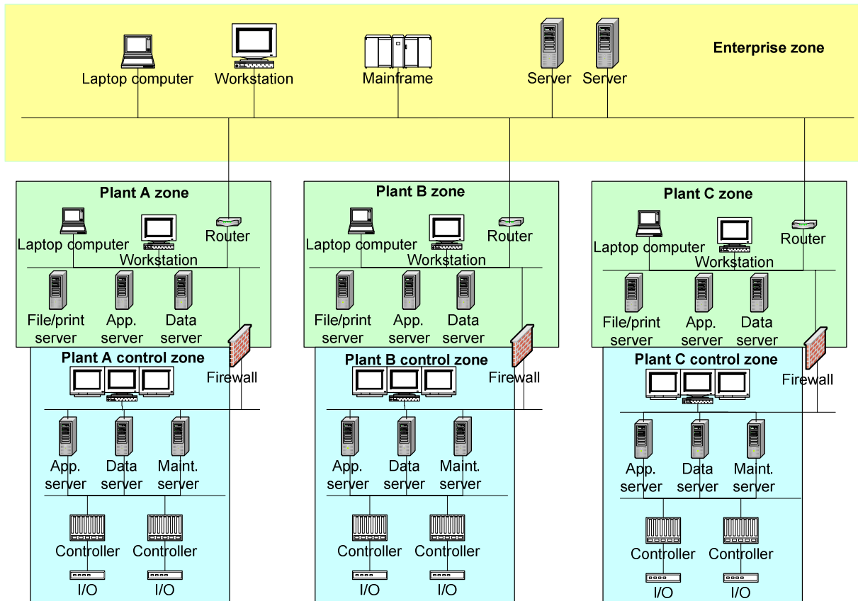
Figure 18 – Separate zones example
