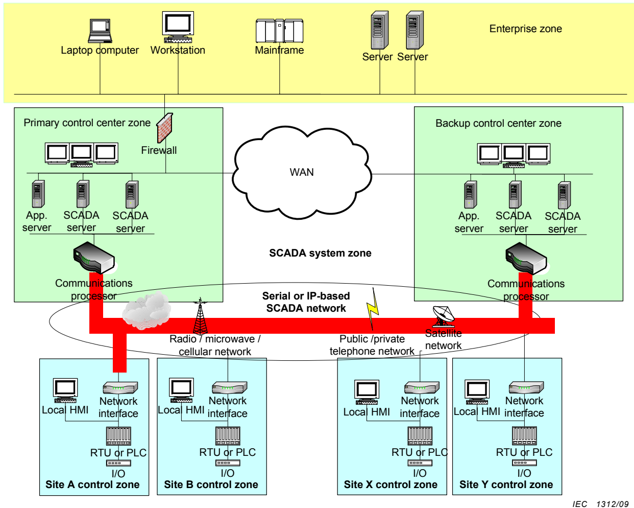
Figure 22 – SCADA conduit example
