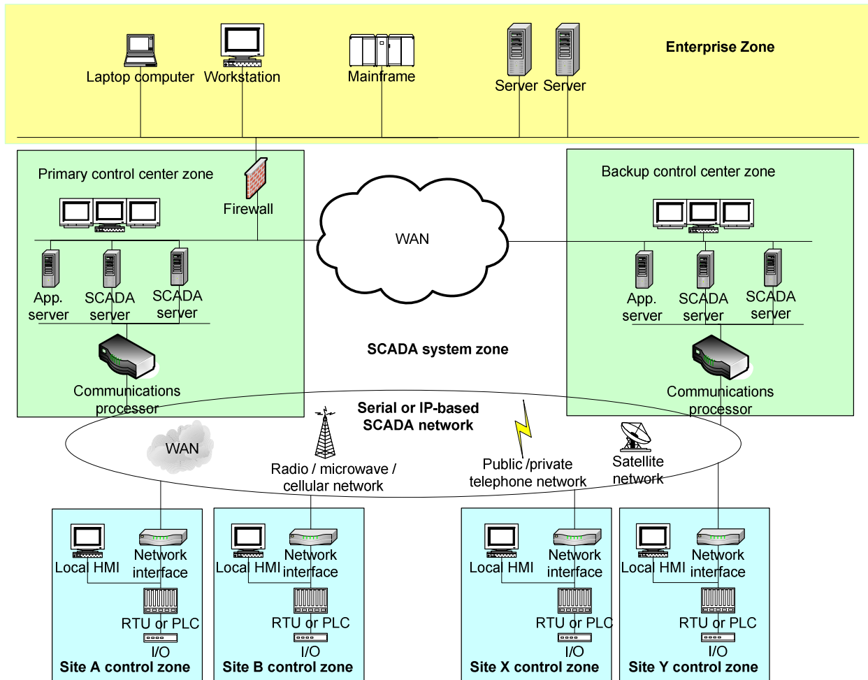
Figure 20 – SCADA separate zones example
