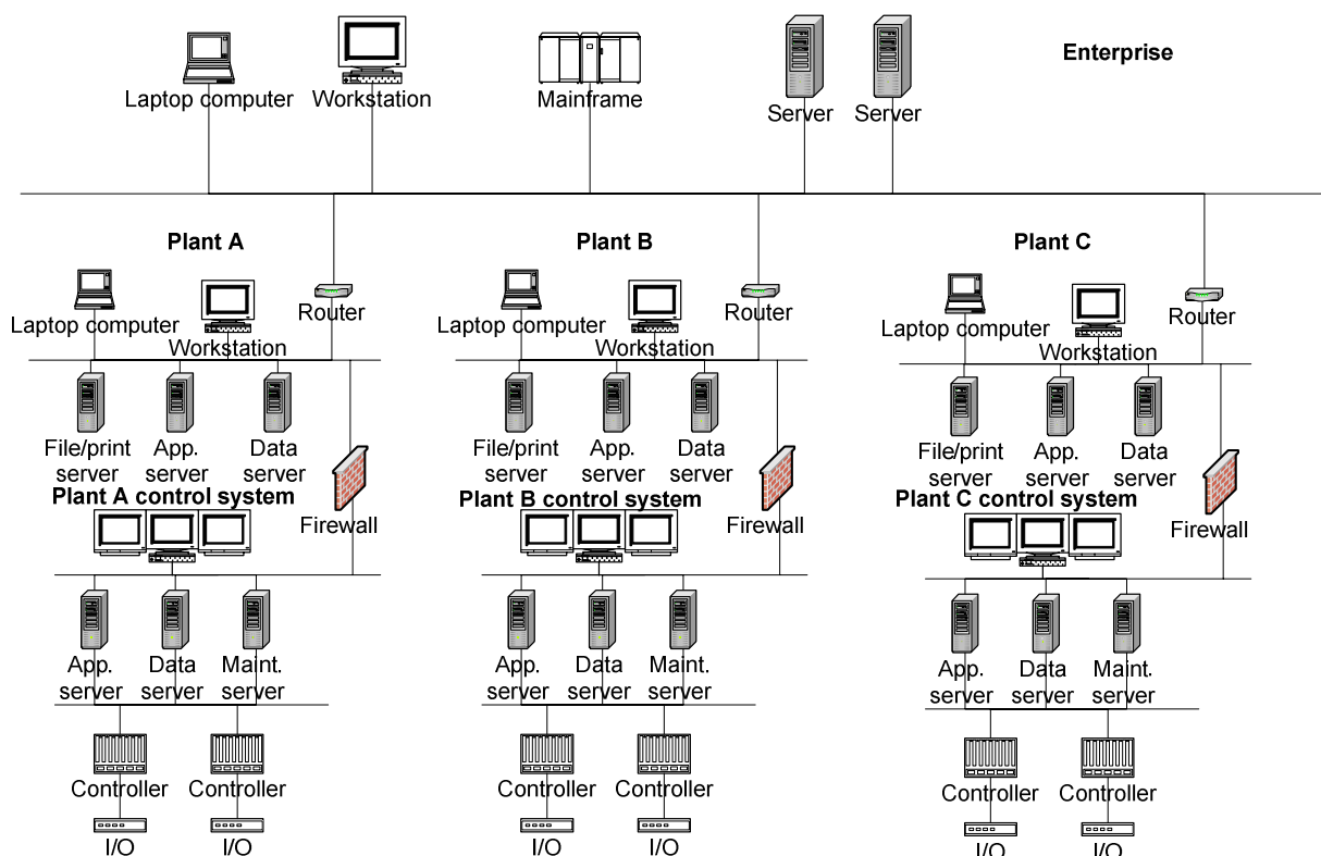
Figure 16 – Reference architecture example
