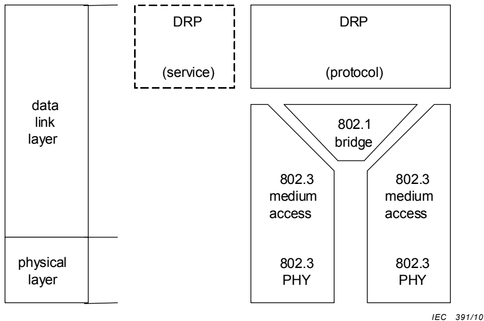
Figure 1 – DRP communication model
