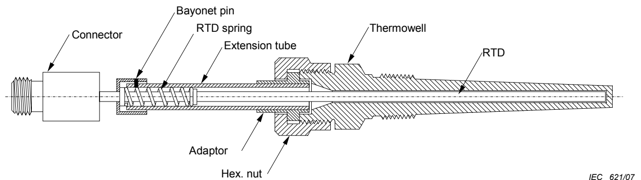
Figure 1 – Form and dimensions of an RTD
