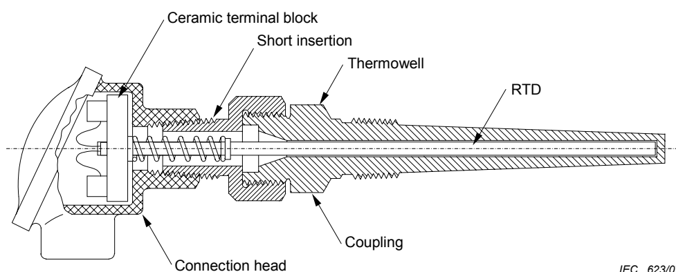
Figure 3 – Installation of a rigid RTD (Type II) long insertion
