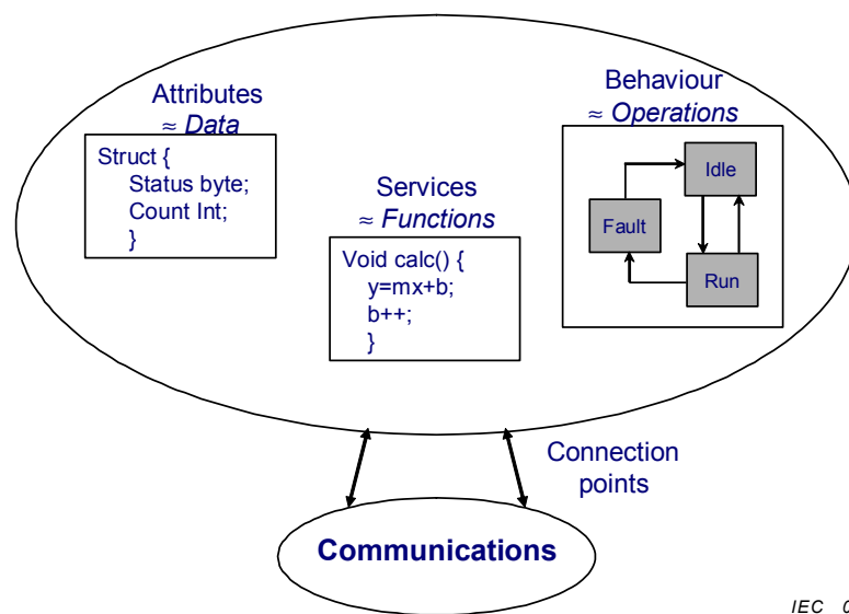
Figure J.1 – Object model elements versus procedural programming elements
