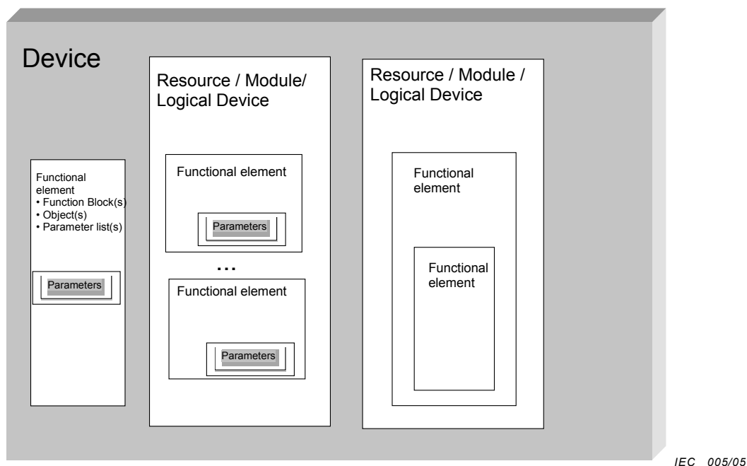
Figure 4 – Example of a modular view of the hardware and software structures of a device
