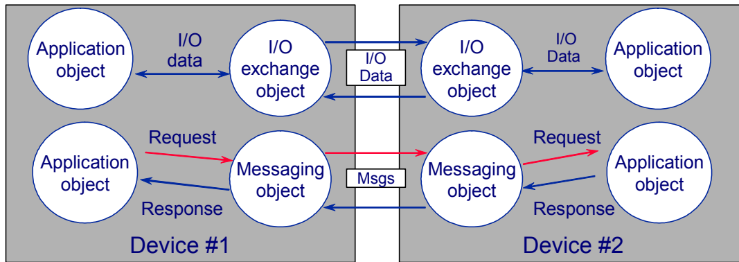
Figure J.6 – Communication management objects (example)
