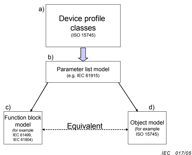
Figure 16 – Device profile models
