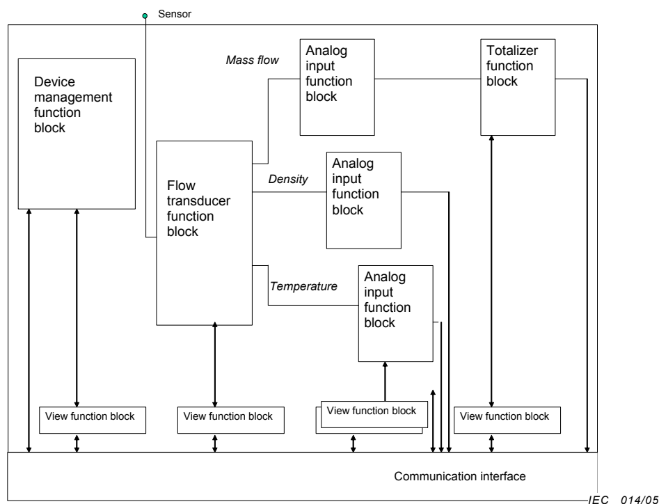
Figure 13 – Device functional structure of a flow transmitter based on the function block model (example)
