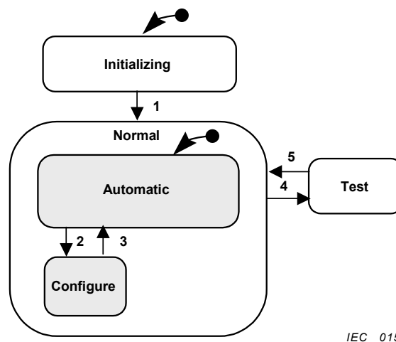
Figure 14 – Device behaviour as state chart diagram (example)
