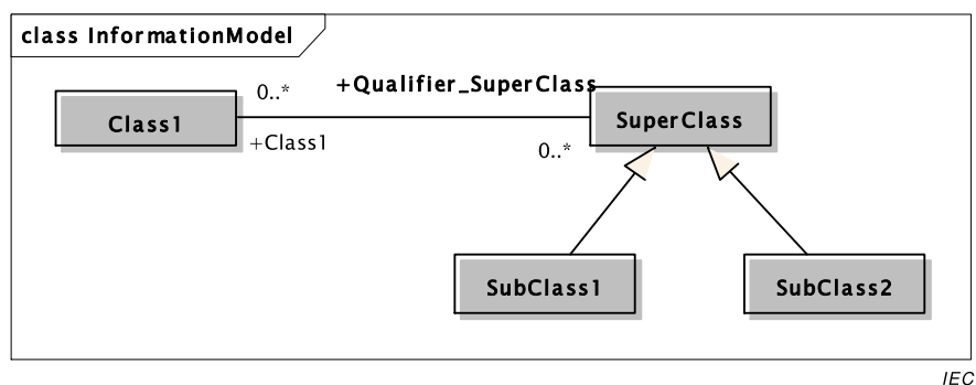
Figure C.9 – Example of end role name with a qualifier
