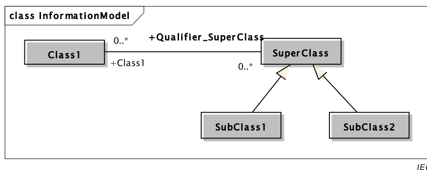
Figure C.3 – Example of end role name with a qualifier
