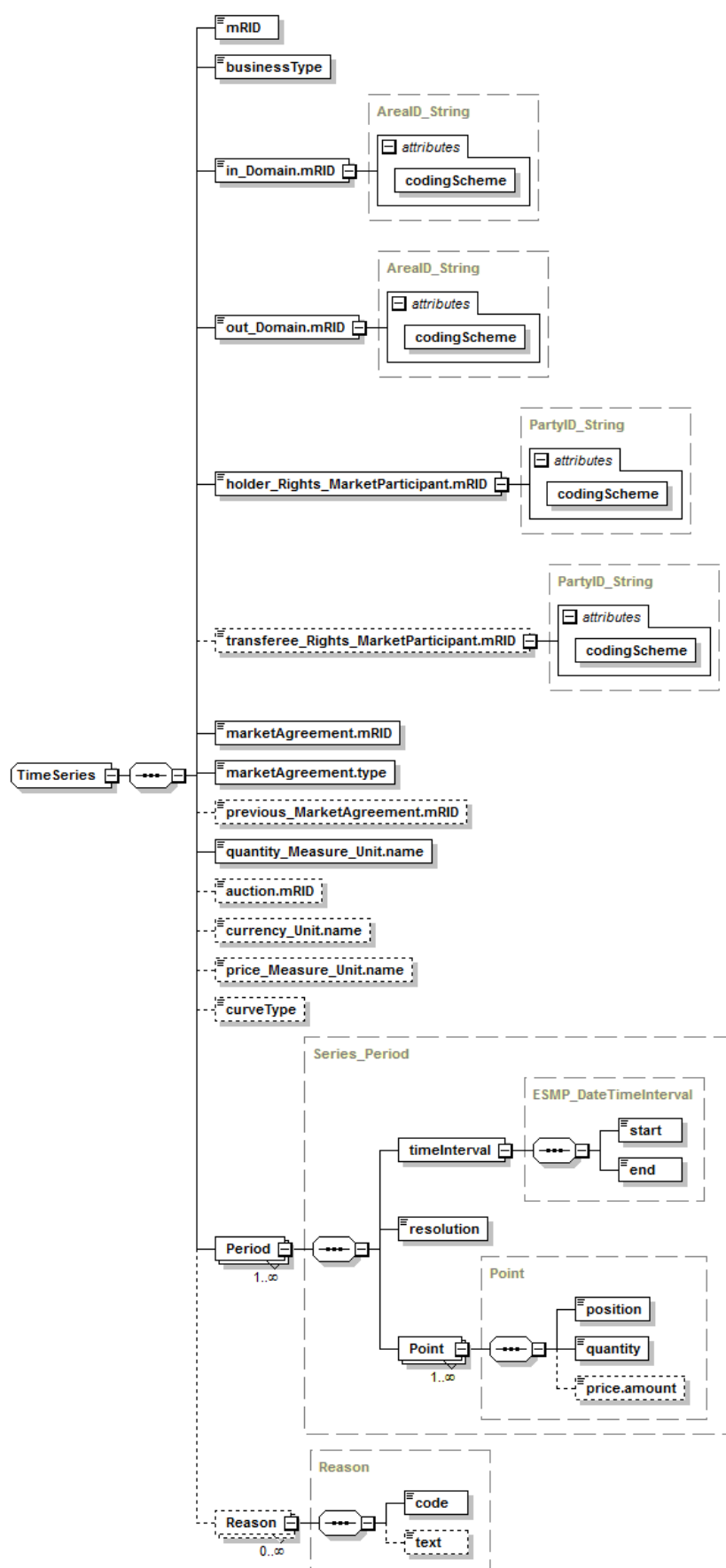
Figure 40 – Structure du schéma XML Rights_MarketDocument – 2/2
