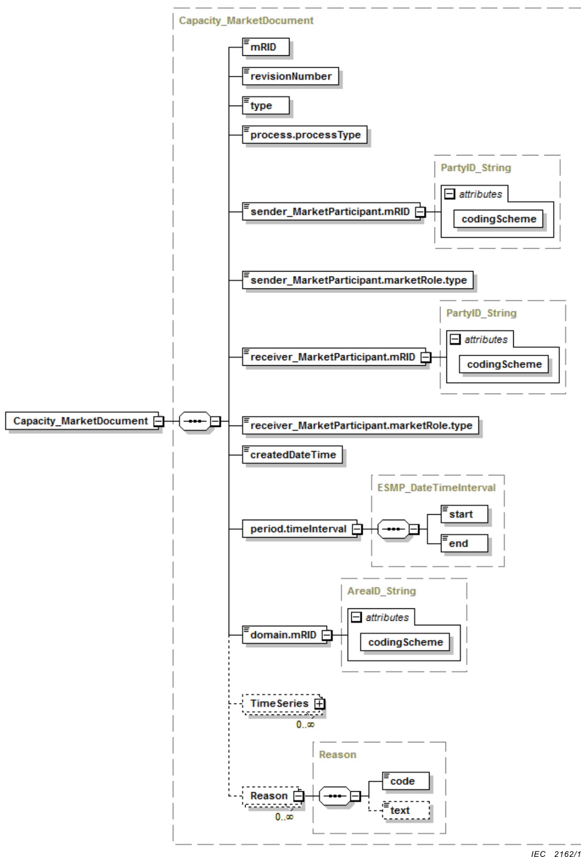
Figure 29 – Structure du schéma XML Capacity_MarketDocument – 1/2
