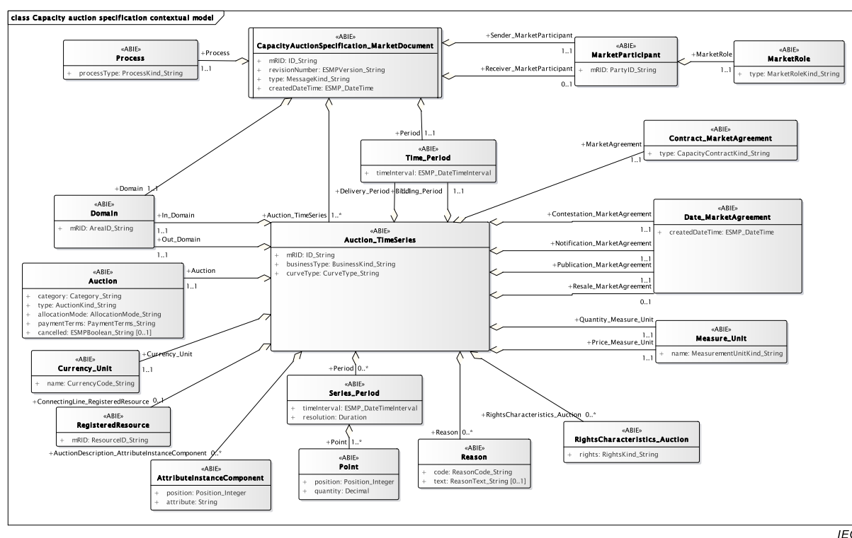
Figure 11 – Capacity auction specification contextual model
