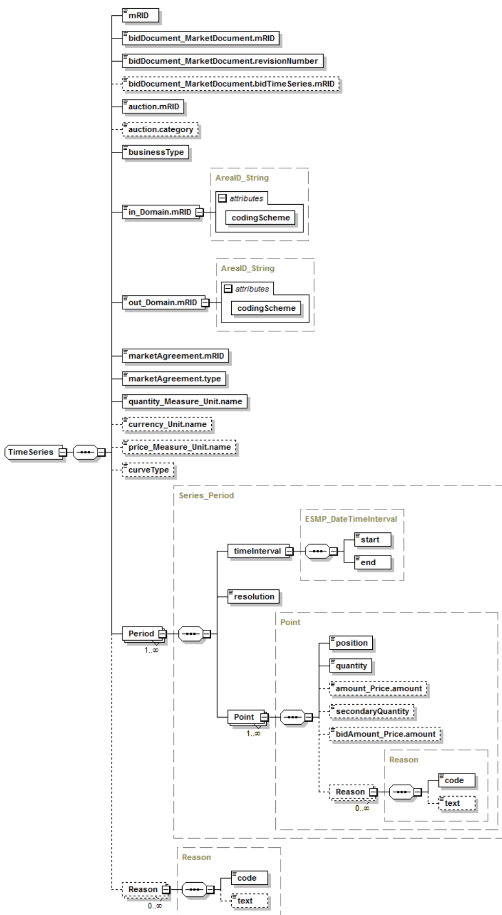
Figure 32 – Structure du schéma XML AllocationResult_MarketDocument – 2/2
