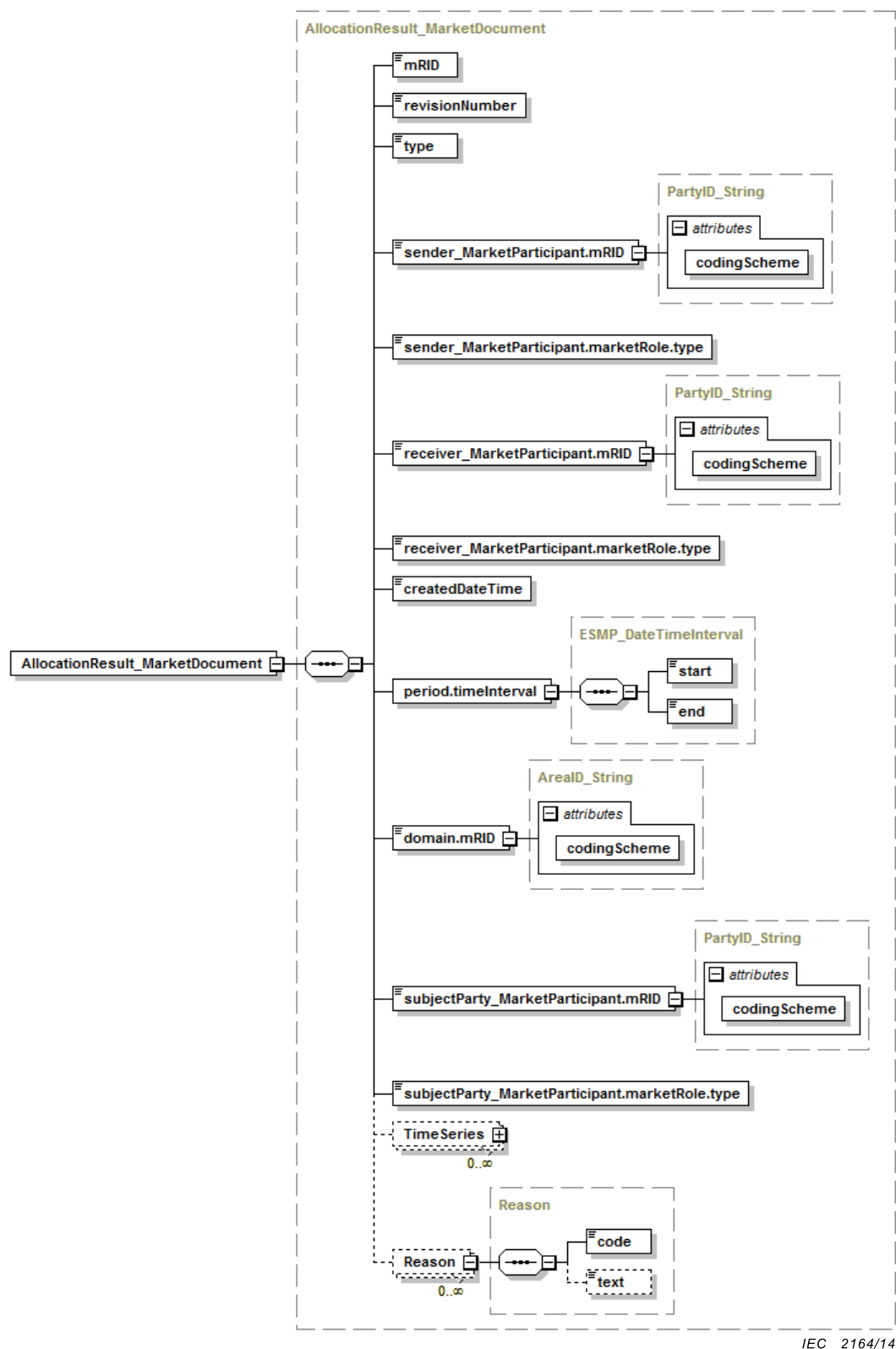
Figure 31 – Structure du schéma XML AllocationResult_MarketDocument – 1/2
