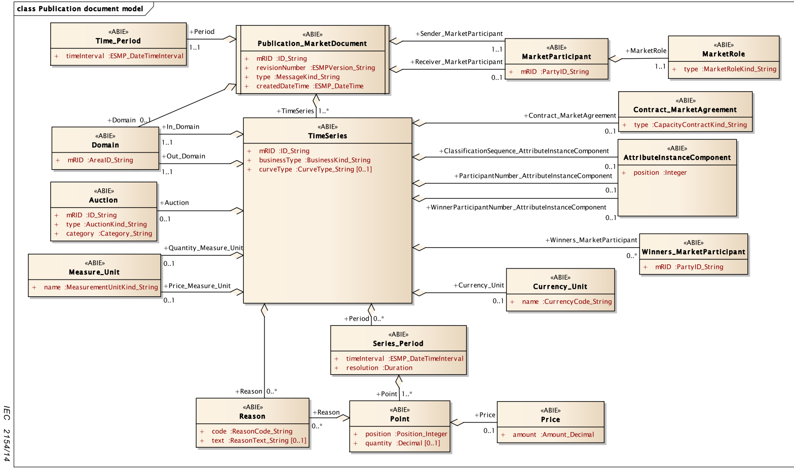
Figure 21 – Publication contextual model
