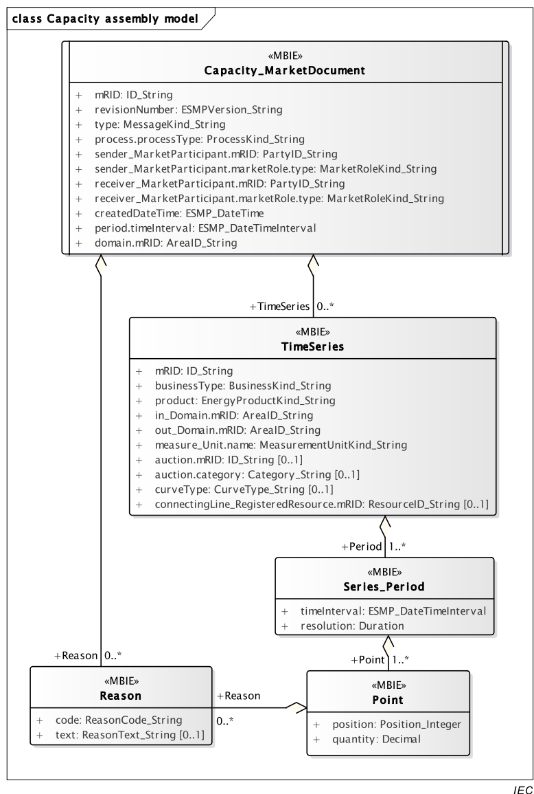
Figure 14 – Capacity assembly model
