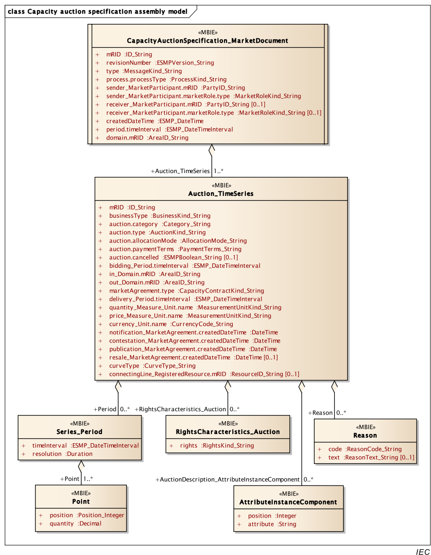
Figure 12 – Capacity auction specification assembly model
