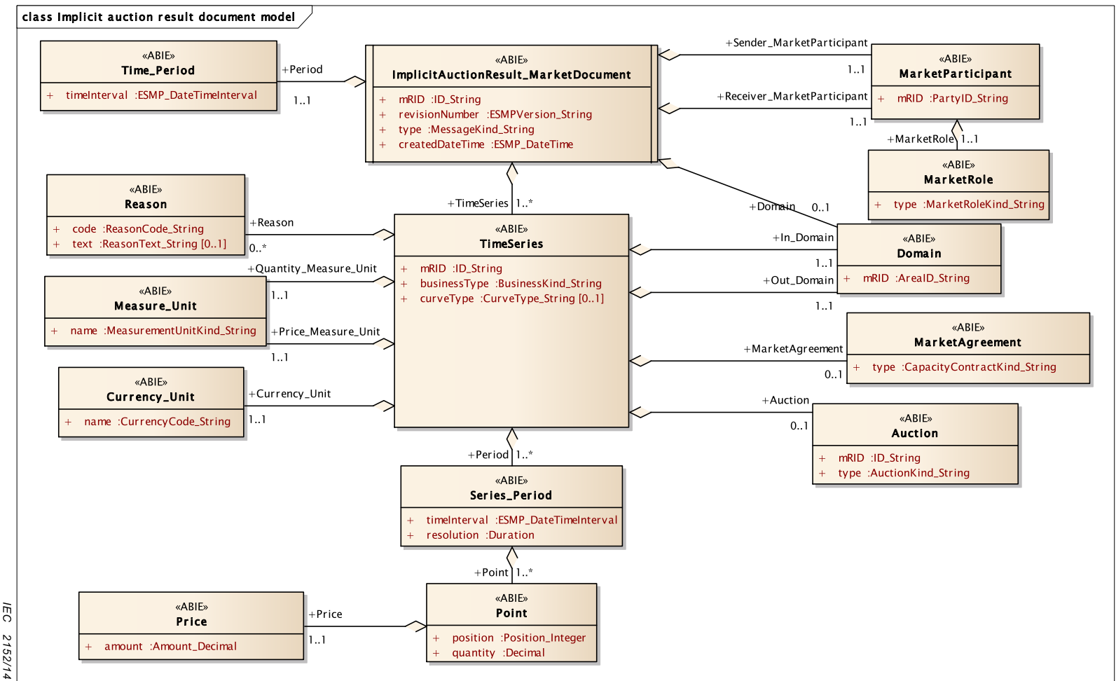
Figure 19 – Implicit auction result contextual model
