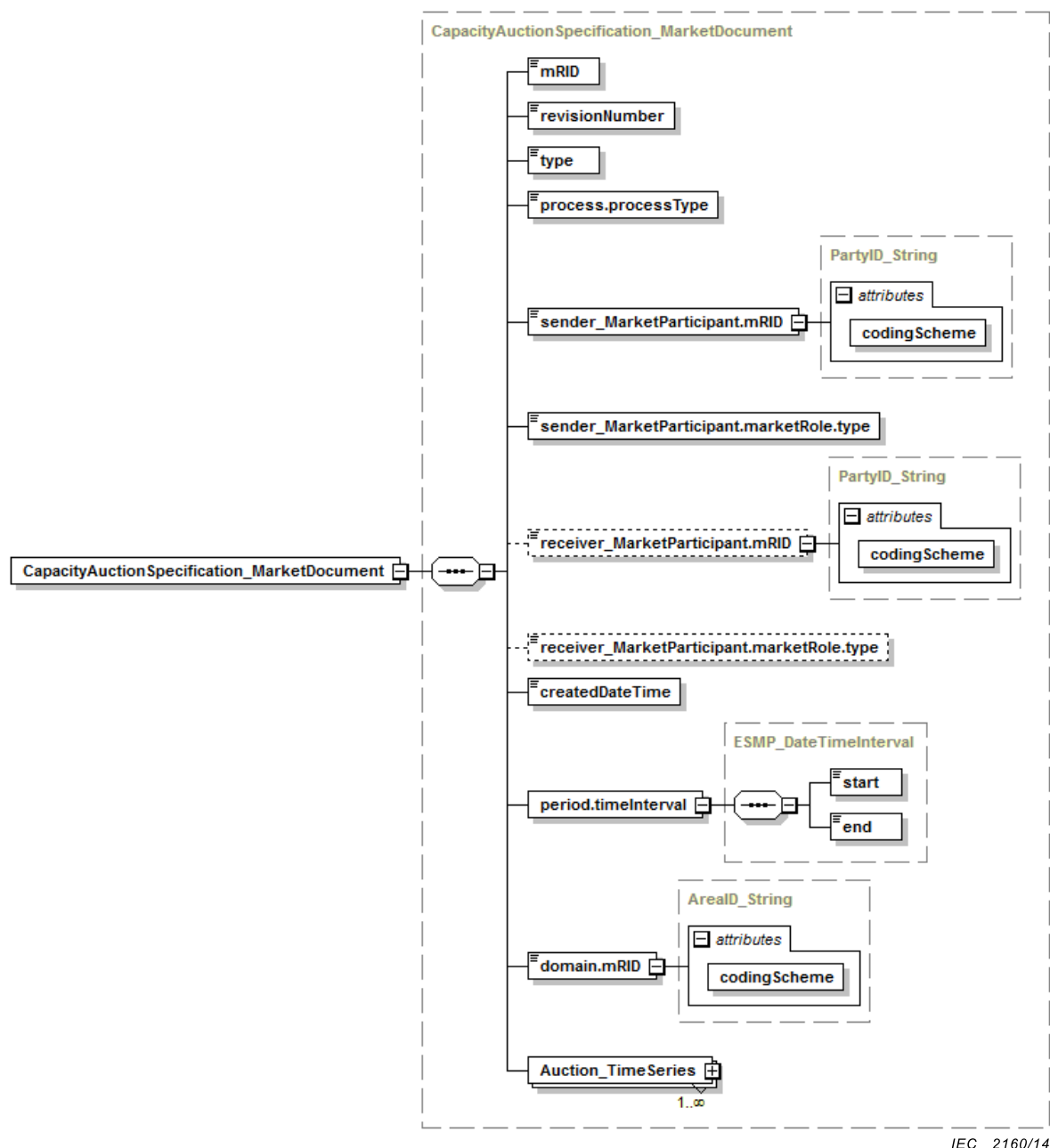
Figure 27 – Structure du schéma XML CapacityAuctionSpecification_MarketDocument – 1/2
