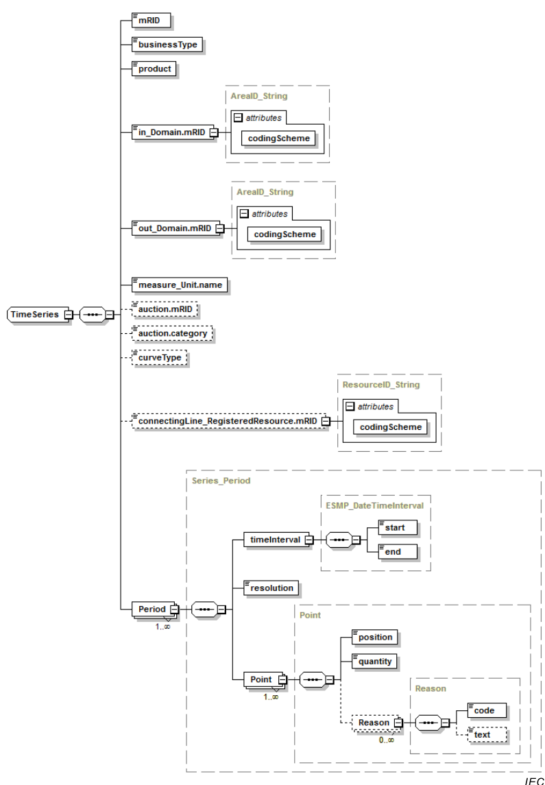
Figure 30 – Structure du schéma XML Capacity_MarketDocument – 2/2
