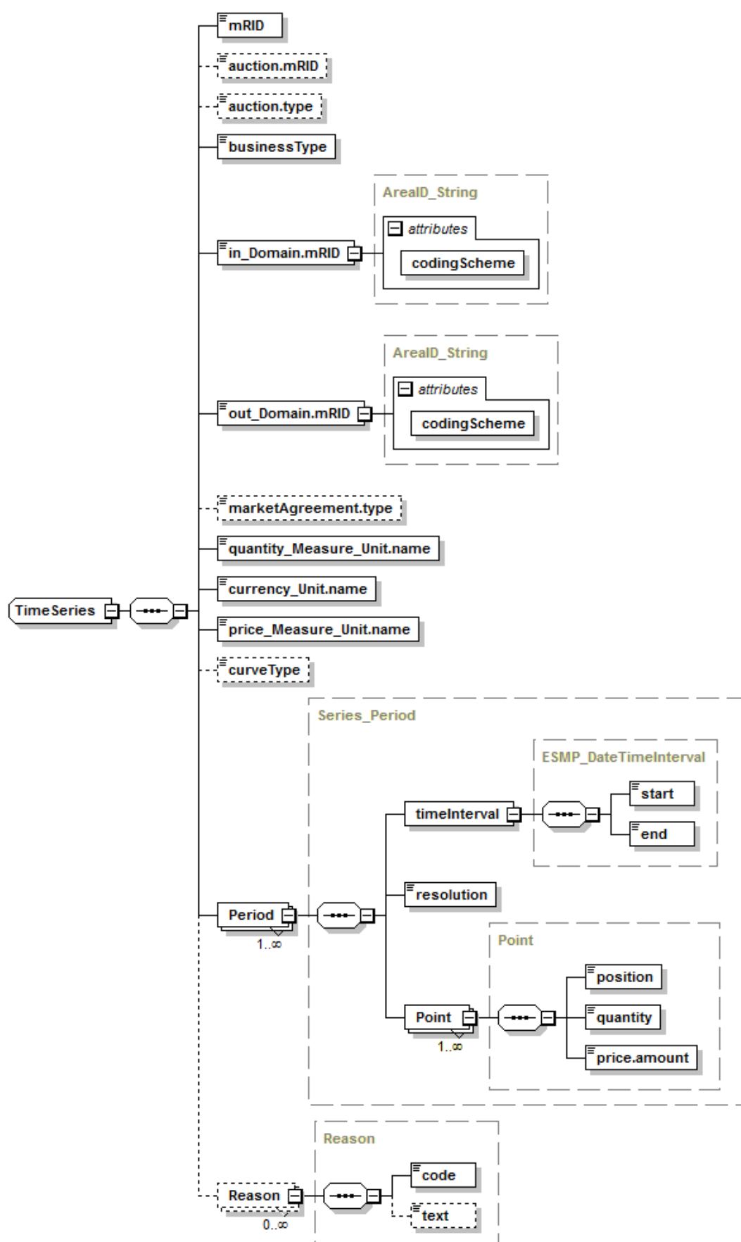
Figure 36 – Structure du schéma XML ImplicitAuctionResult_MarketDocument – 2/2
