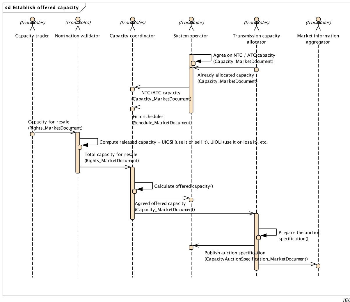
Figure 4 – Establish offered capacity overview
