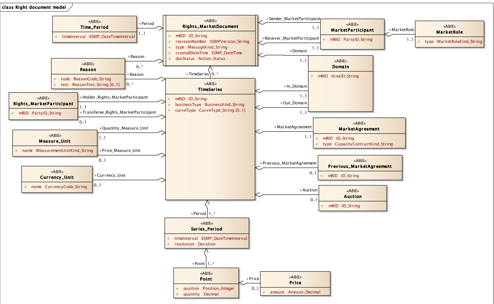
Figure 23 – Rights contextual model
