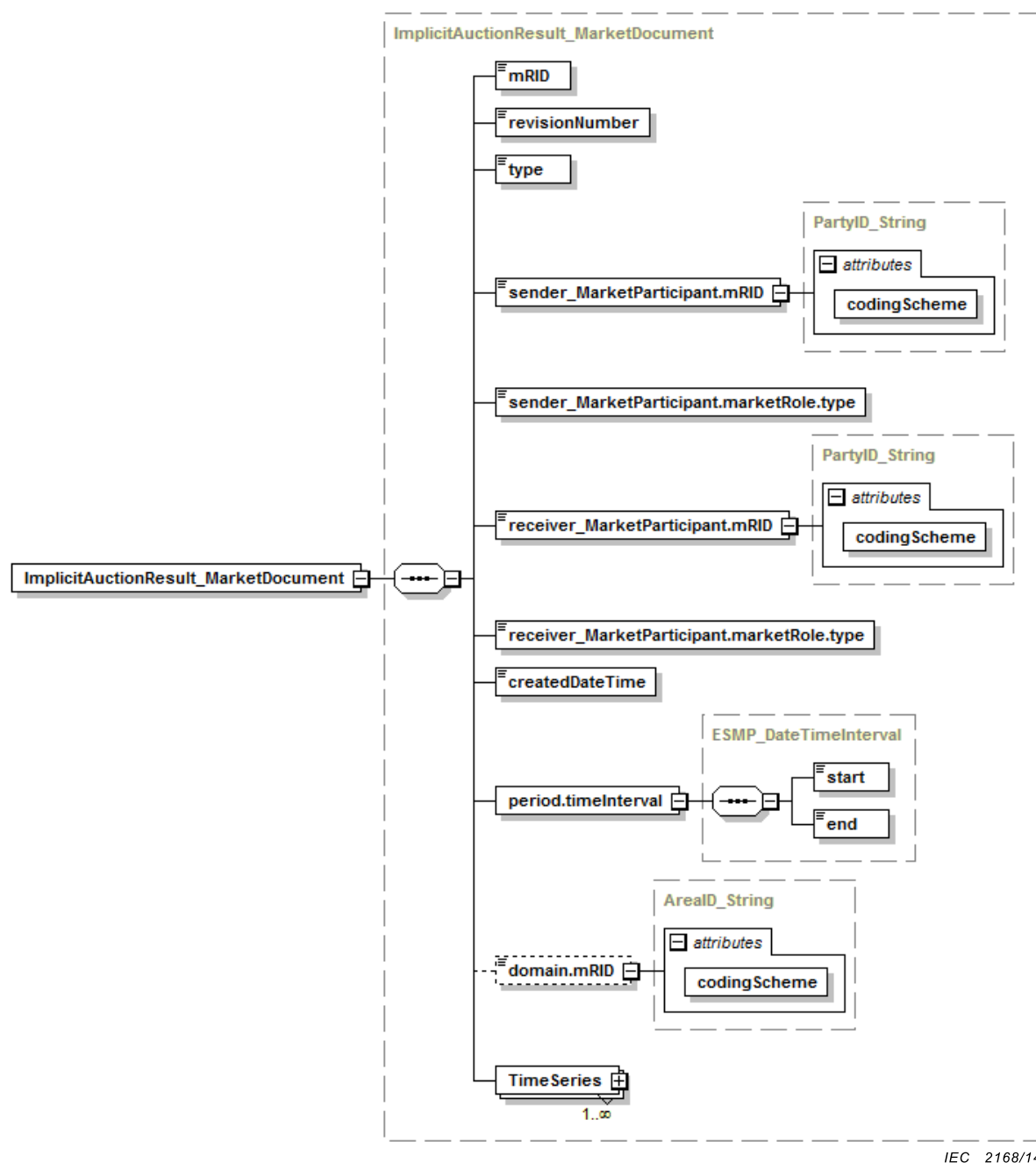
Figure 35 – ImplicitAuctionResult_MarketDocument XML schema structure – 1/2
