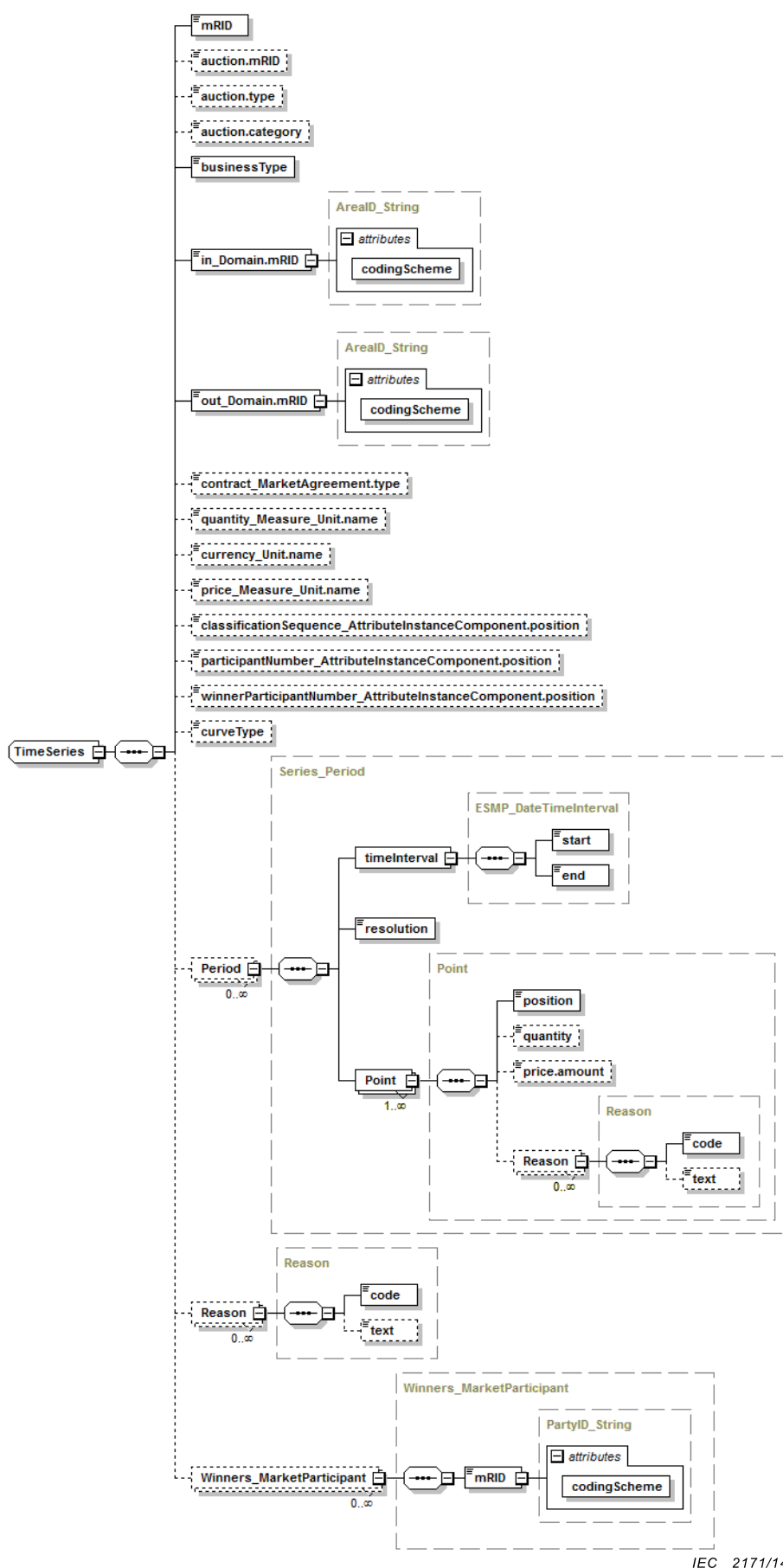
Figure 38 – Structure du schéma XML Publication_MarketDocument – 2/2
