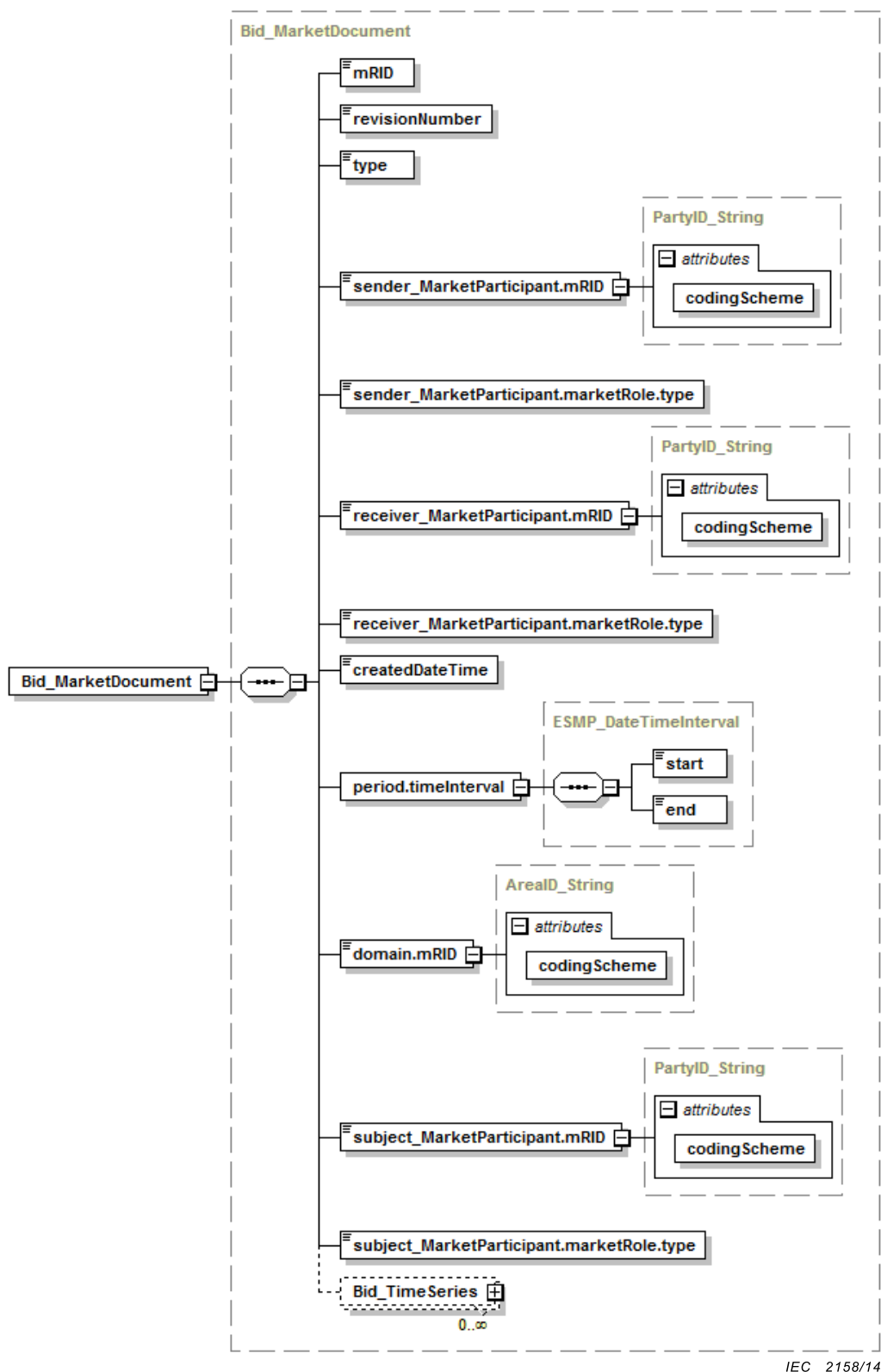
Figure 25 – Bid_MarketDocument XML schema structure – 1/2
