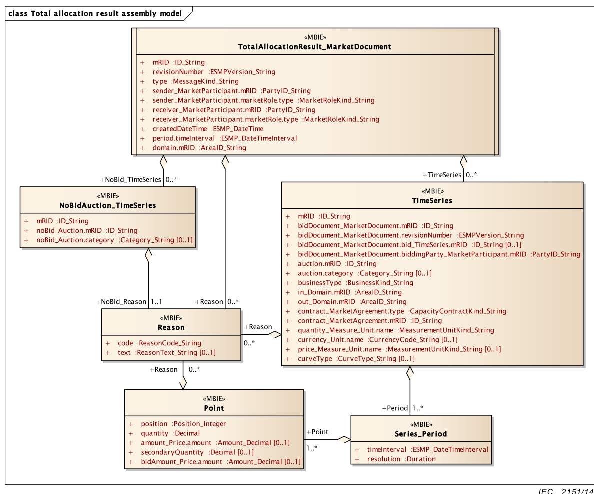
Figure 18 – Total allocation result assembly model
