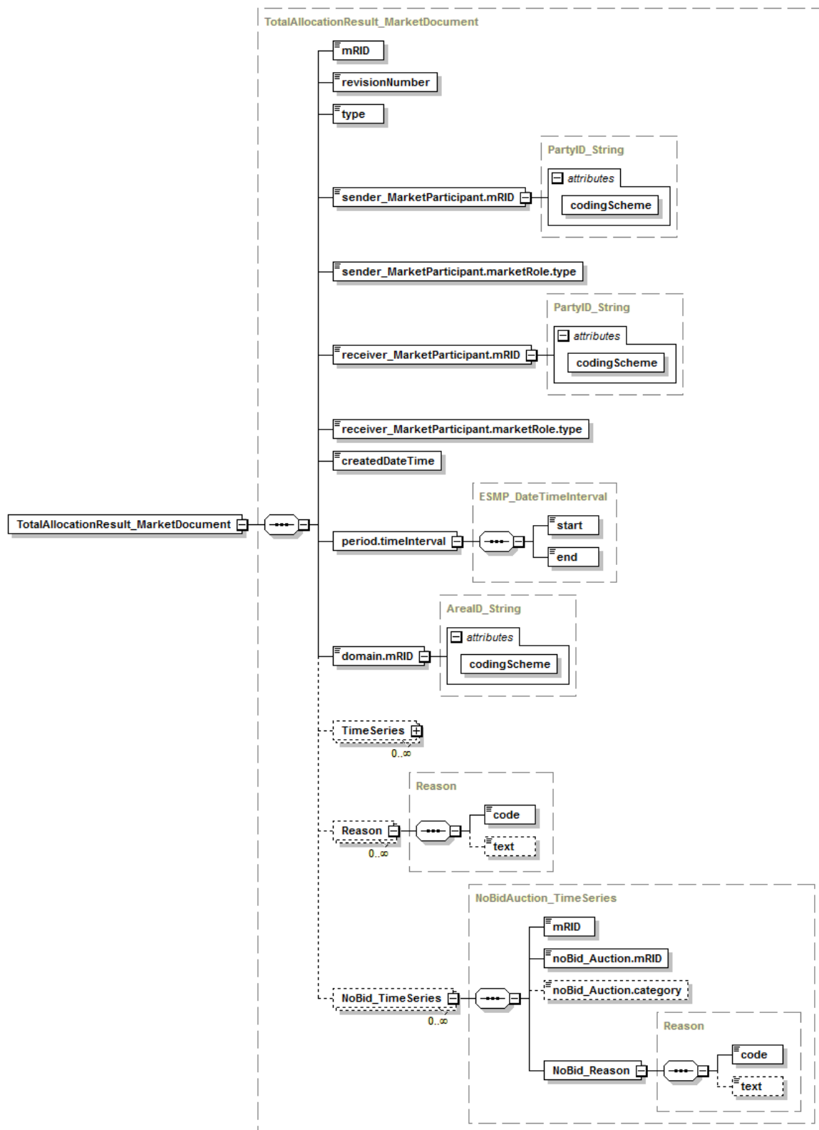
Figure 33 – TotalAllocationResult_MarketDocument XML schema structure – 1/2
