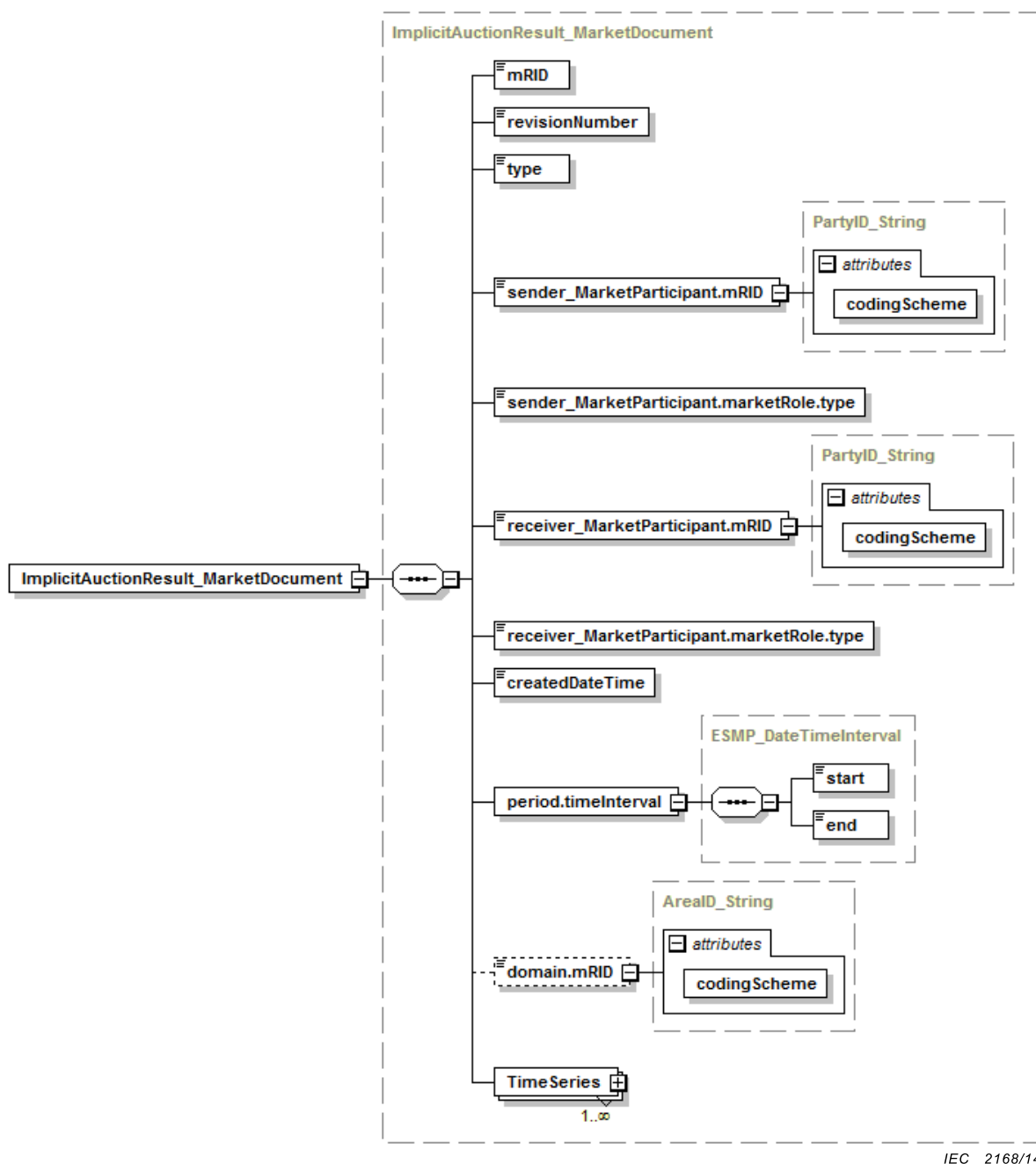
Figure 35 – Structure du schéma XML ImplicitAuctionResult_MarketDocument – 1/2
