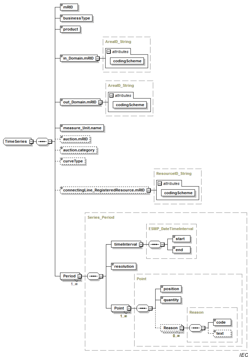
Figure 30 – Capacity_MarketDocument XML schema structure – 2/2
