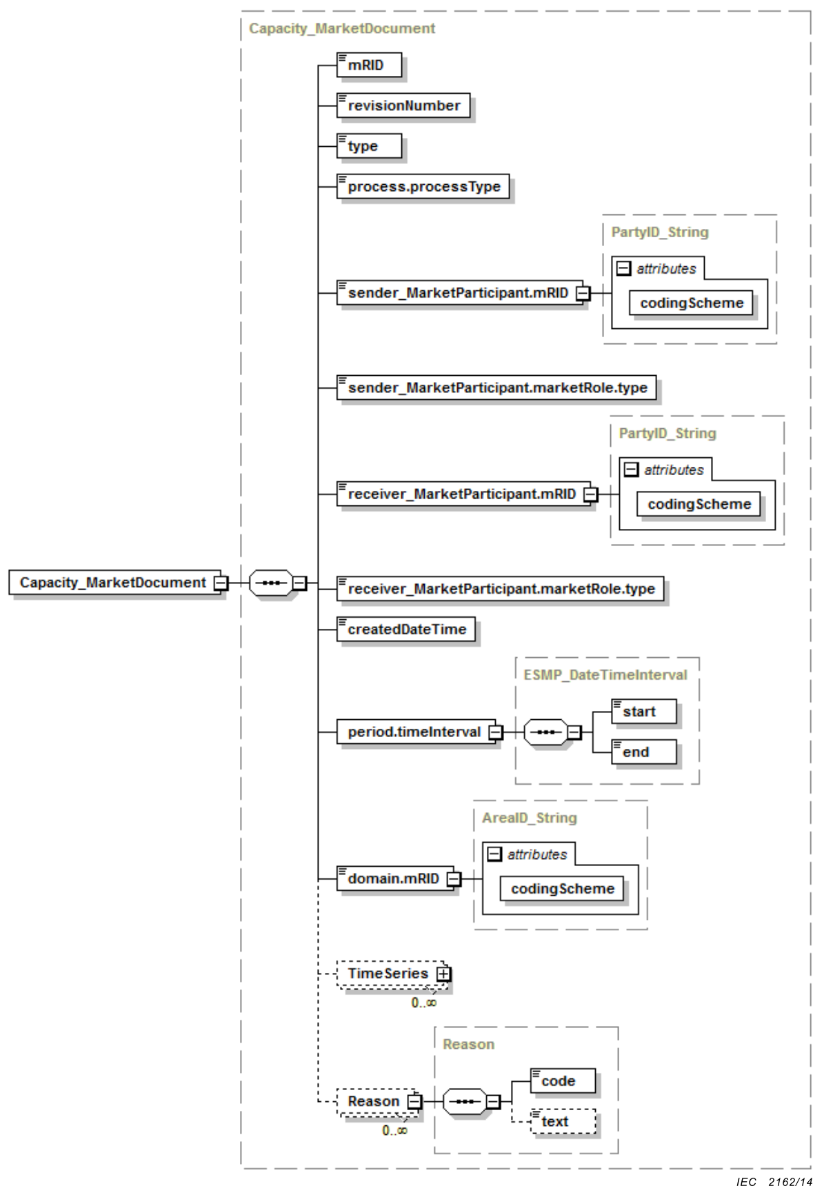
Figure 29 – Structure du schéma XML Capacity_MarketDocument – 1/2
