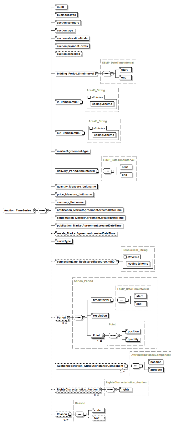
Figure 28 – CapacityAuctionSpecification_MarketDocument XML schema structure – 2/2
