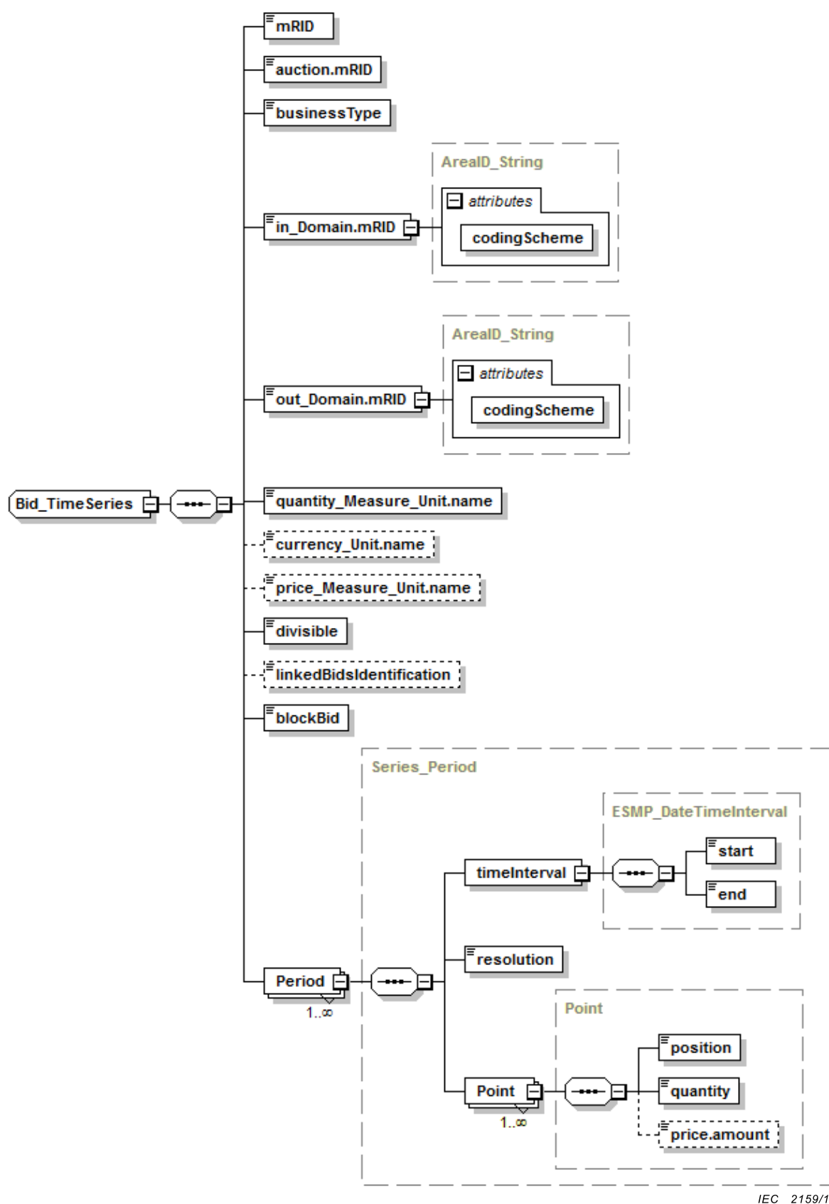
Figure 26 – Structure du schéma XML Bid_MarketDocument – 2/2
