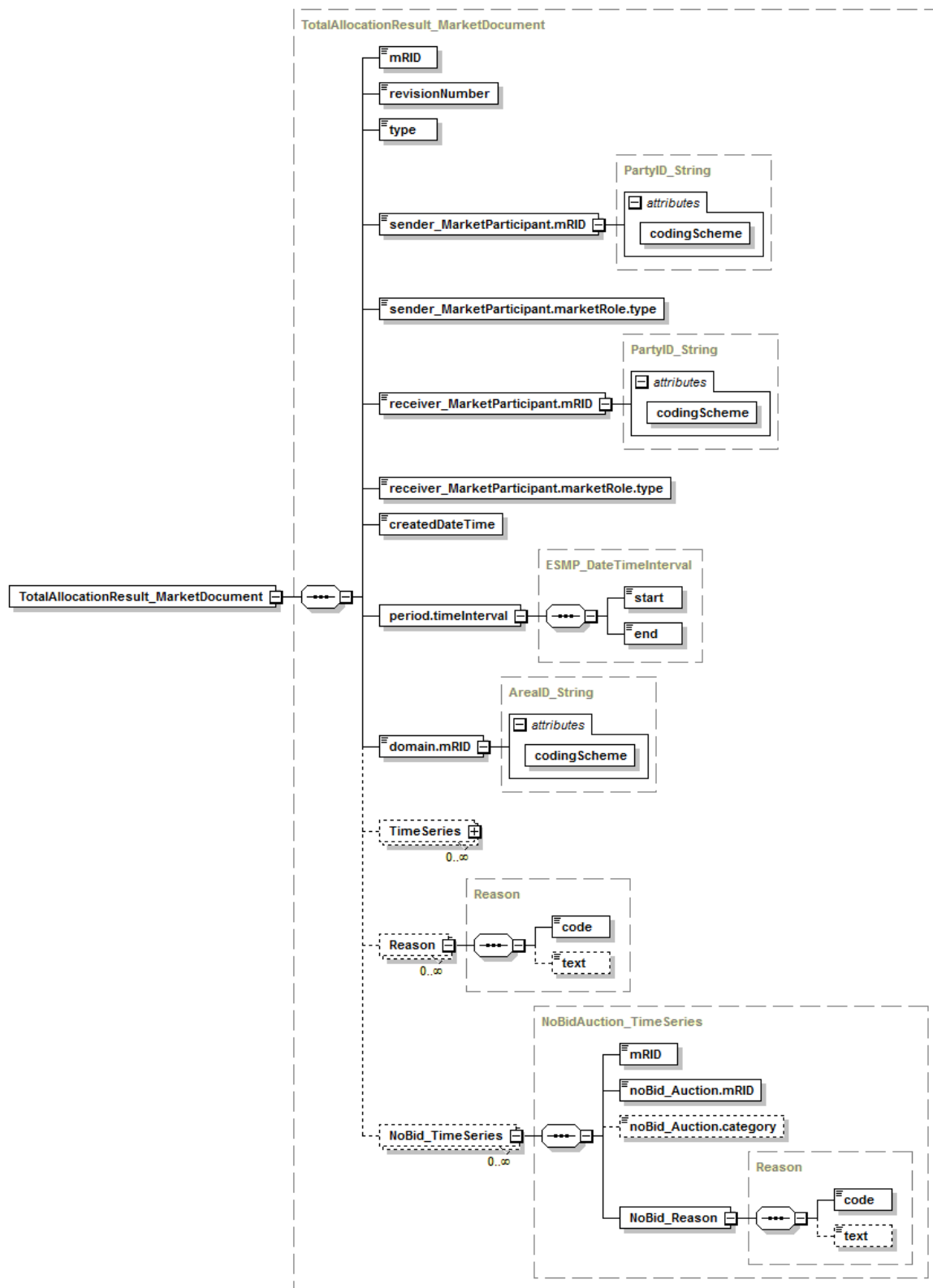
Figure 33 – Structure du schéma XML TotalAllocationResult_MarketDocument – 1/2
