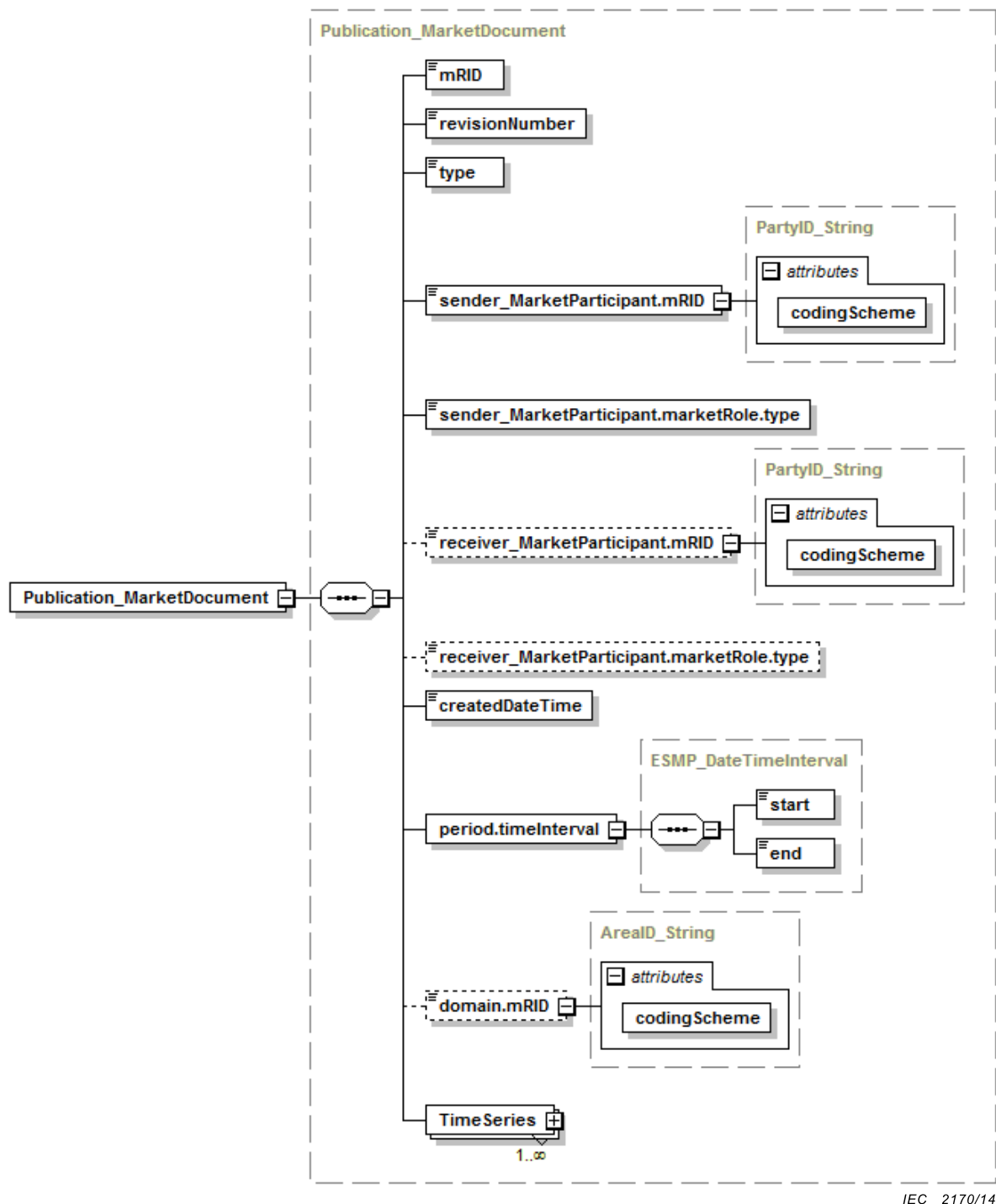
Figure 37 – Structure du schéma XML Publication_MarketDocument – 1/2
