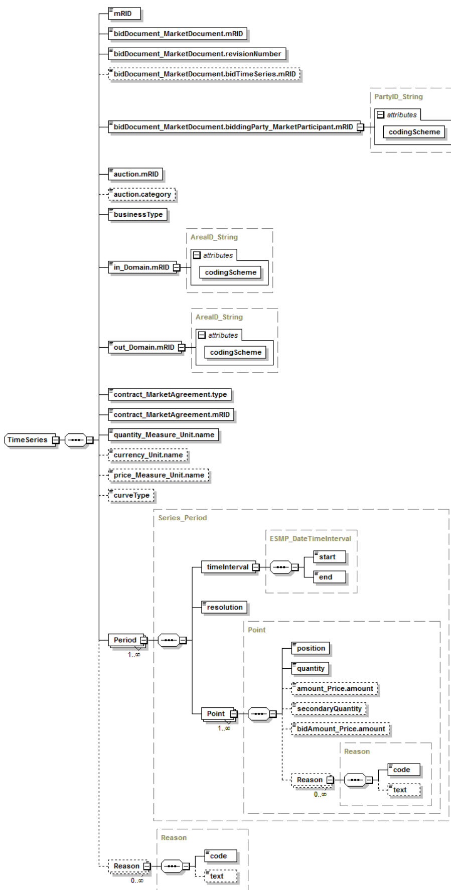
Figure 34 – Structure du schéma XML TotalAllocationResult_MarketDocument – 2/2
