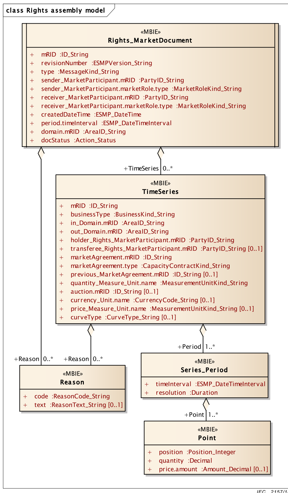
Figure 24 – Rights assembly model
