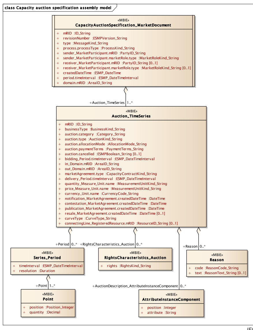
Figure 12 – Capacity auction specification assembly model
