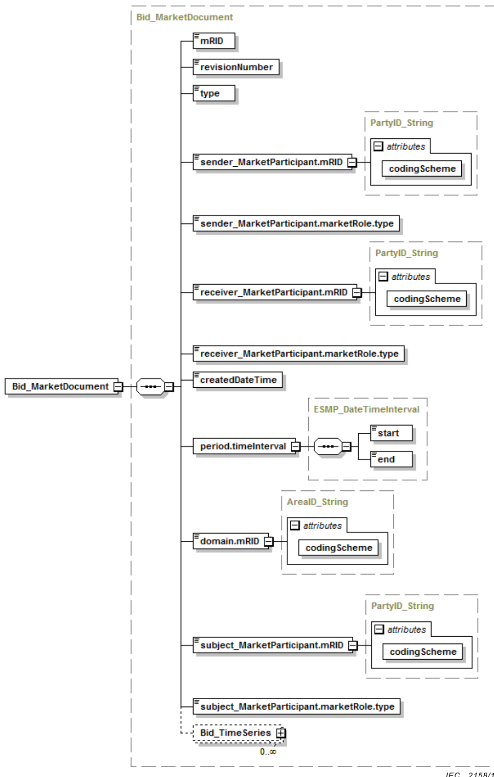
Figure 25 – Structure du schéma XML Bid_MarketDocument – 1/2
