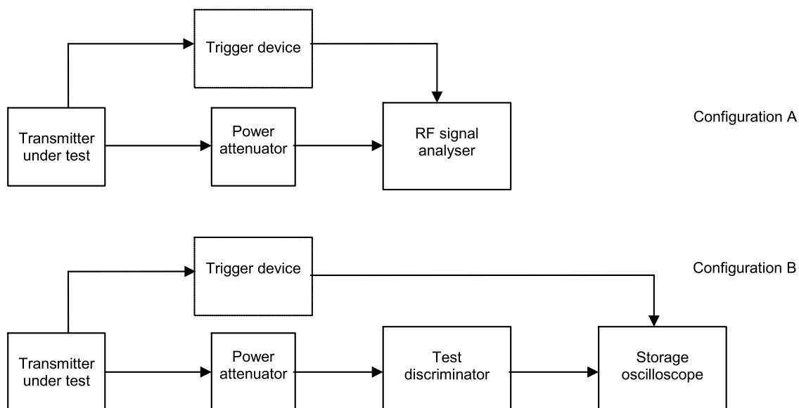
Figure 7 – Measurement arrangement
