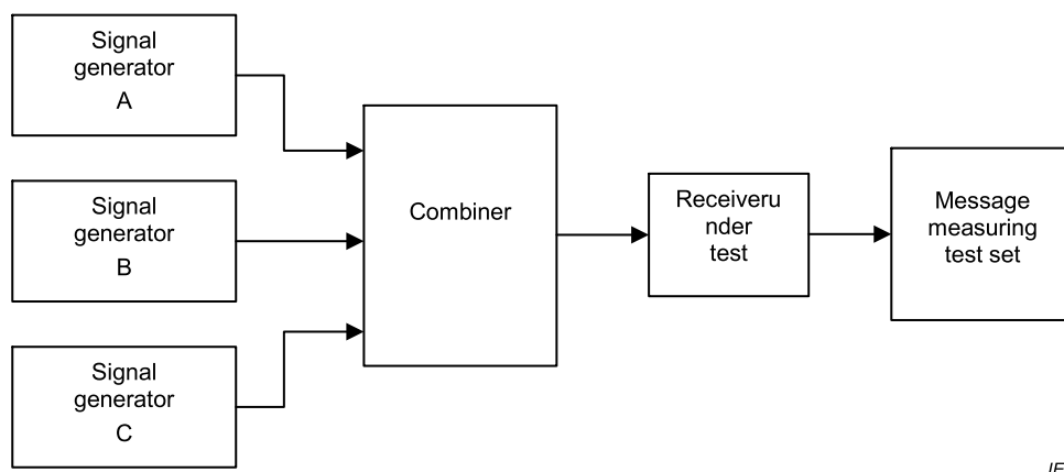
Figure 15 – Measurement arrangement
