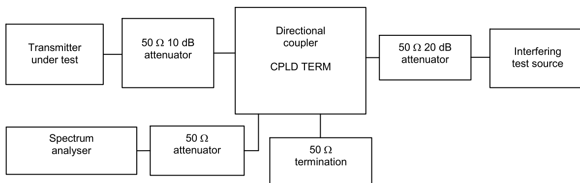
Figure 9 – Measurement arrangement
