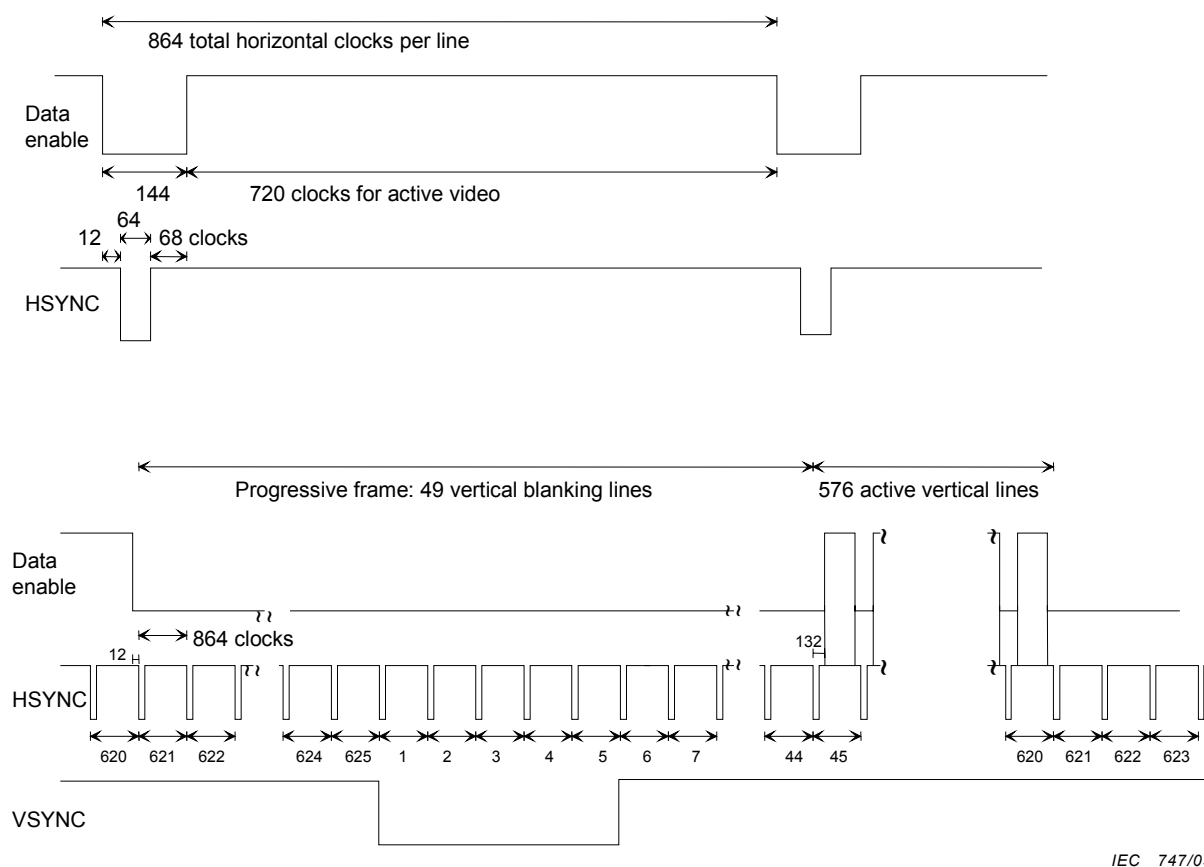
Figure 9 – Timing parameters for 720x576p, 50 Hz
