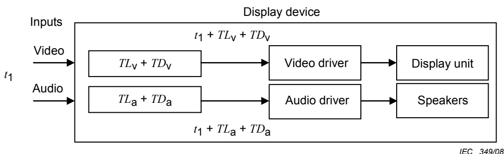
Figure 4 – Display device
