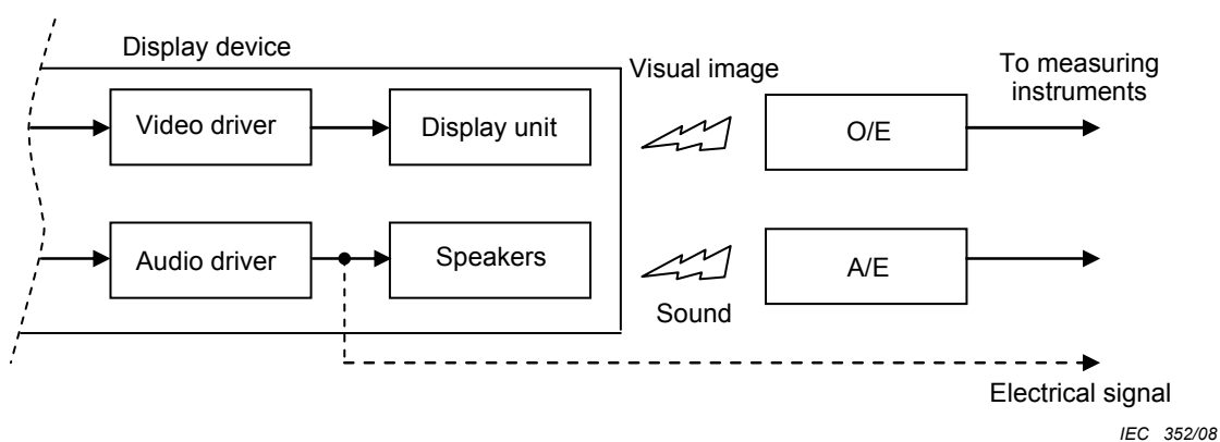
Figure 7 – Measurement of reproduced signal
