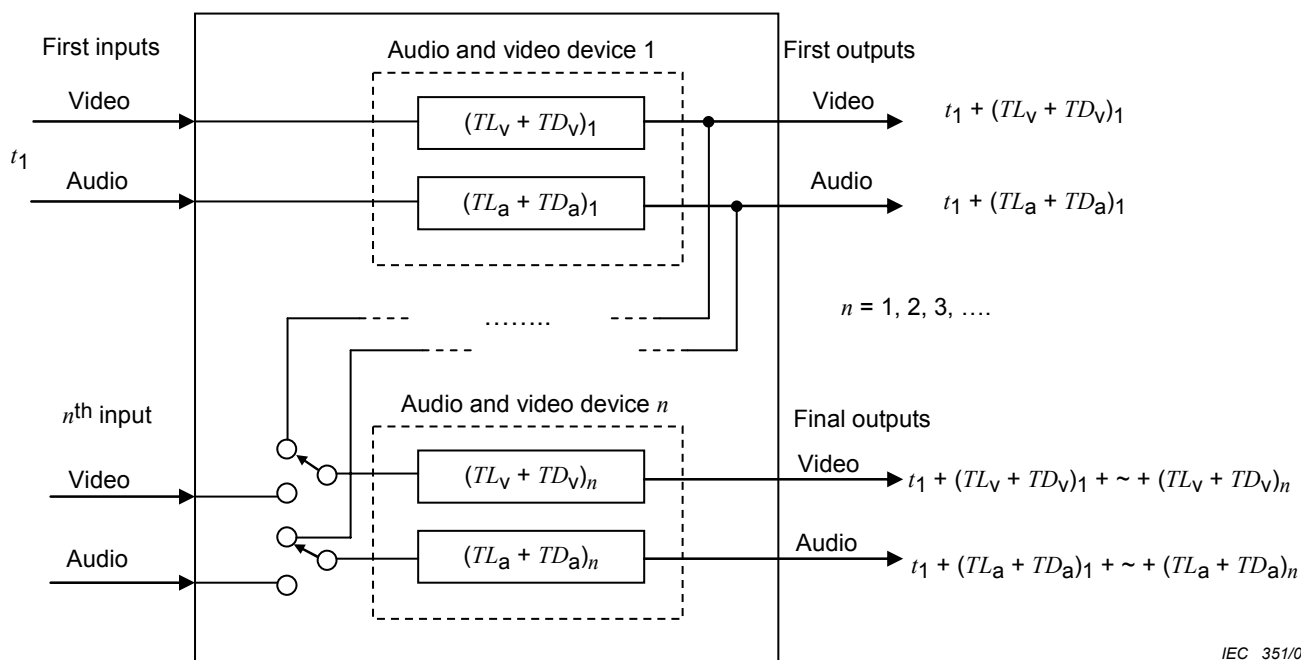
Figure 6 – Compound equipment
