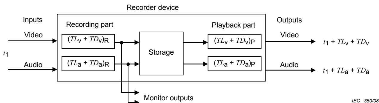
Figure 5 – Recorder device
