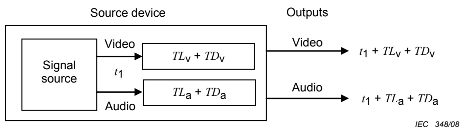
Figure 3 – Source device
