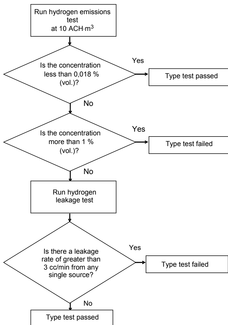
Figure C.7.1 – Flow chart for hydrogen tests
