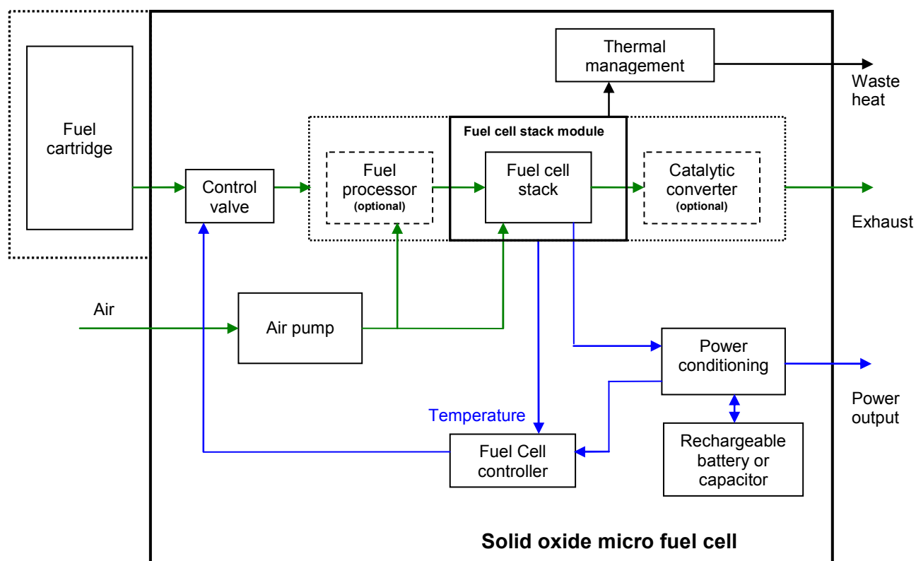
Figure F.1 – Butane powered SOFC block diagram
