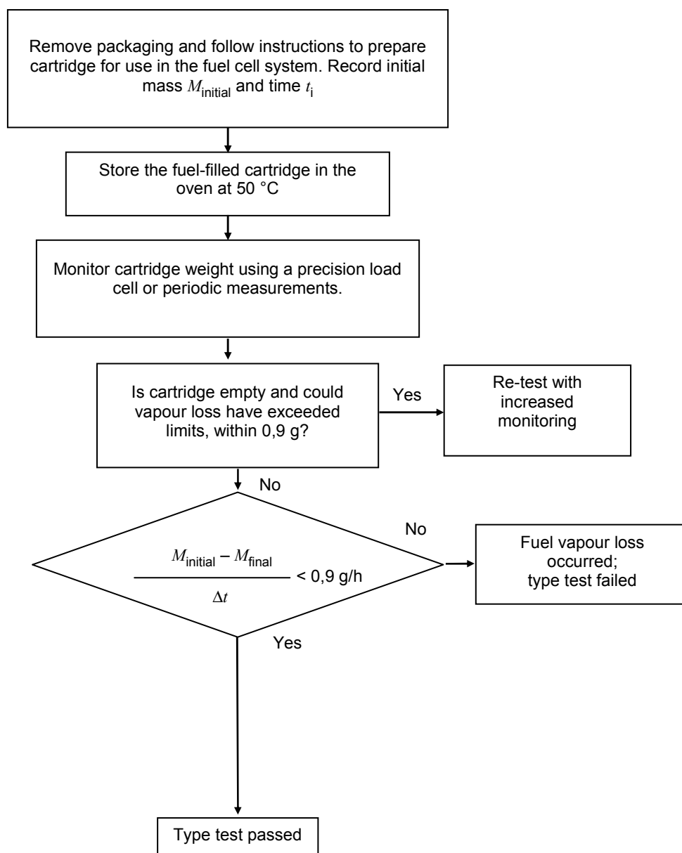
Figure F.6 – Fuel cartridge leakage and mass loss flow chart for long-term storage
