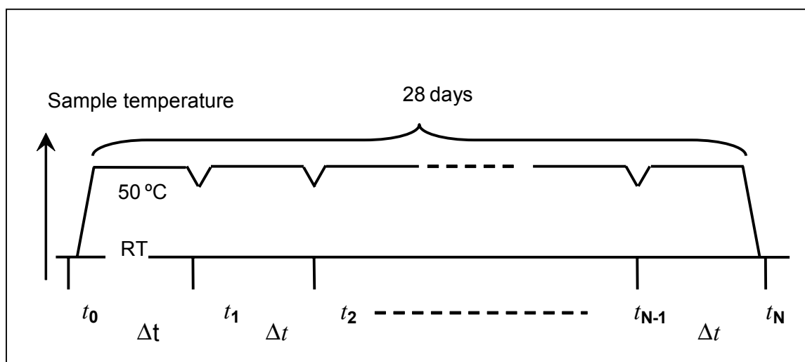
Figure E.4 – Leakage measurement schedule
