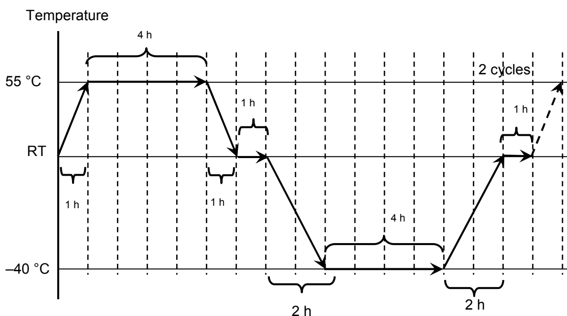
Figure 6 – Temperature cycling
