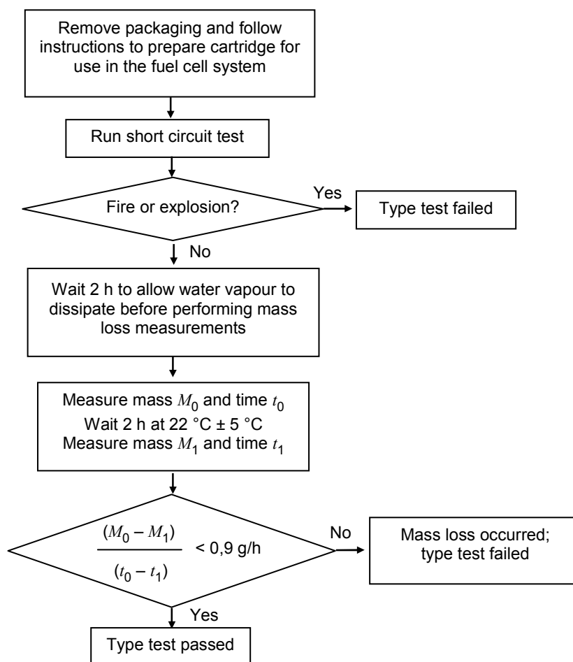
Figure F.5 – Micro fuel cell system/unit leakage and mass loss flow chart for short-circuit test
