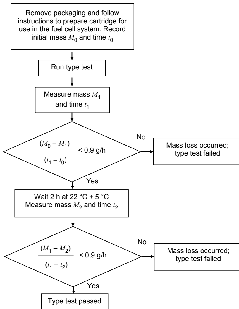
Figure F.2 – Cartridge leakage and mass loss test flow chart for low external pressure, vibration, drop, compressive loading, and internal pressure tests
