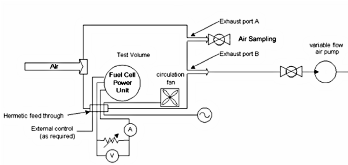
Figure E.5 – Operational emission test apparatus
