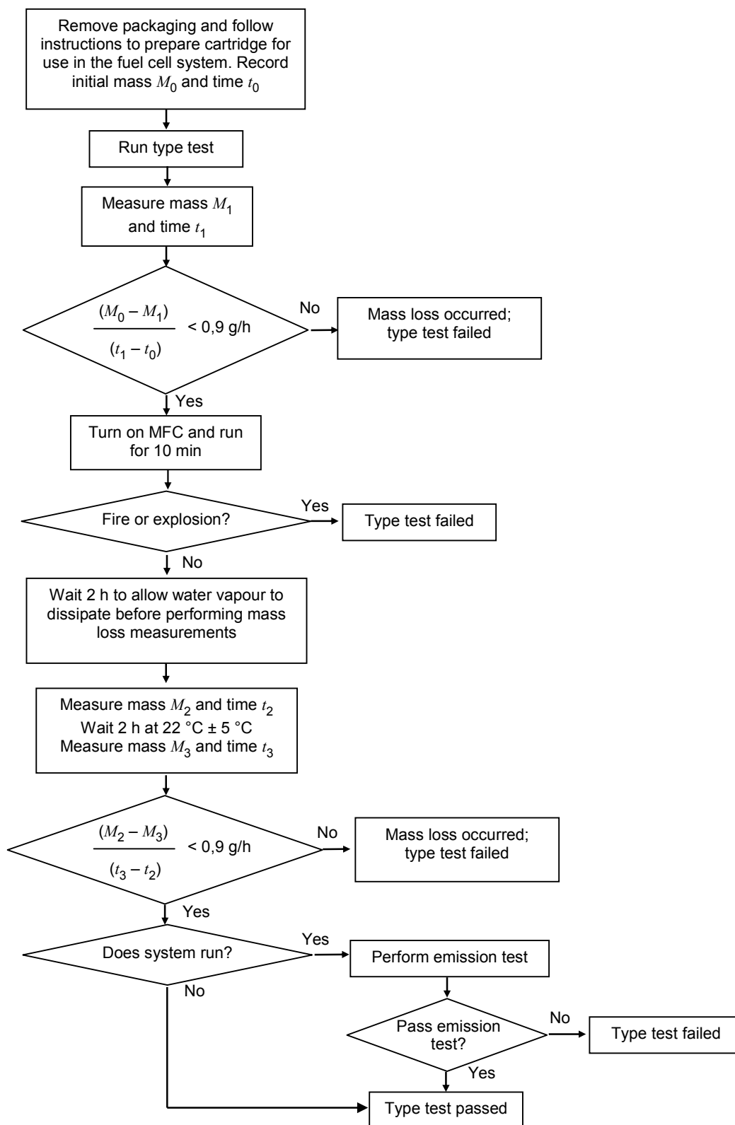
Figure F.4 – Micro fuel cell system / unit leakage and mass loss flow chart for vibration, drop, pressure differential, and compressive loading tests
