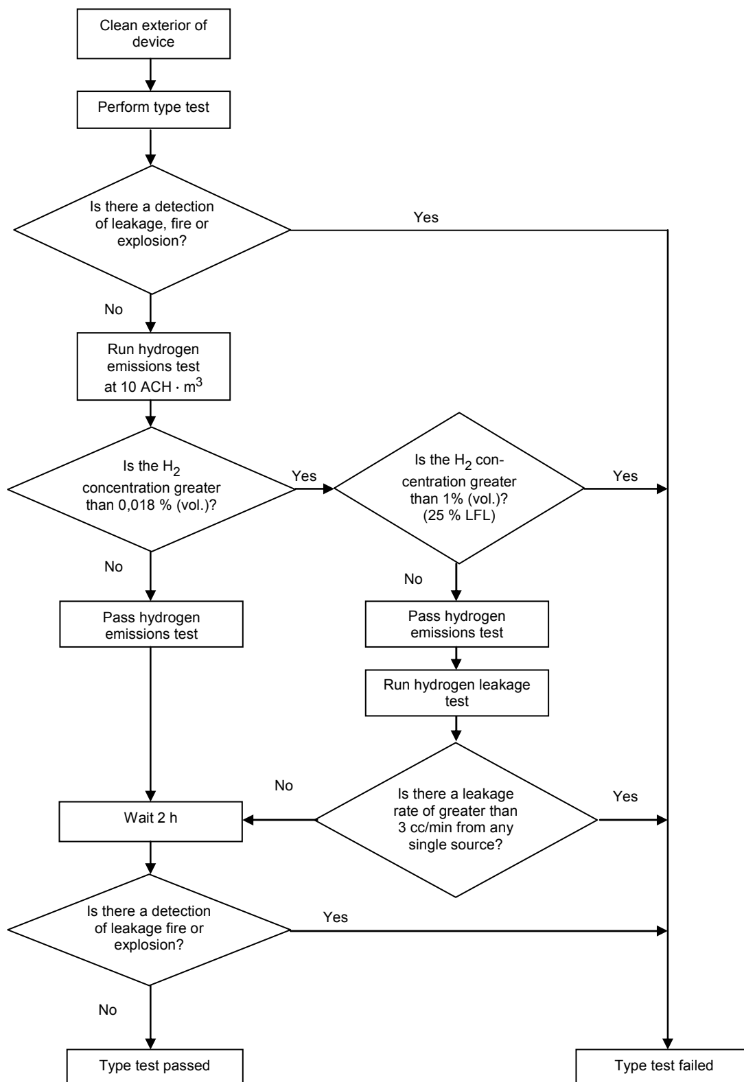
Figure E.3 – Flowchart for leakage measurement and testing procedure
