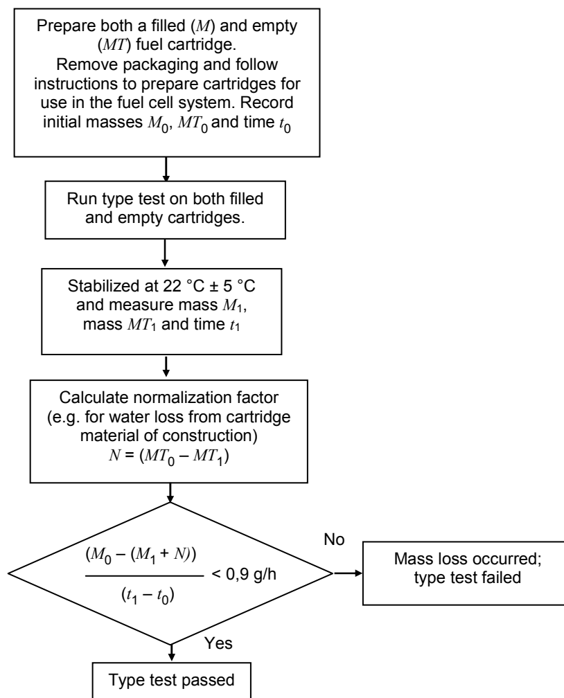
Figure F.3 – Cartridge leakage and mass loss test flow chart for temperature cycling type test and high temperature exposure test
