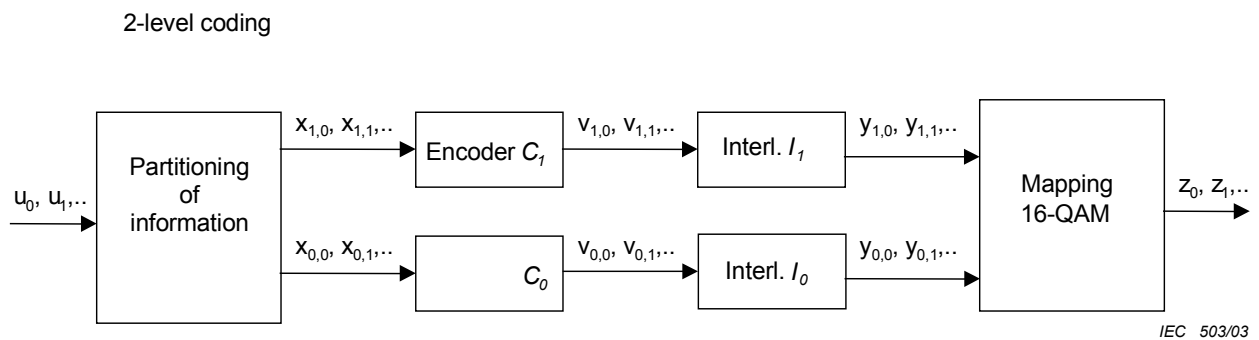
Figure 24 – Multilevel coding with 2 levels (SM)
