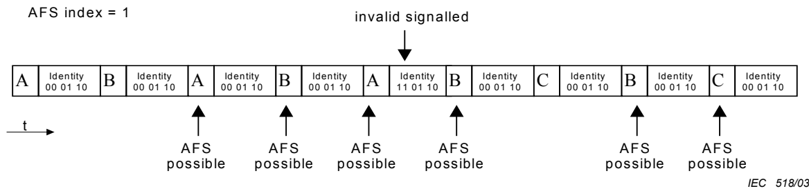
Figure G.4 – Example 3
