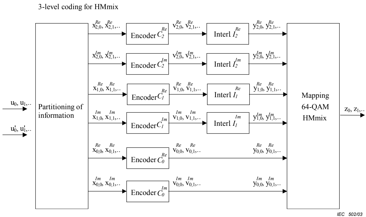
Figure 23 – Multilevel coding with 3 levels for HMix
