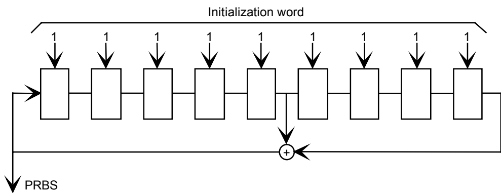
Figure 20 – PRBS generator
