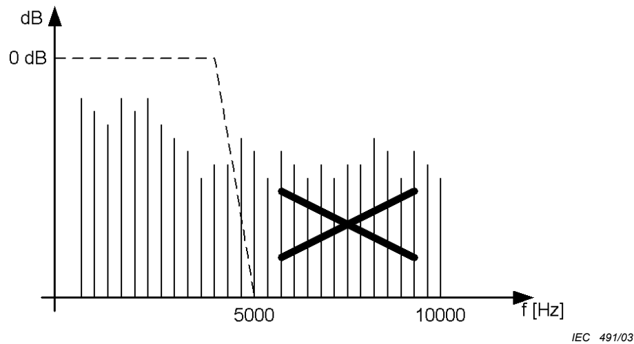
Figure 12 – Example of band-limiting of a typical signal
