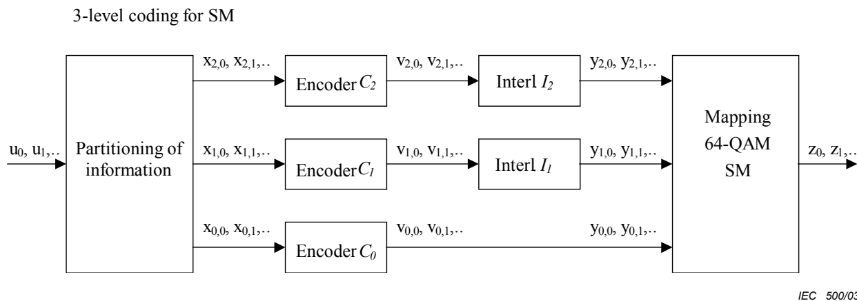
Figure 21 – Multilevel coding with 3 levels for SM
