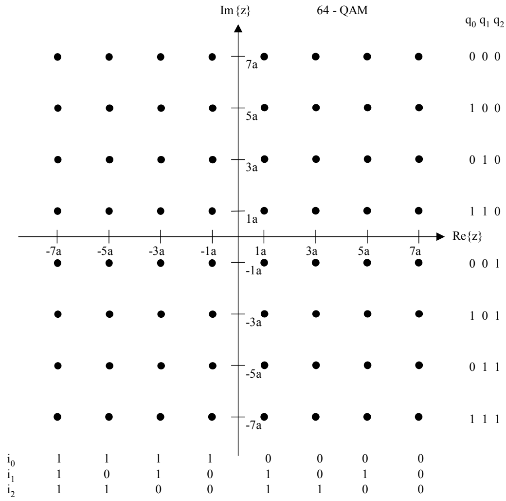
Figure 29 – HMix 64-QAM mapping with corresponding bit pattern
