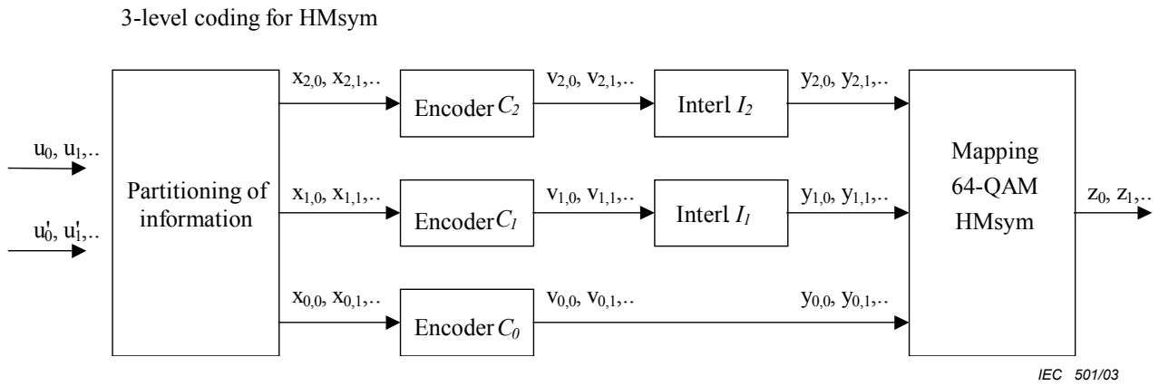
Figure 22 – Multilevel coding with 3 levels for HMsym
