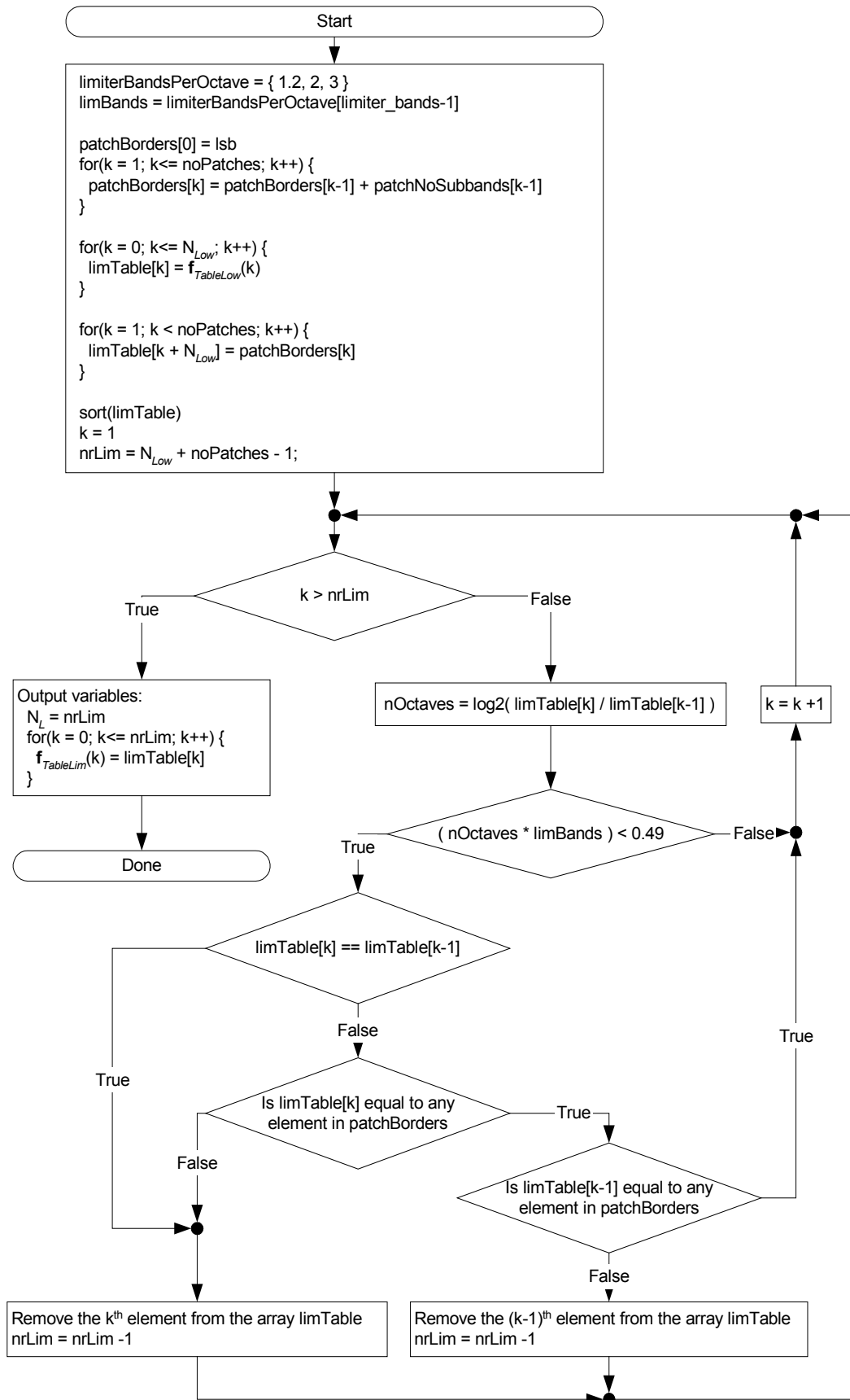
Figure 18 – Calculation of f_{\text{TableLim}} if limiter_bands > 0
