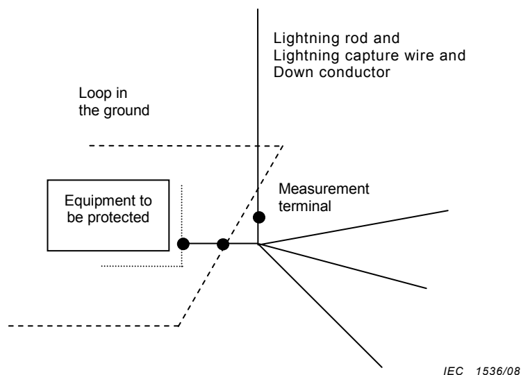
Figure 7 – Example of a simplified lightning protection including a crow's foot earth termination
