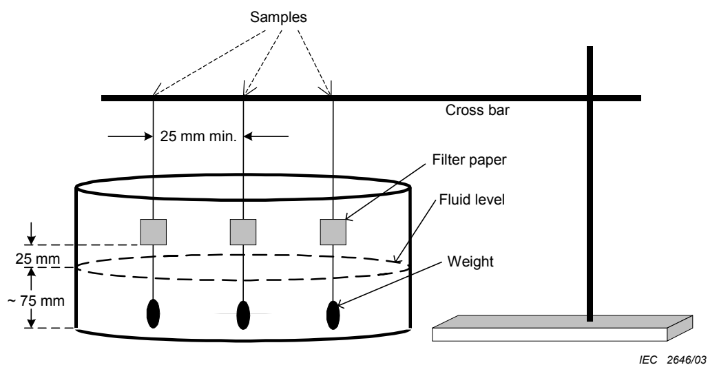
Figure 1 – Wicking test configuration
